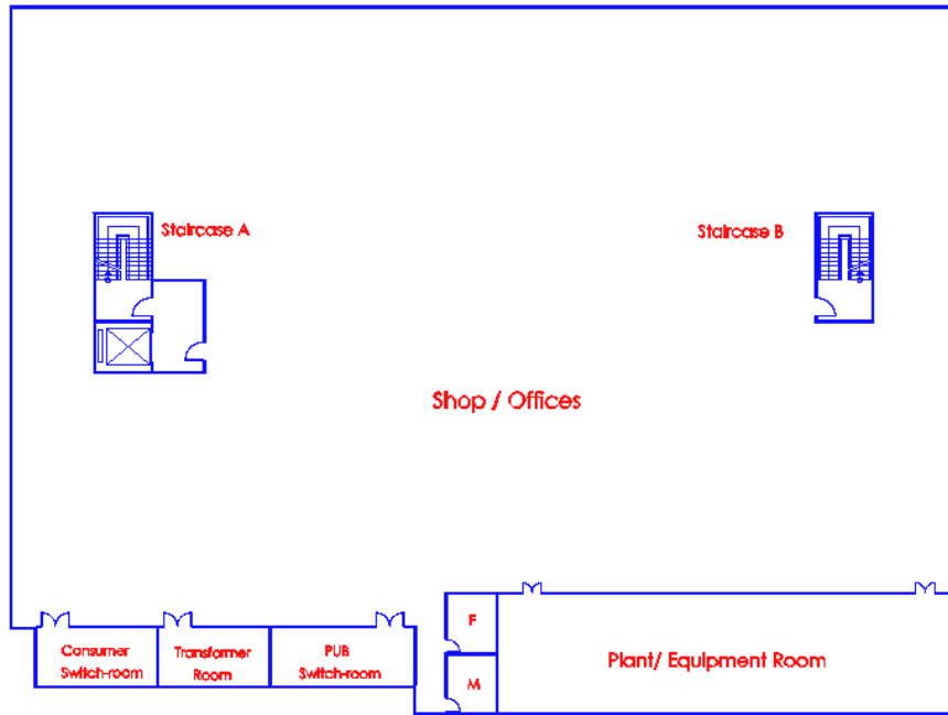
Basement 1
