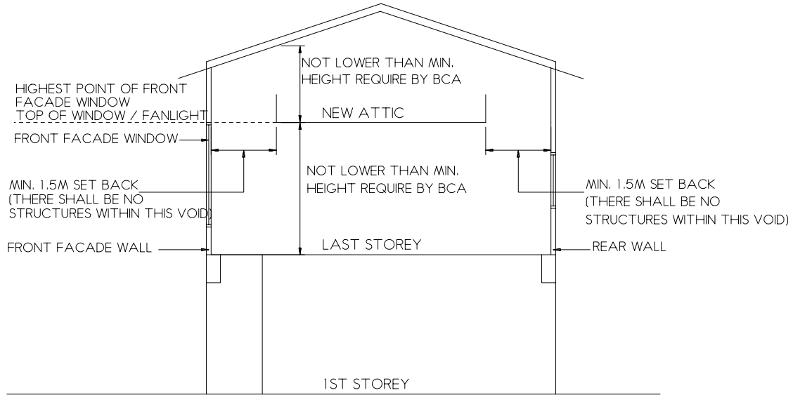
TYPICAL SECTION
