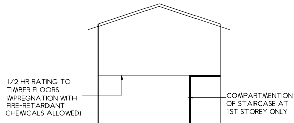
a) RETAIN EXISTING 2-STOREY SHOPHOUSE
