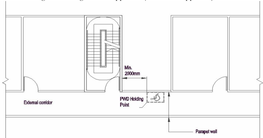
Diagram 3.2.3(a) - 3
