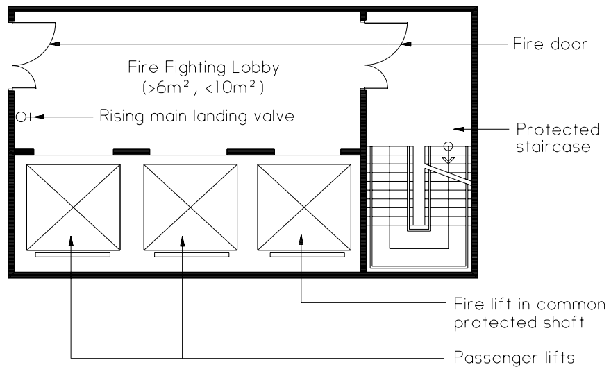
Diagram 6.6.3(b) - 3
