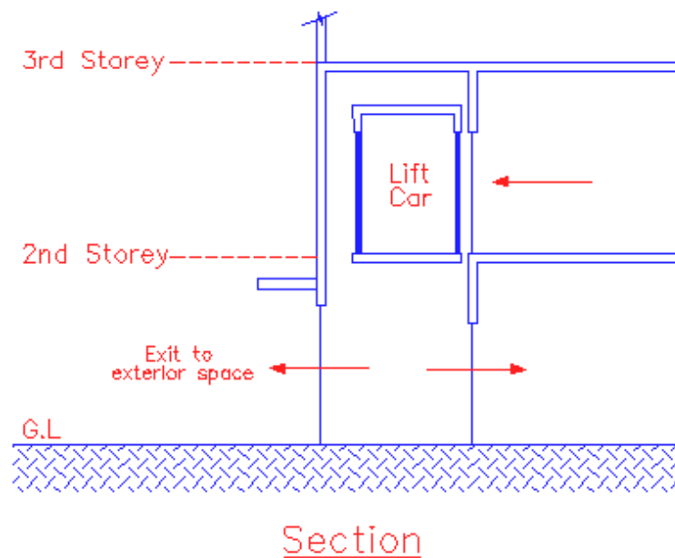
Diagram 6.6.4(f)
