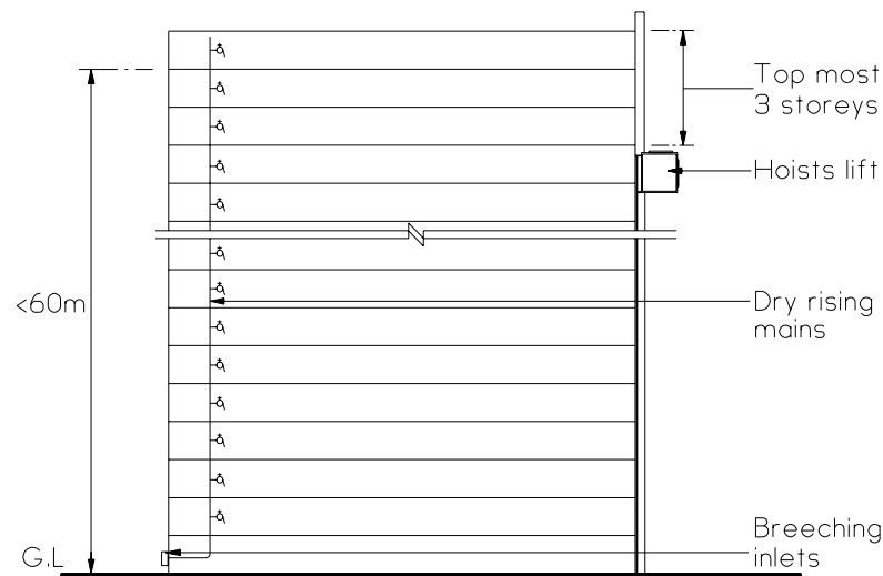
Diagram 6.2.6 - 1
