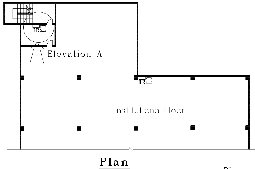
Diagram 6.3.3 - 1
