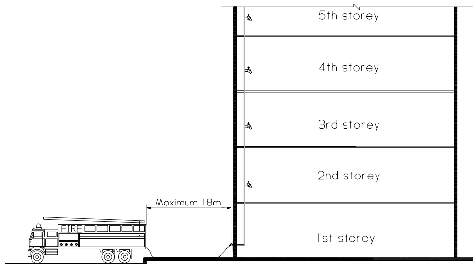
Diagram 6.2.3(a)
