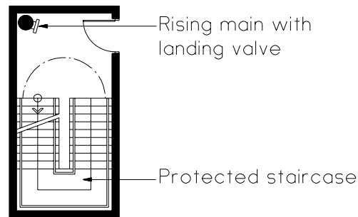
Diagram 6.2.2(b)(iii)
