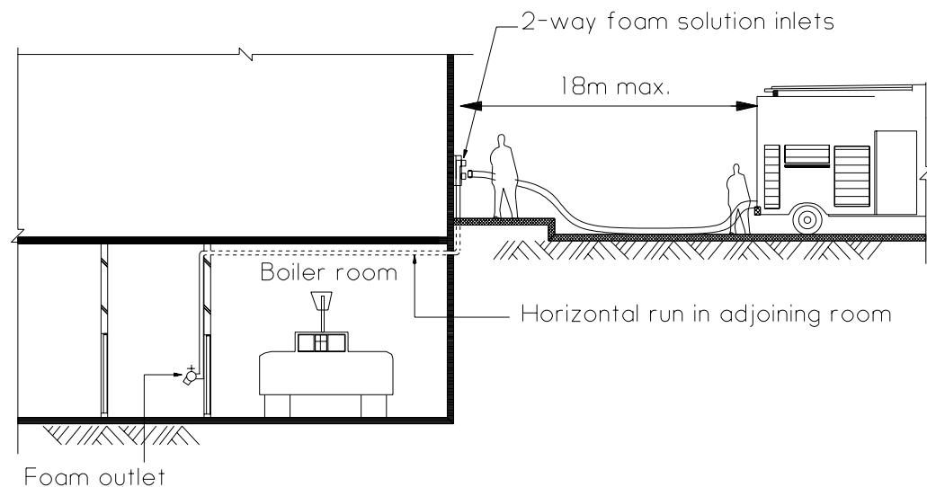
Diagram 6.2.7
