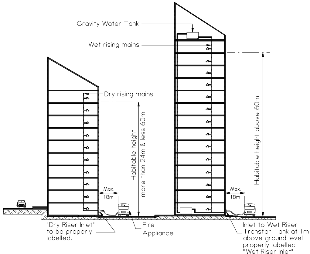
Diagram 6.2.1(c)
