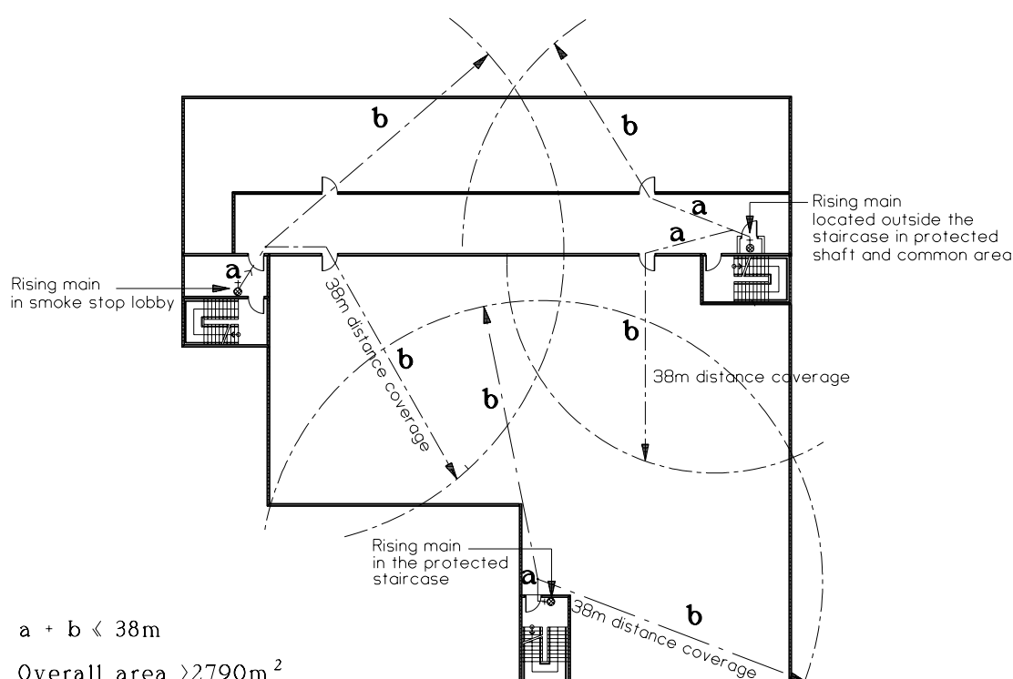
Diagram 6.2.2(a) - 1
