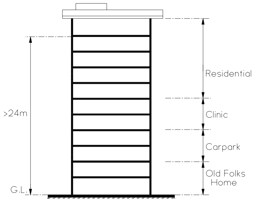
Diagram 6.4.1(c) - 3
