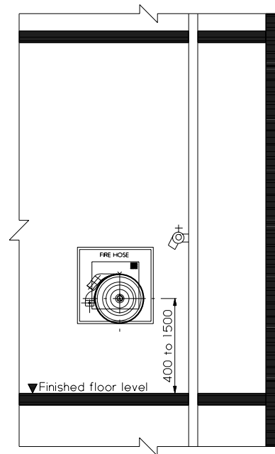
Detail 'A'
