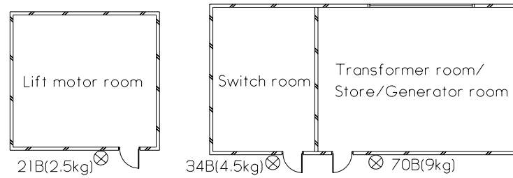
Diagram 6.1.2 - 2
