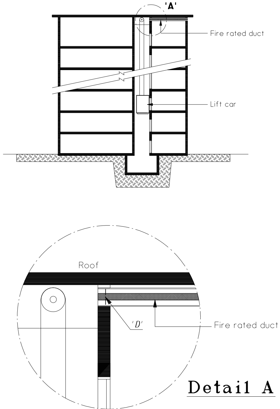
Drawing 6.6.1 – 2
