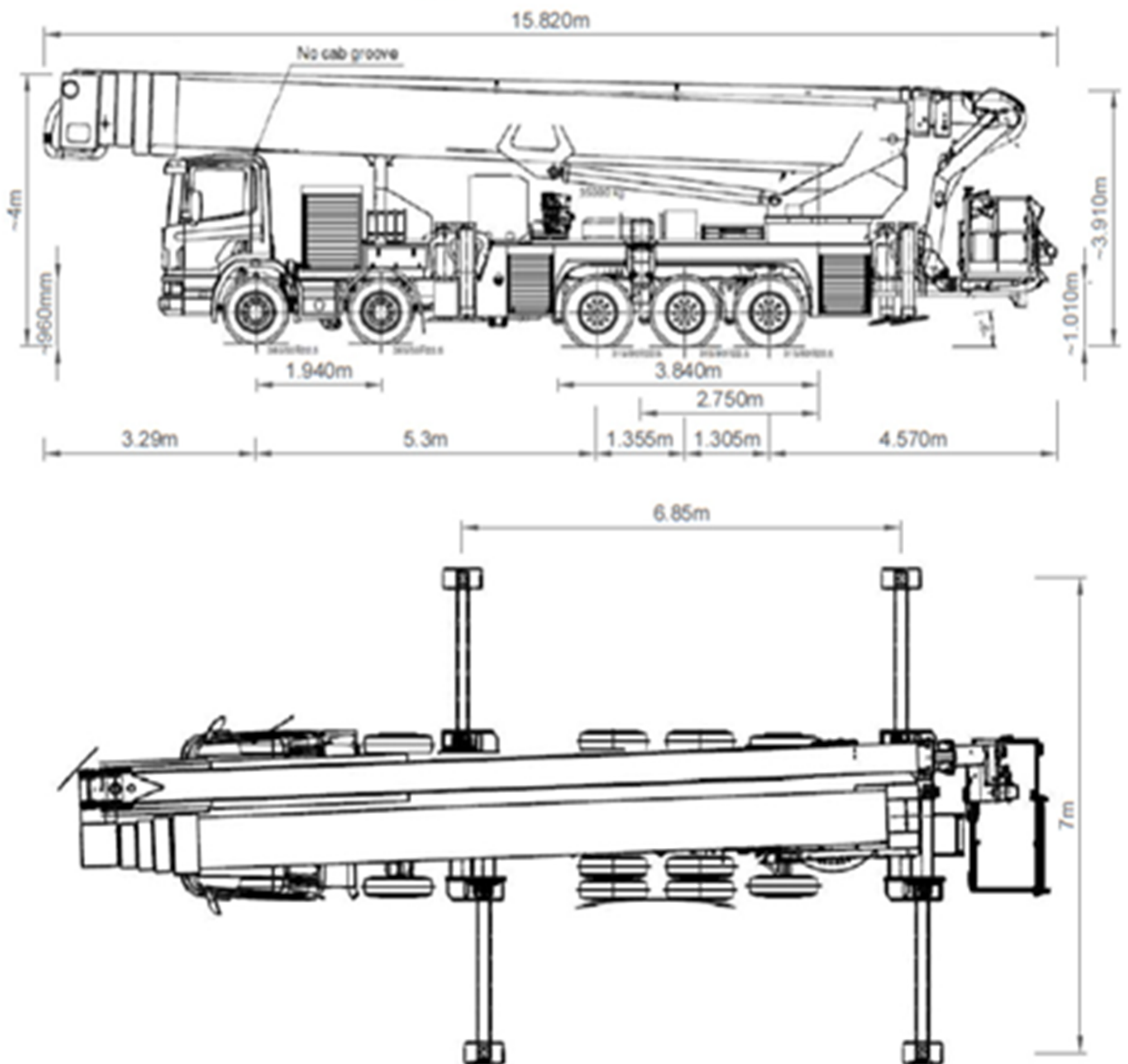
Diagram 4.2.4d.(1) – 3: HL 90 Firefighting Appliances – Wheels & Jacks Layout
