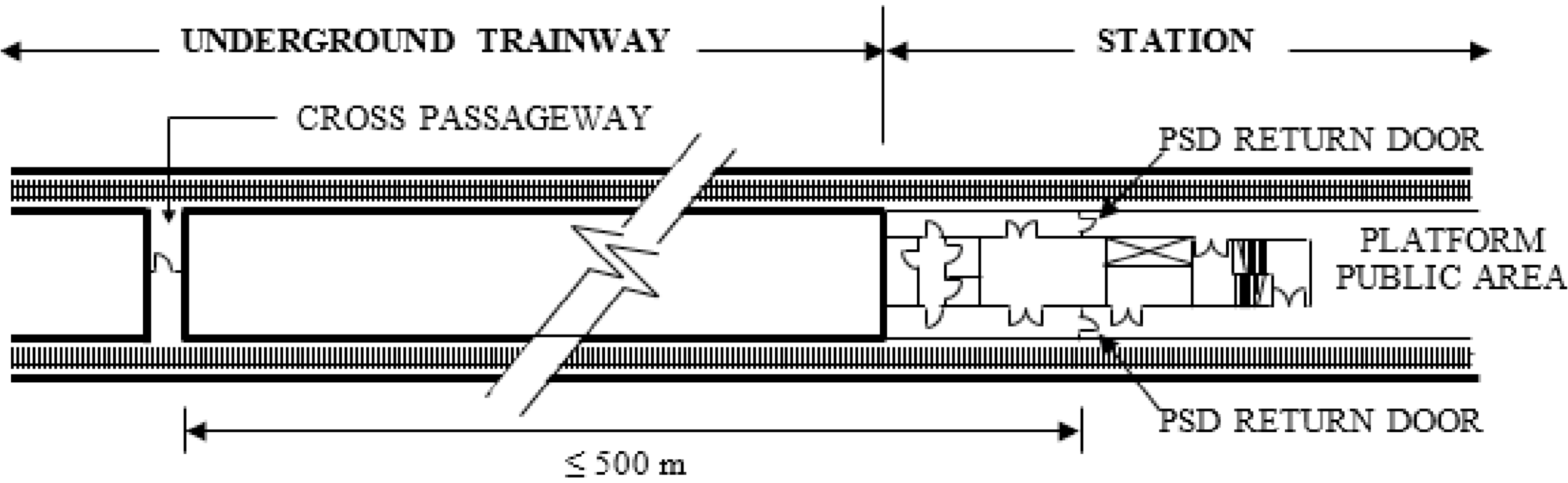
Diagram 9.3.3a.: Location of First Cross-passageway in Underground Trainways
