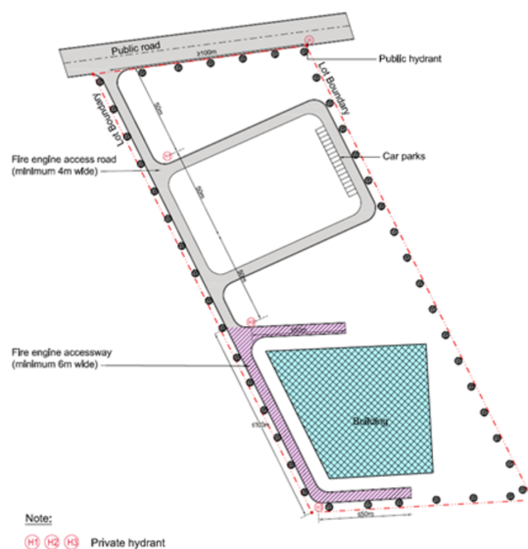
Diagram 4.4.1c.: Siting of Private Fire Hydrant
