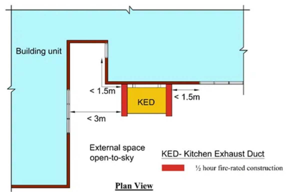
Diagram 7.1.12c.(2): Fire resistance construction for kitchen exhaust duct
