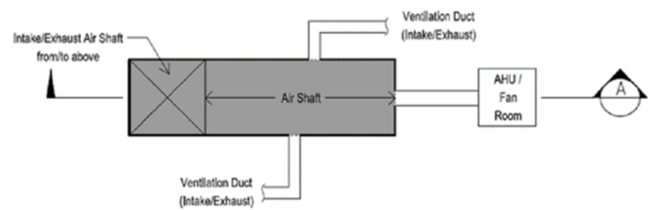
Diagram 7.1.16 – 1: Air Shaft Plan Layout
