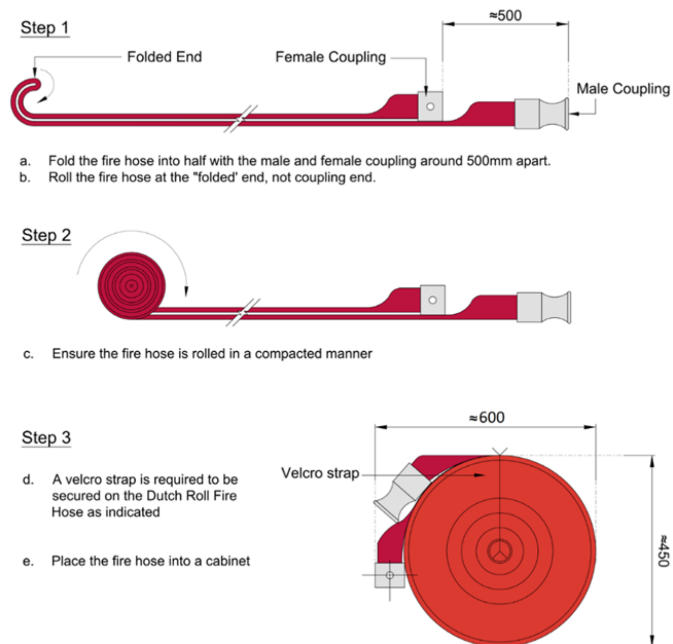
Diagram 6.2.4c.(9): Dutch Roll Folding Method
