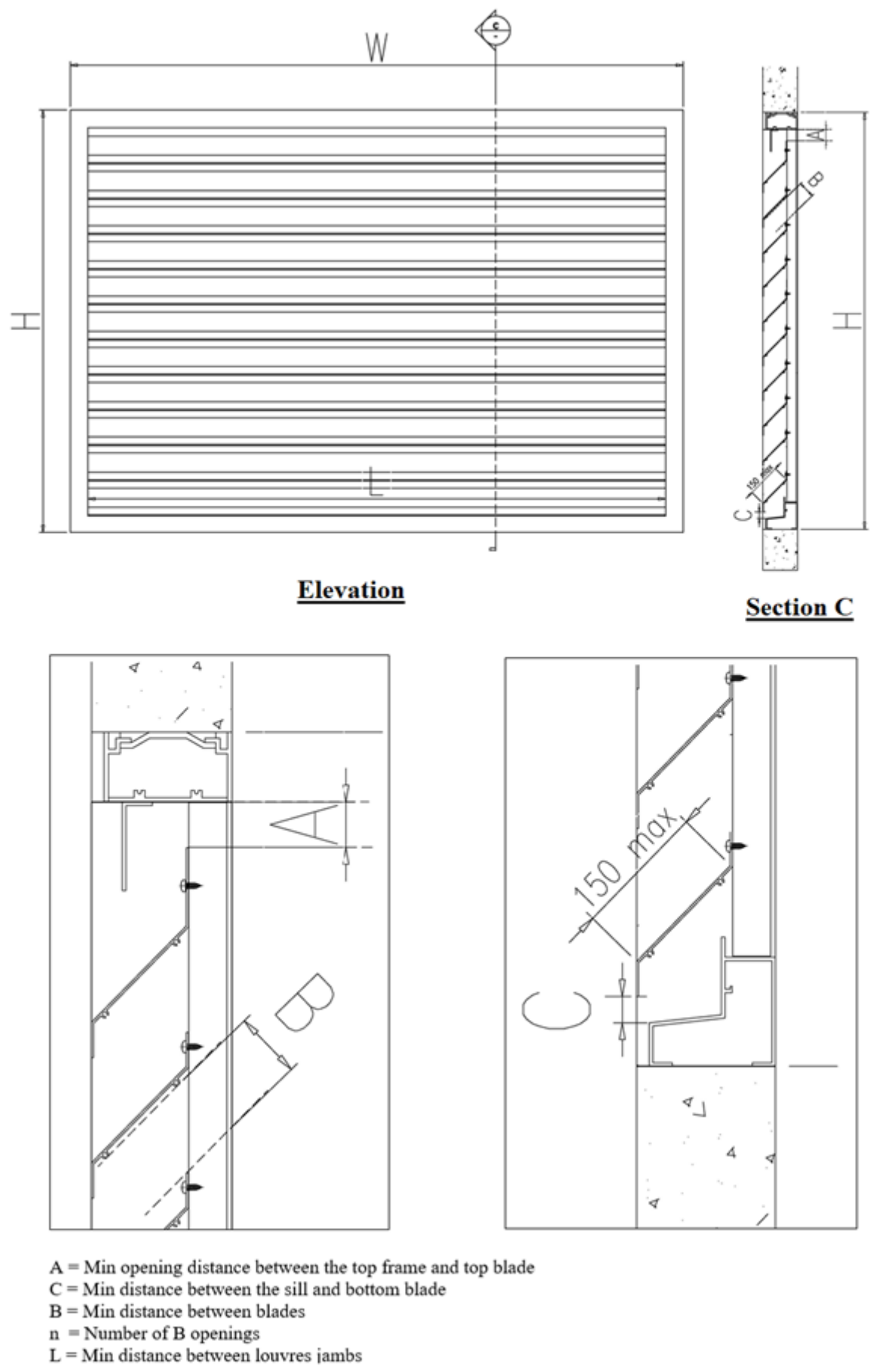
Diagram 1.4.87: Ventilation Opening Size
