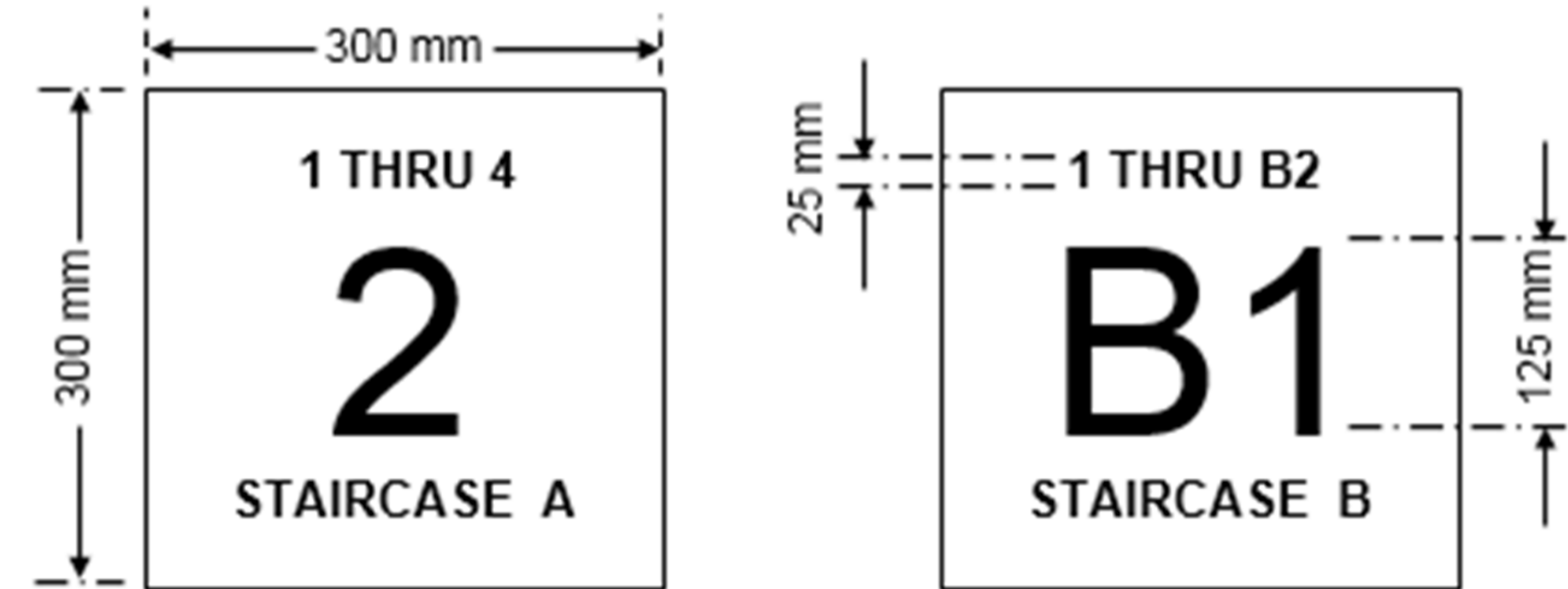
Diagram 2.2.10h.: Stair Identification Sign
