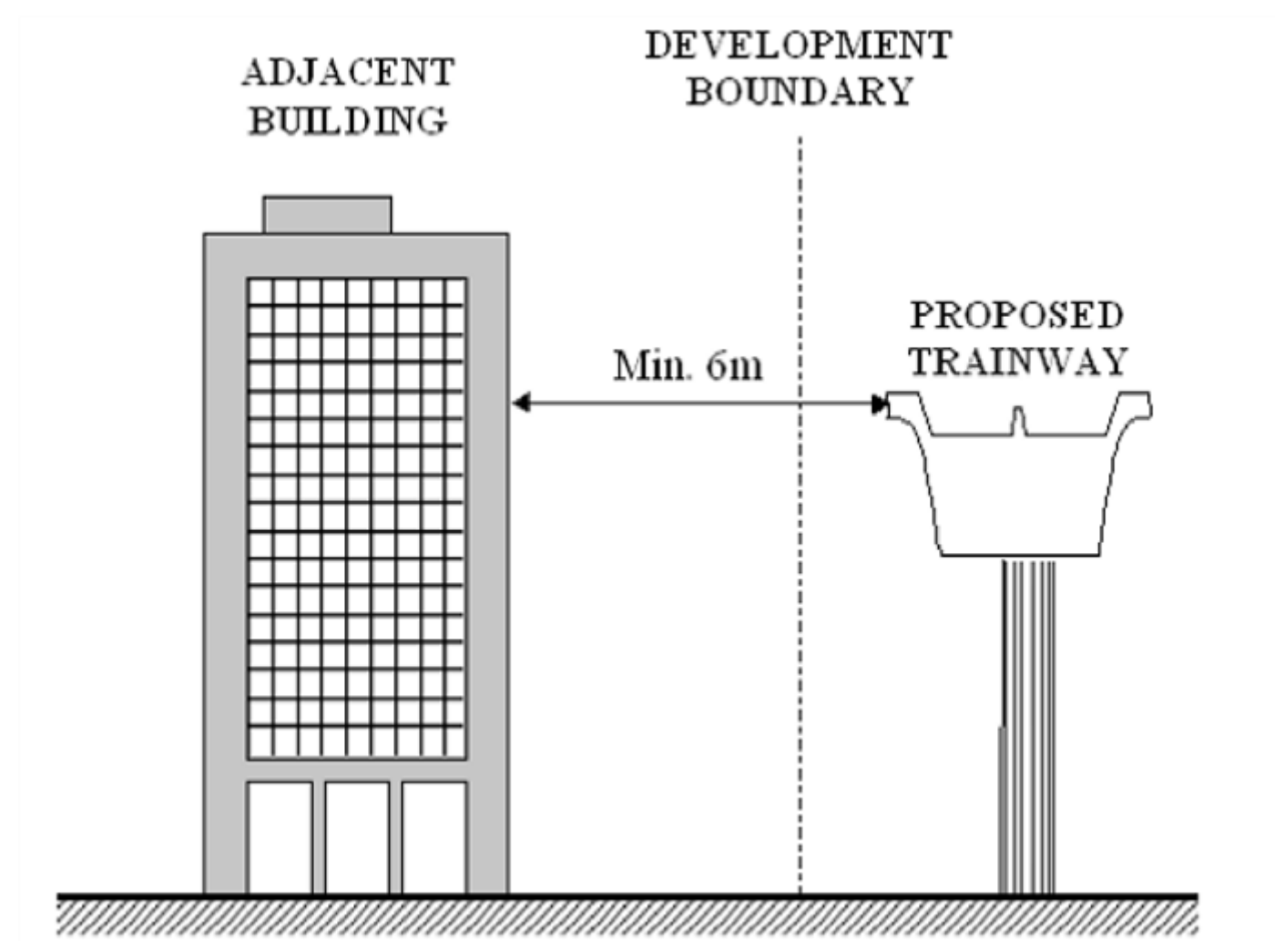
Diagram 9.4.2b.: Separation Distance – Proposed Trainway Outside Development Boundary
