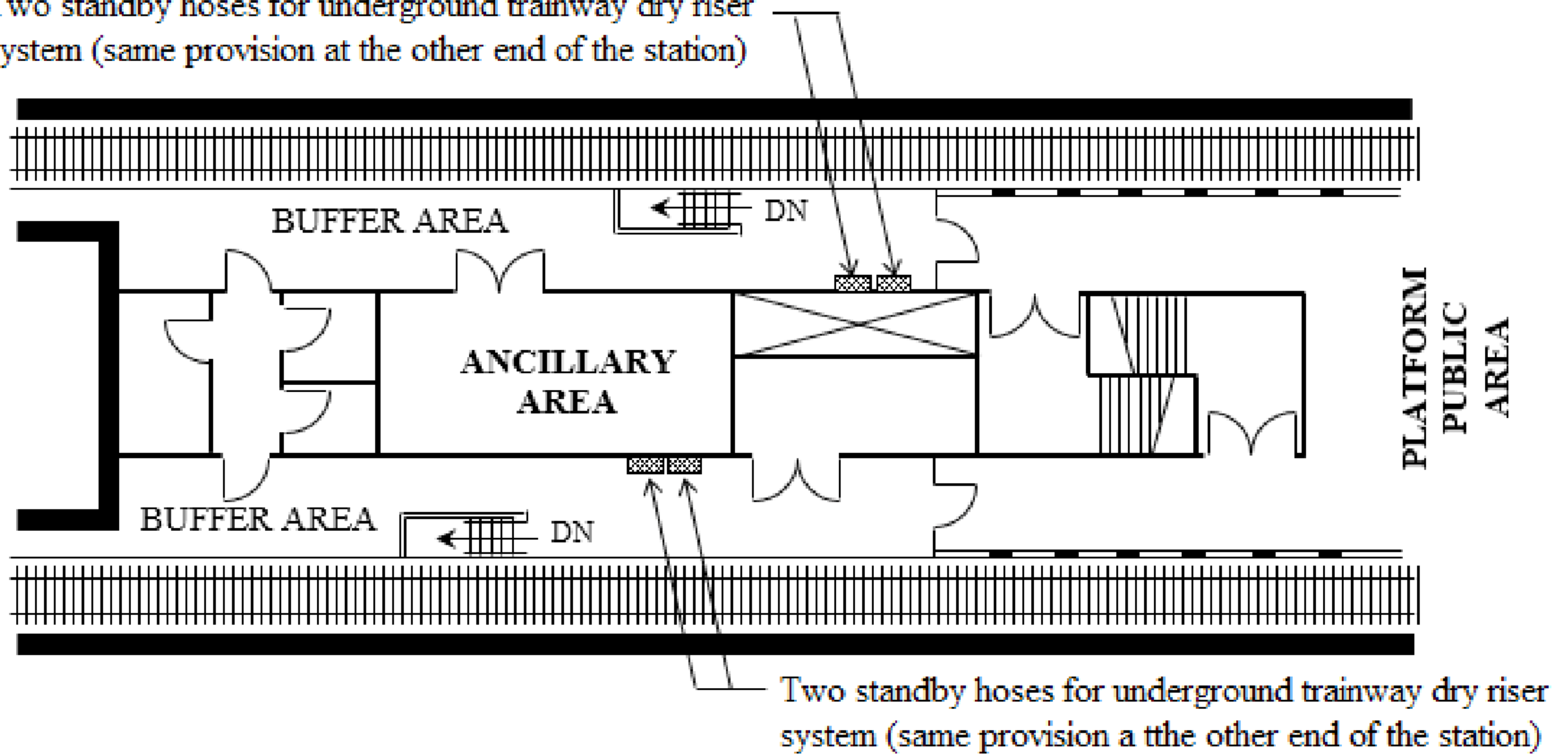
Diagram 9.3.9a(9)(a): Location of Standby Hoses Outside Platform Public Area
