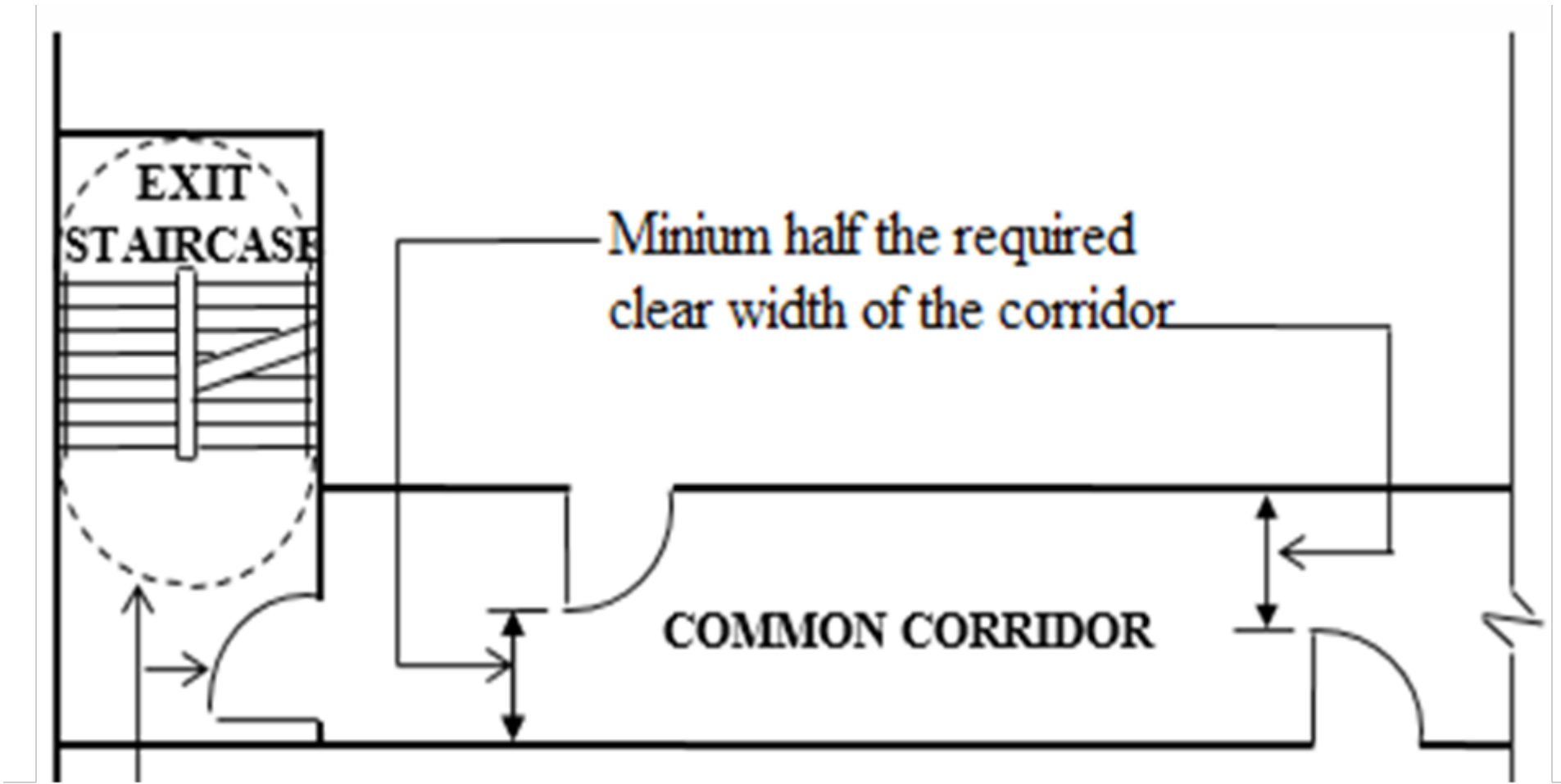
Diagram 2.2.17e.(1): Exit Doors Opening into Exit Staircases and Exit Passageways
