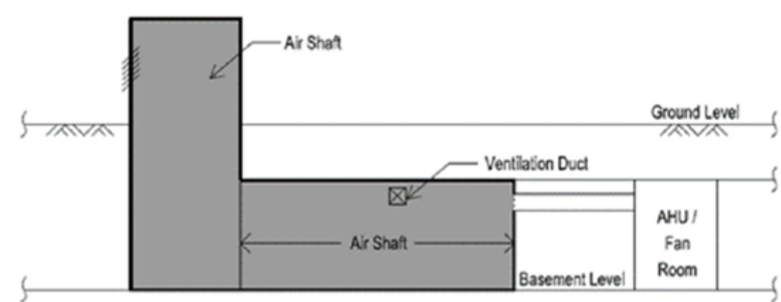
Diagram 7.1.16 – 2: Air Shaft Section A-A
