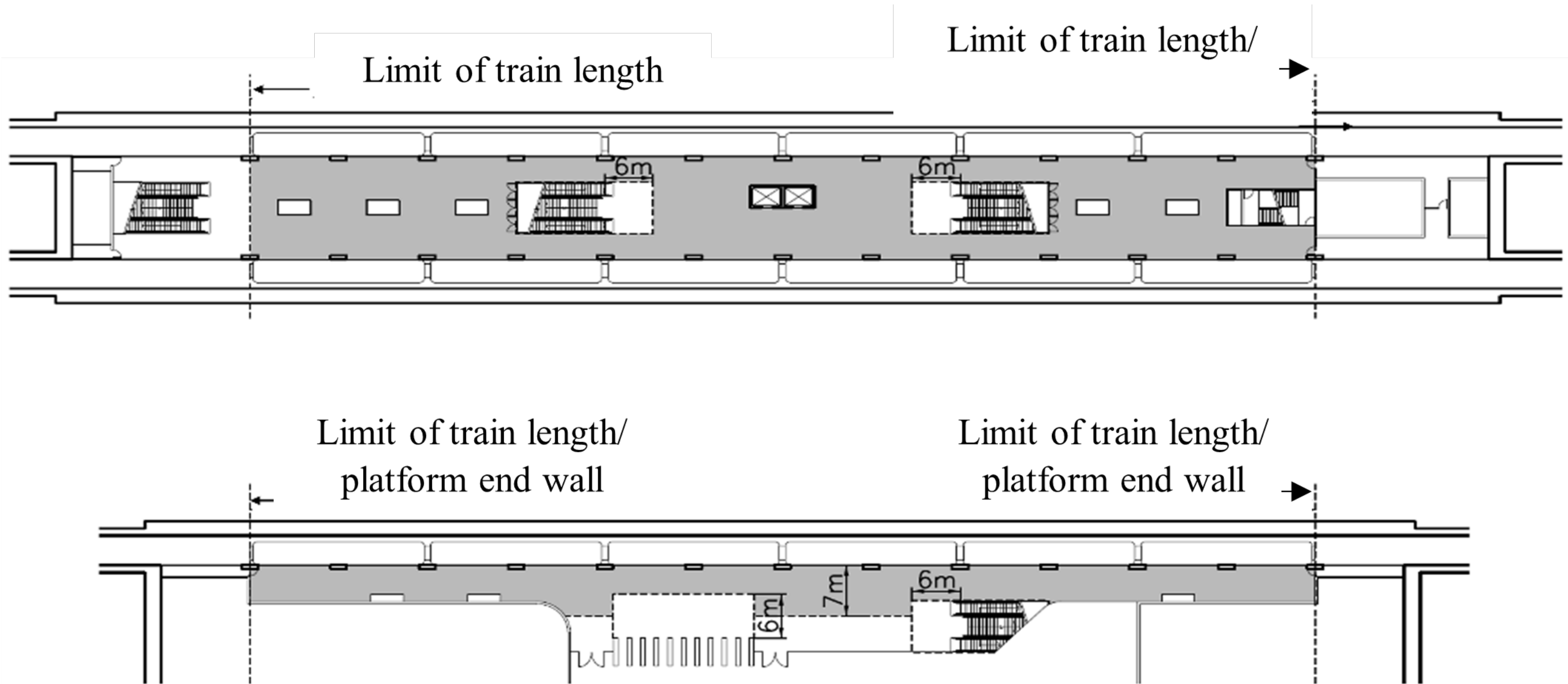
Diagram 1.4.80: Layout of Station Platform
