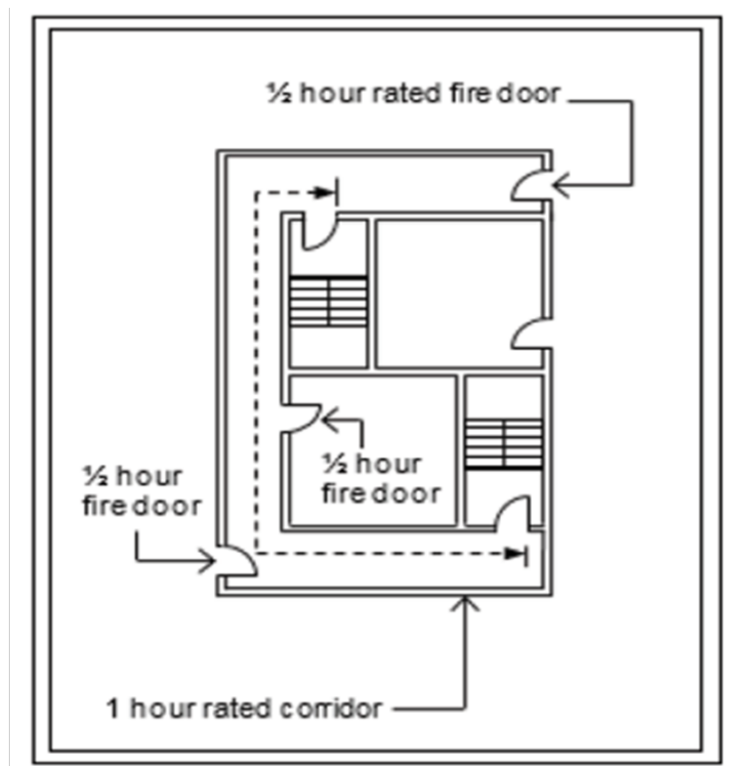
Diagram 2.2.19c.: Remoteness of Exit
