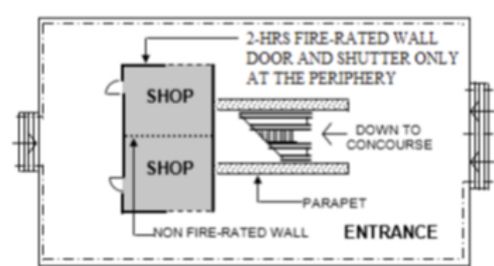
Diagram 3.2.4c.: Compartmentation of Commercial Spaces
