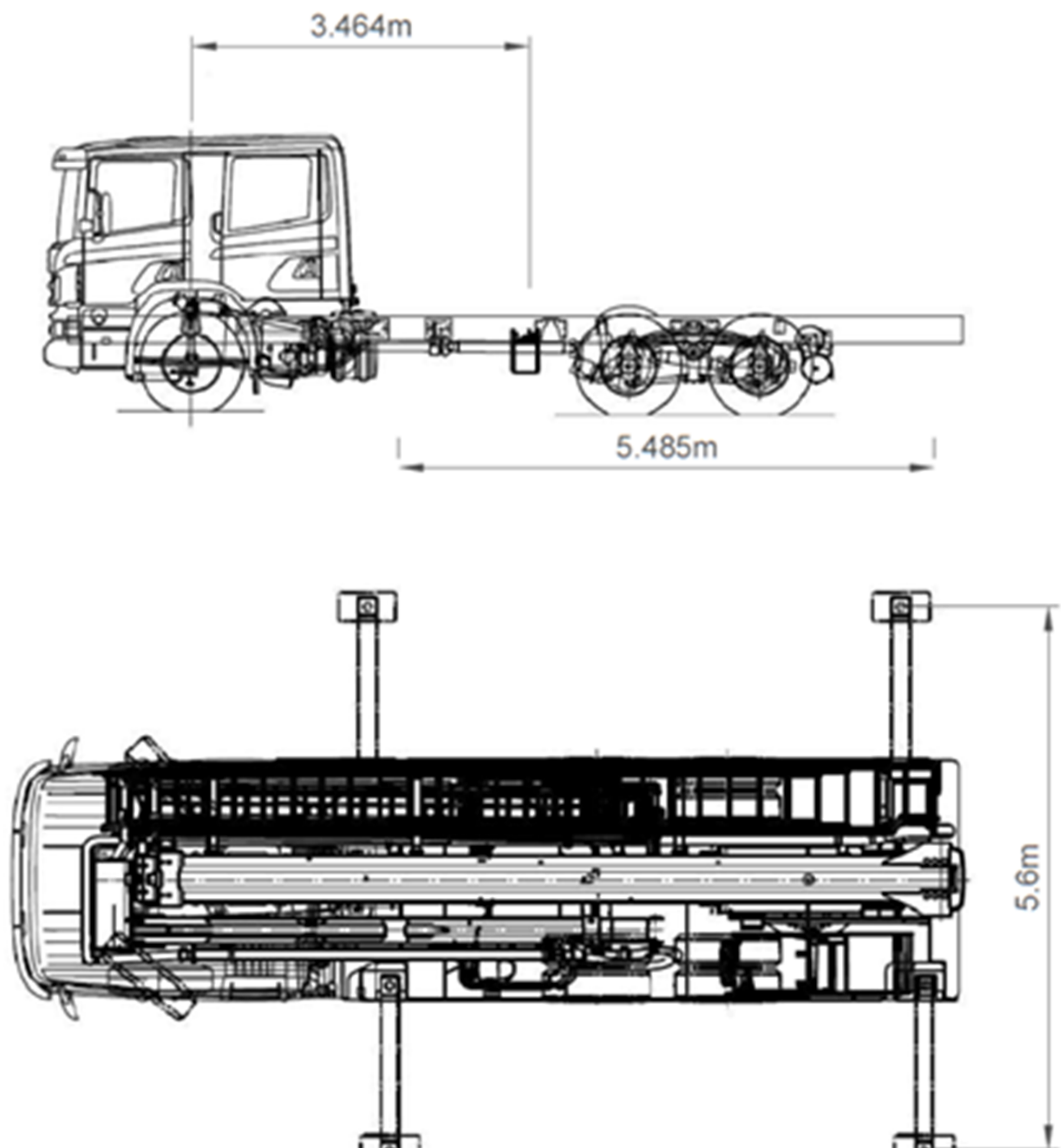
Diagram 4.2.4d.(1) – 1: CPL 34 Firefighting Appliances – Wheels & Jacks Layout
