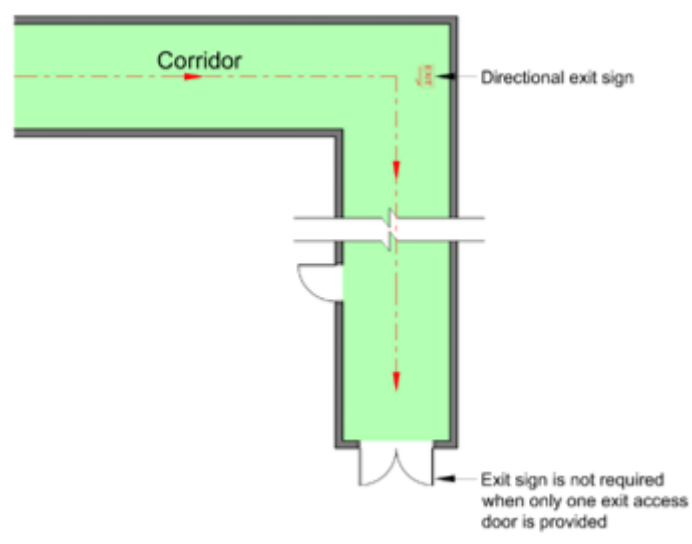
Diagram 8.1.7b.(1): Location of directional signs
