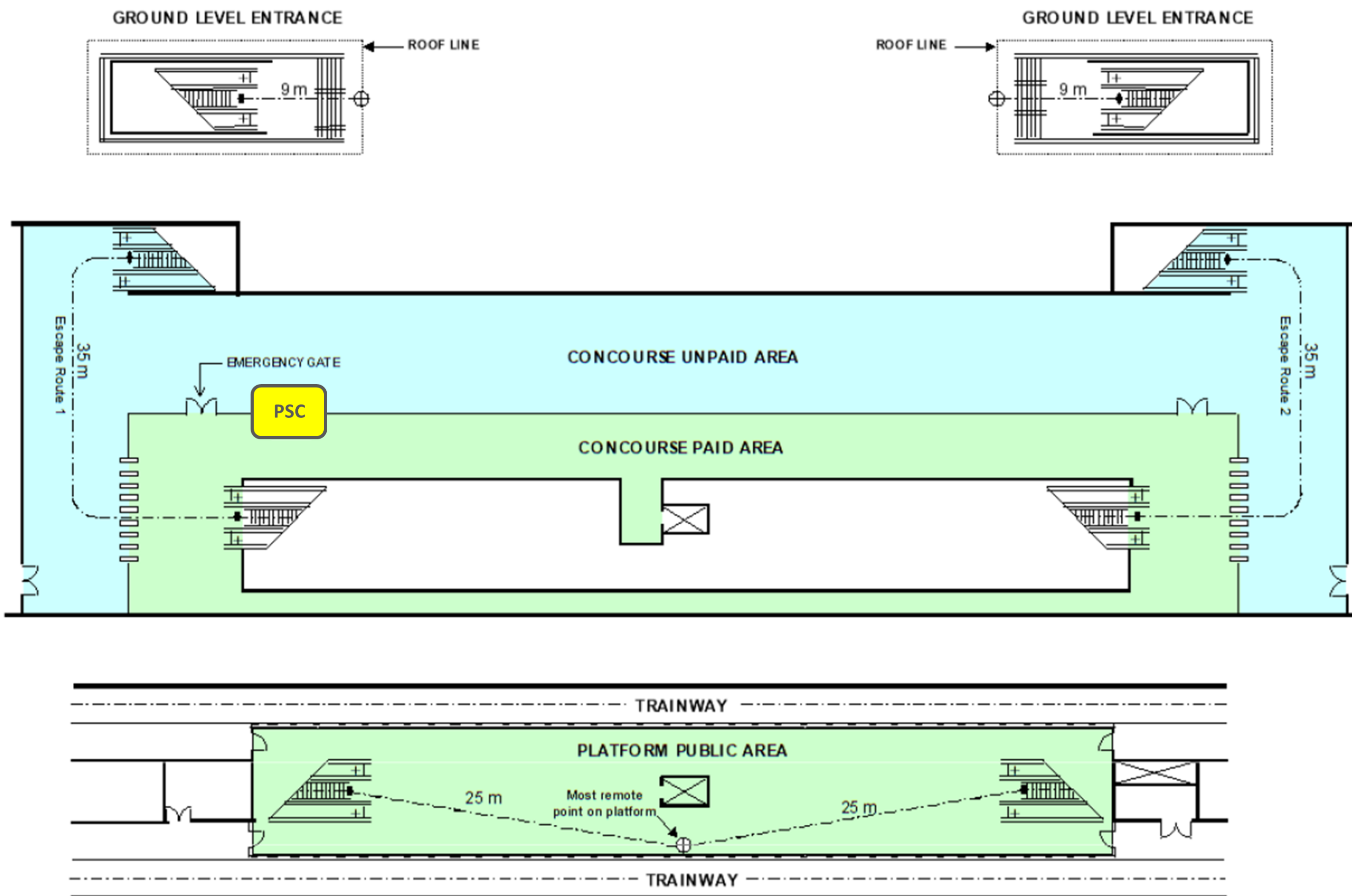
Figure A-2.1: Centre Platform Station
