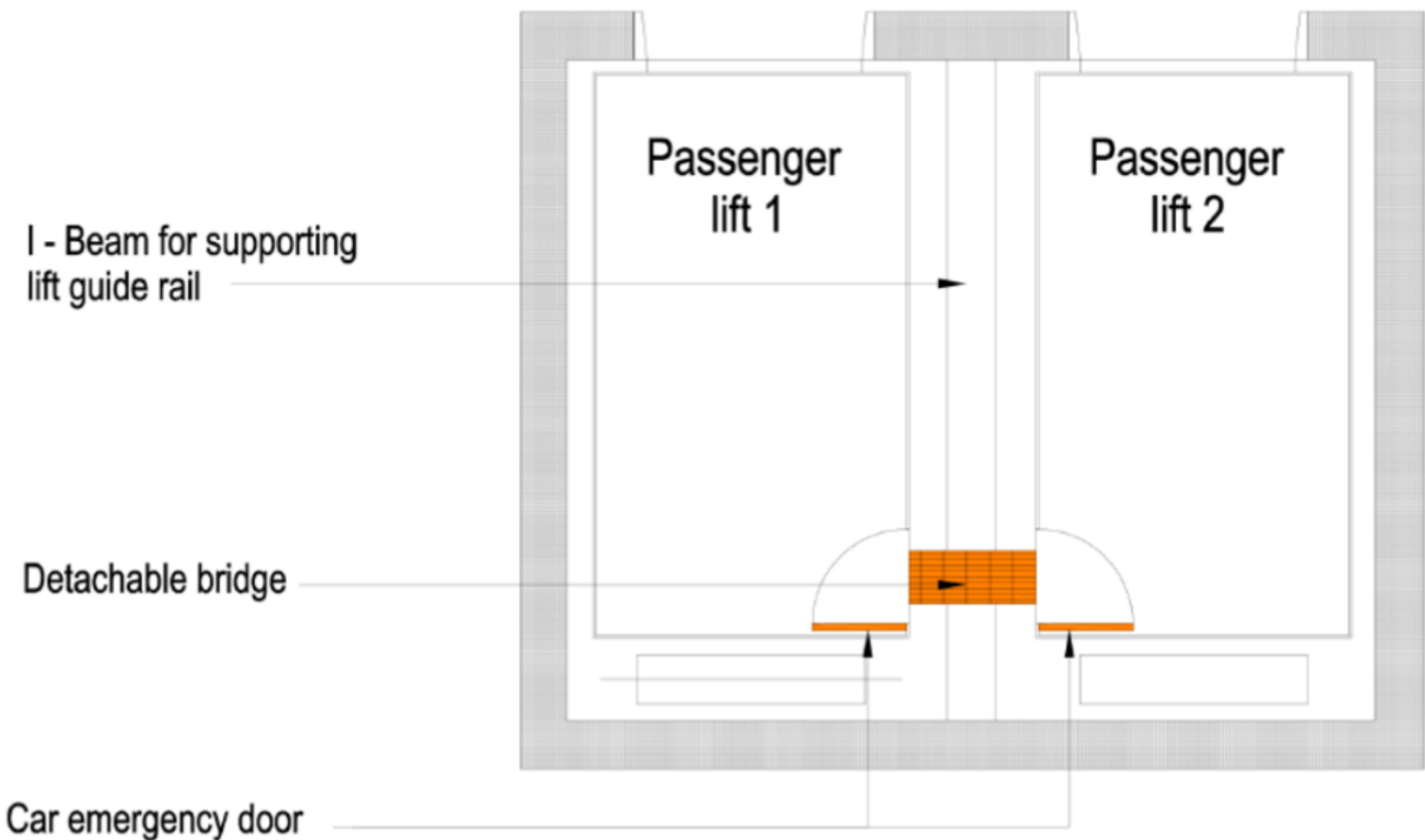
Diagram 6.6.9d.(2): Car Emergency Doors – Deployed of Bridging Plate
