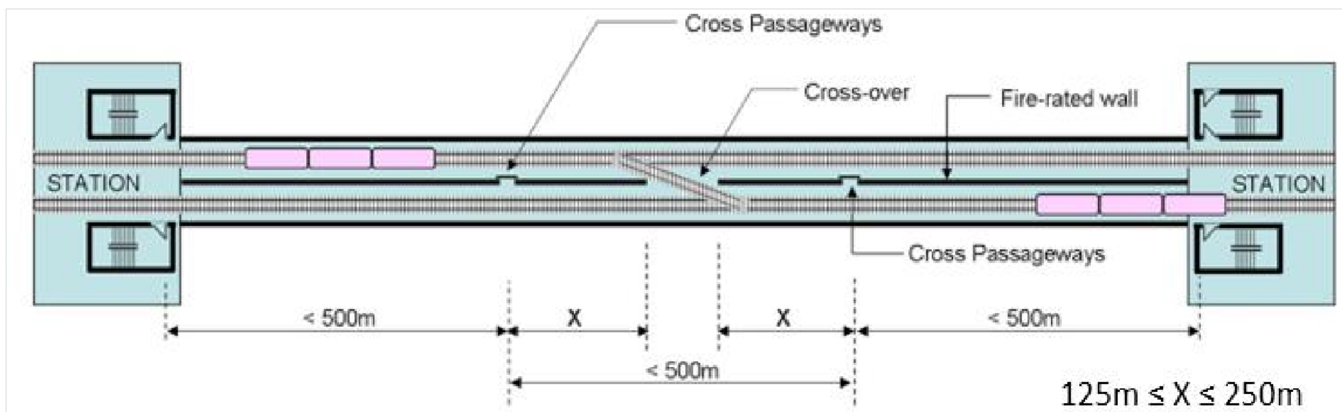
Diagram 9.3.3g.: Cross-over Between Enclosed Trainways
