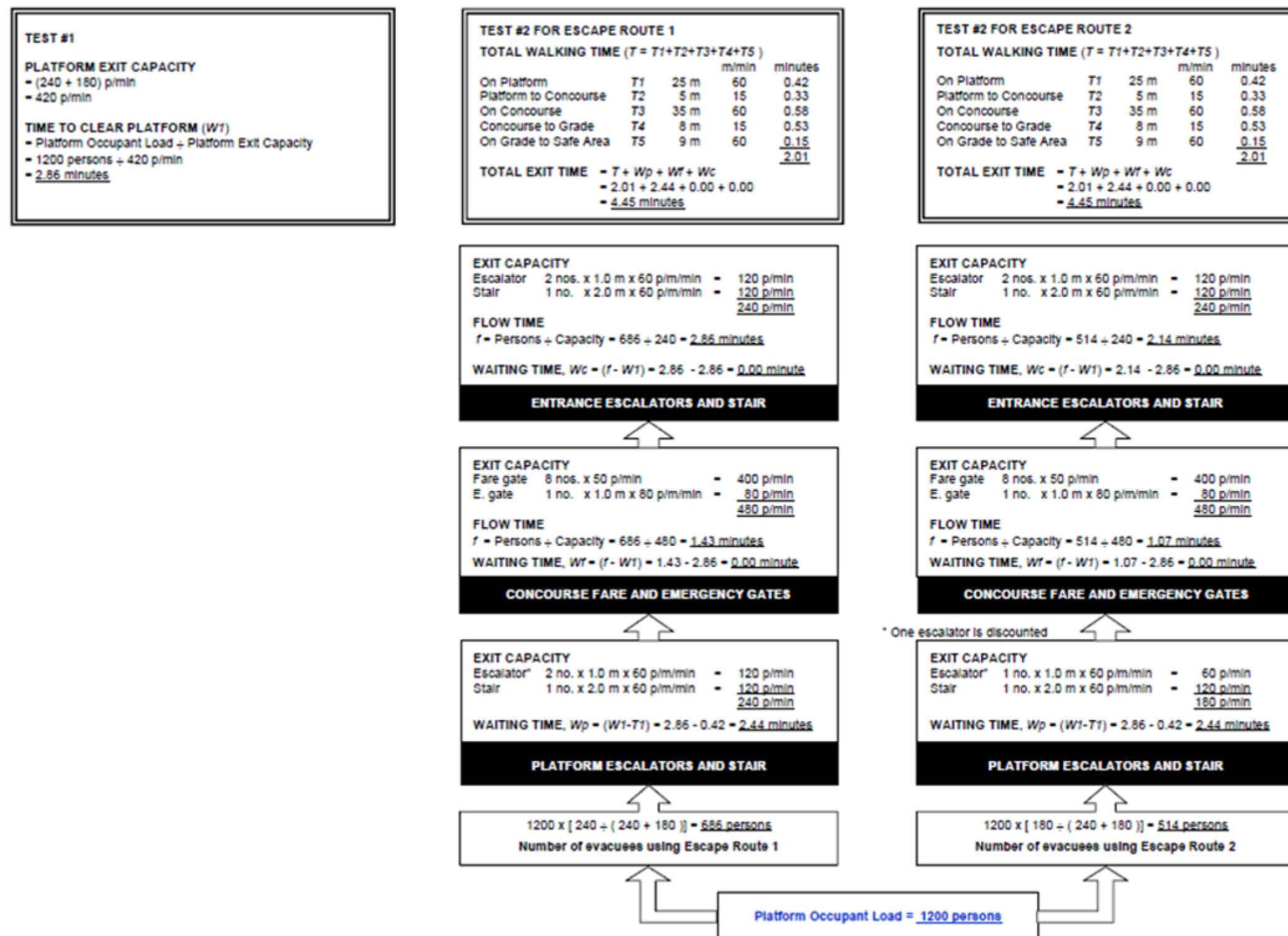
Figure A-2.2: Egress Analysis
