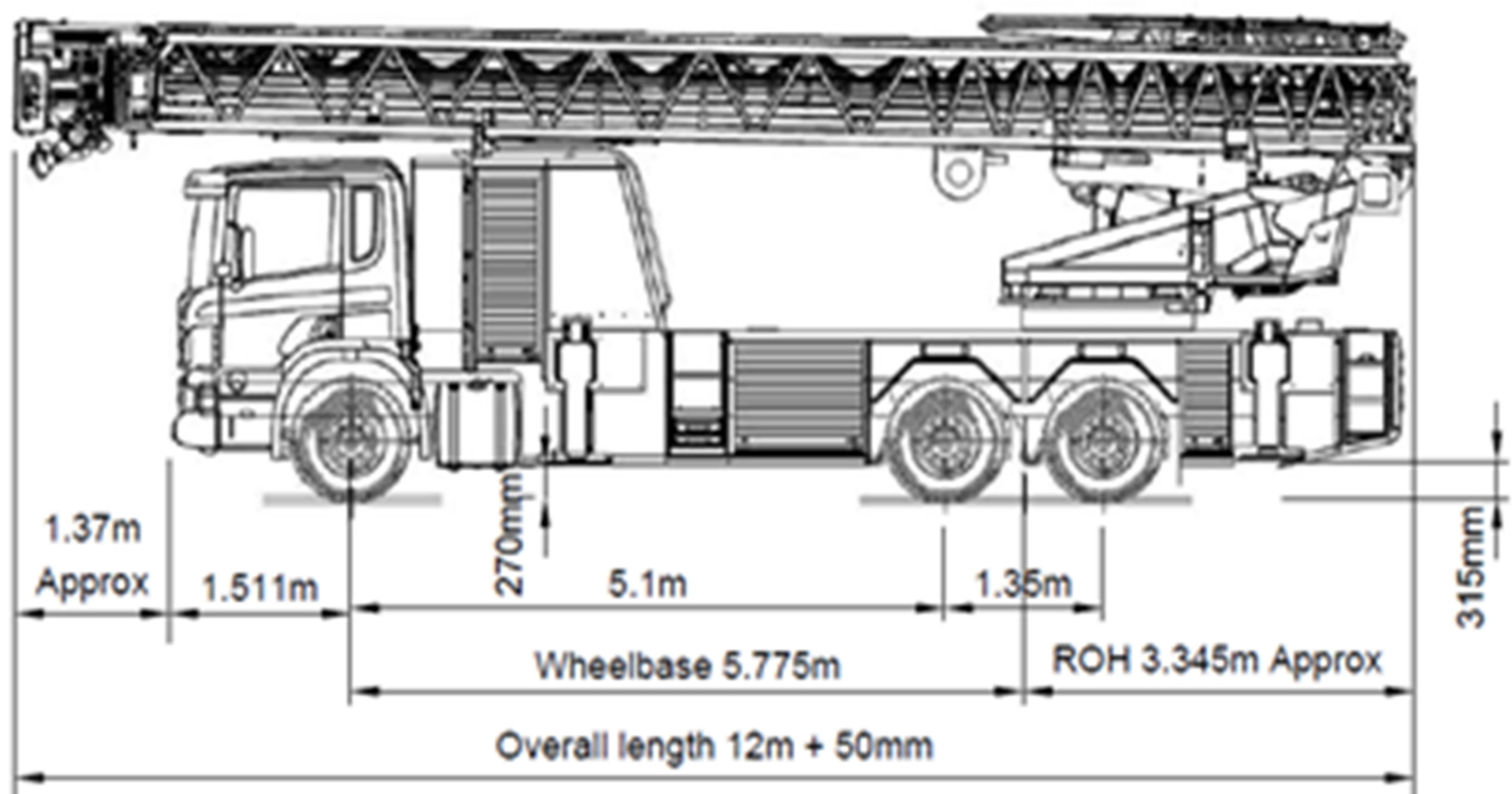
Diagram 4.2.4d(1) – 2: AL 56 Firefighting Appliances – Wheels & Jacks Layout
