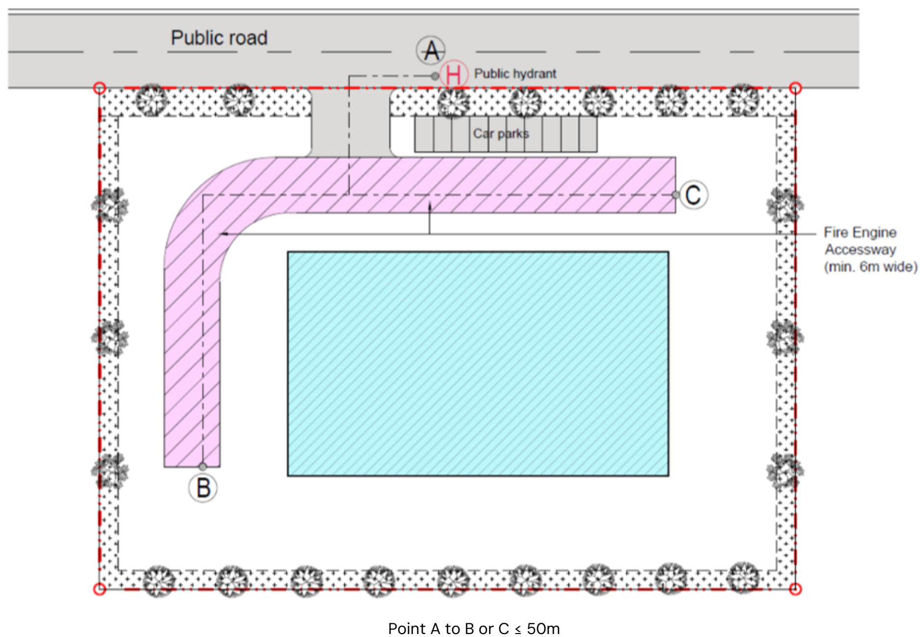
Diagram 4.4.1a.: Provision of Private Fire Hydrant
