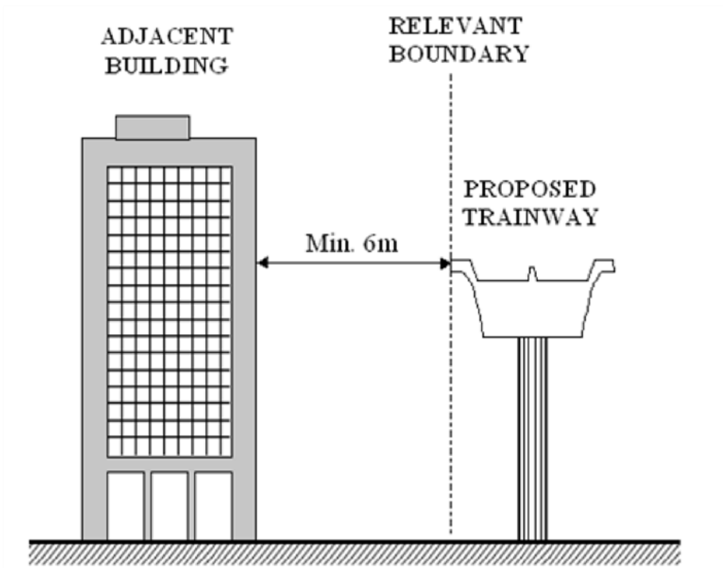
Diagram 9.4.2a.: Separation Distance
