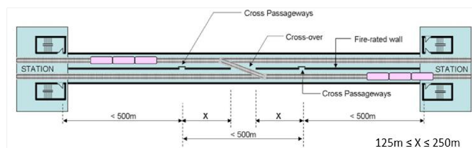
Diagram 9.3.3g: Cross-over Between Enclosed Trainways
