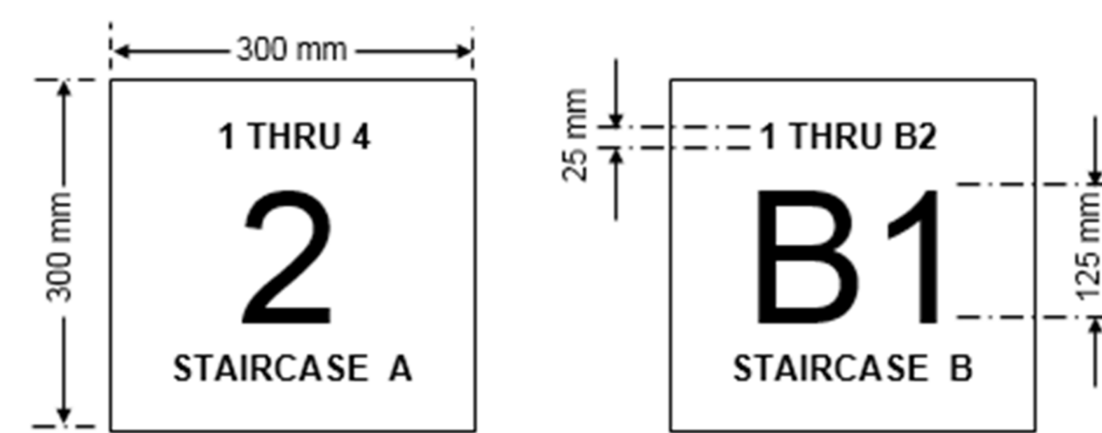
Diagram 2.2.10h: Stair Identification Sign
