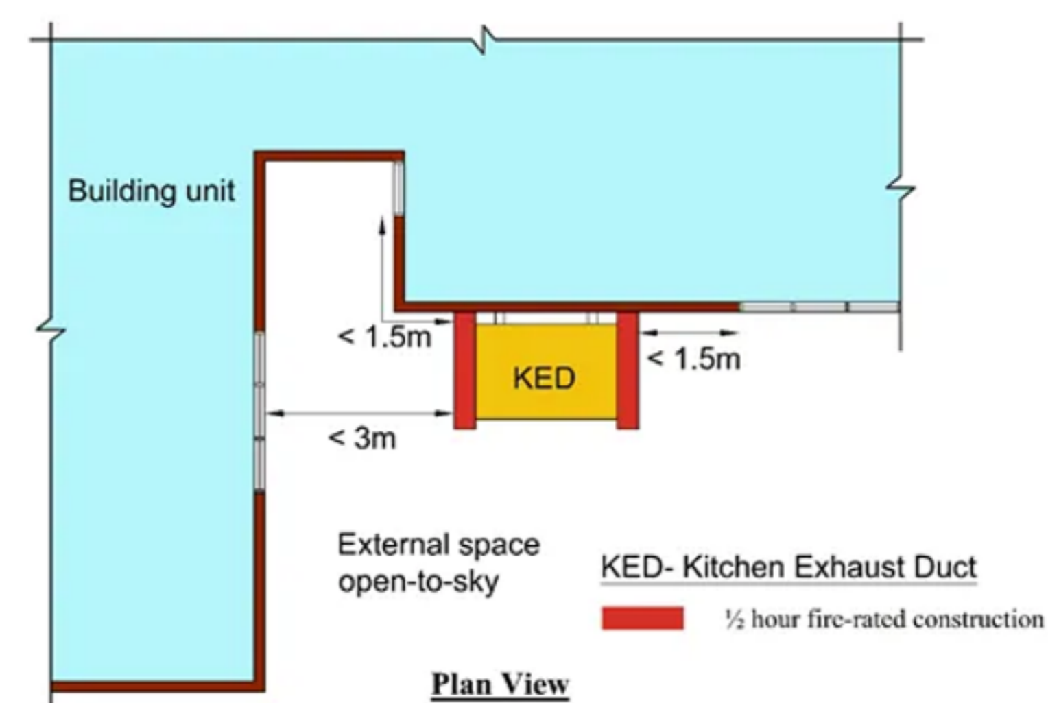
Diagram 7.1.12c(2): Fire resistance construction for kitchen exhaust duct
