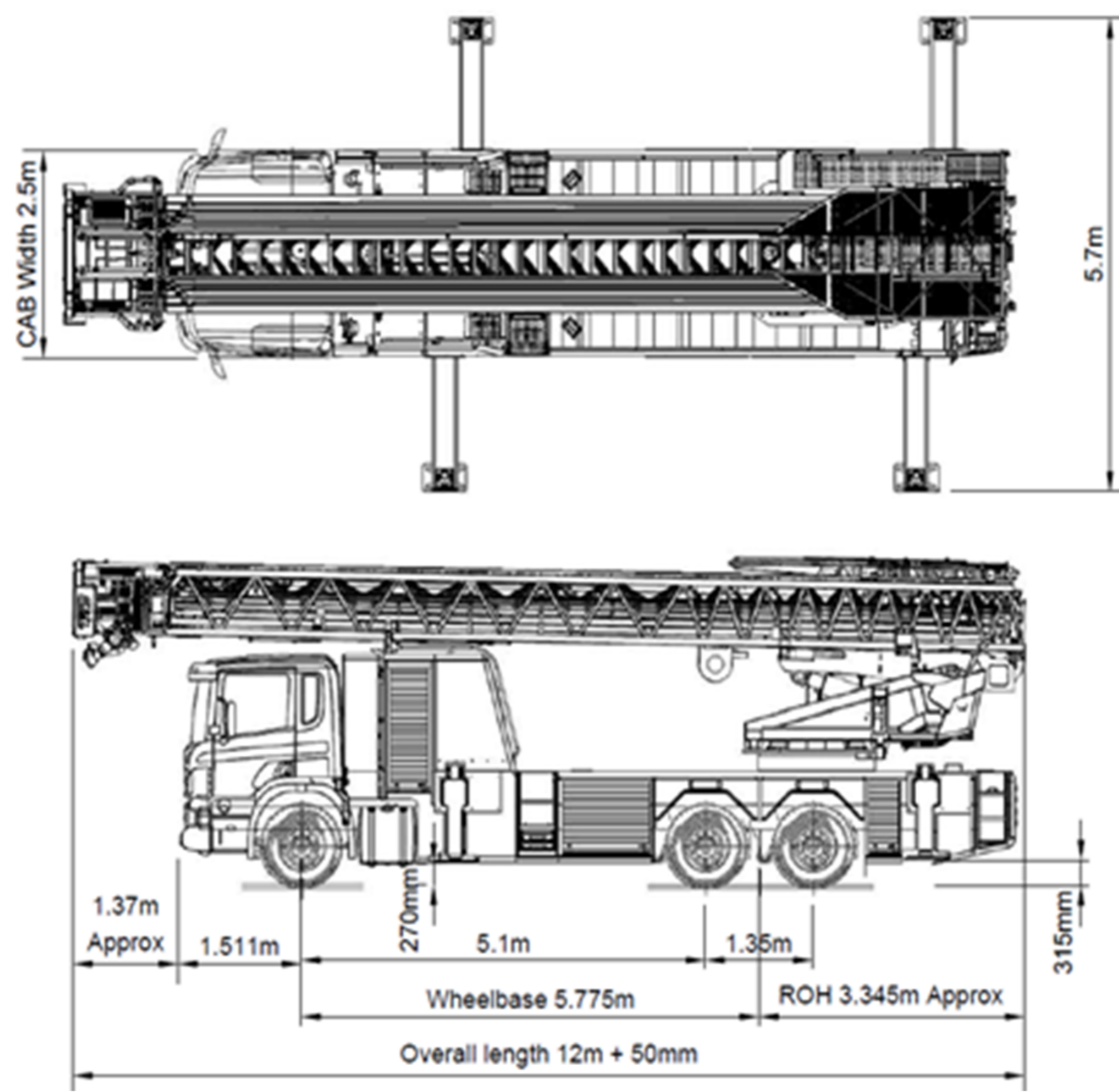
Diagram 4.2.4d.(1) – 2: AL 56 Firefighting Appliances – Wheels & Jacks Layout
