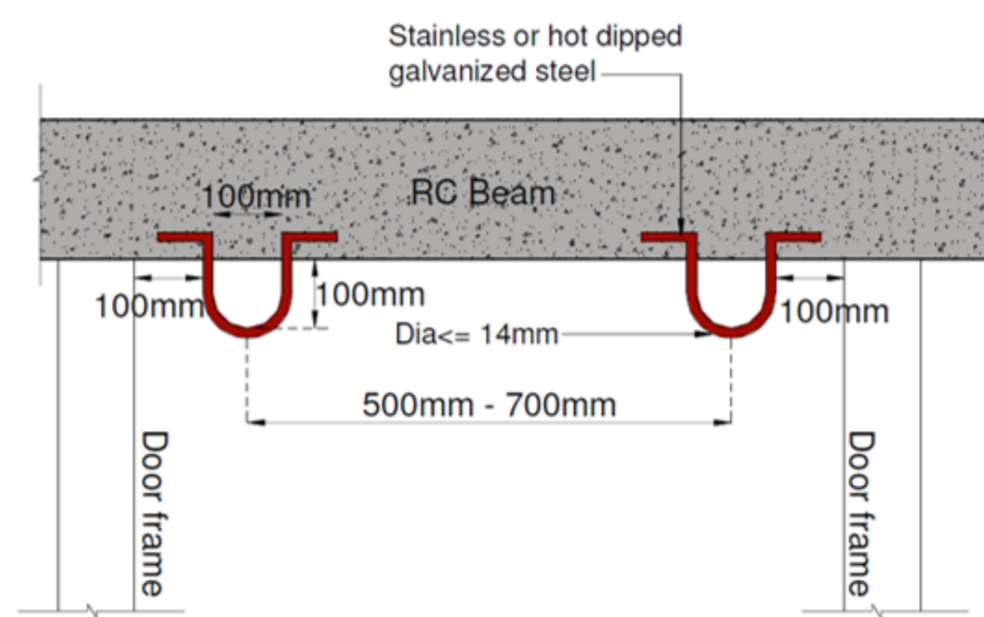
Diagram 6.6.9b(3): Rescue Hook Design
