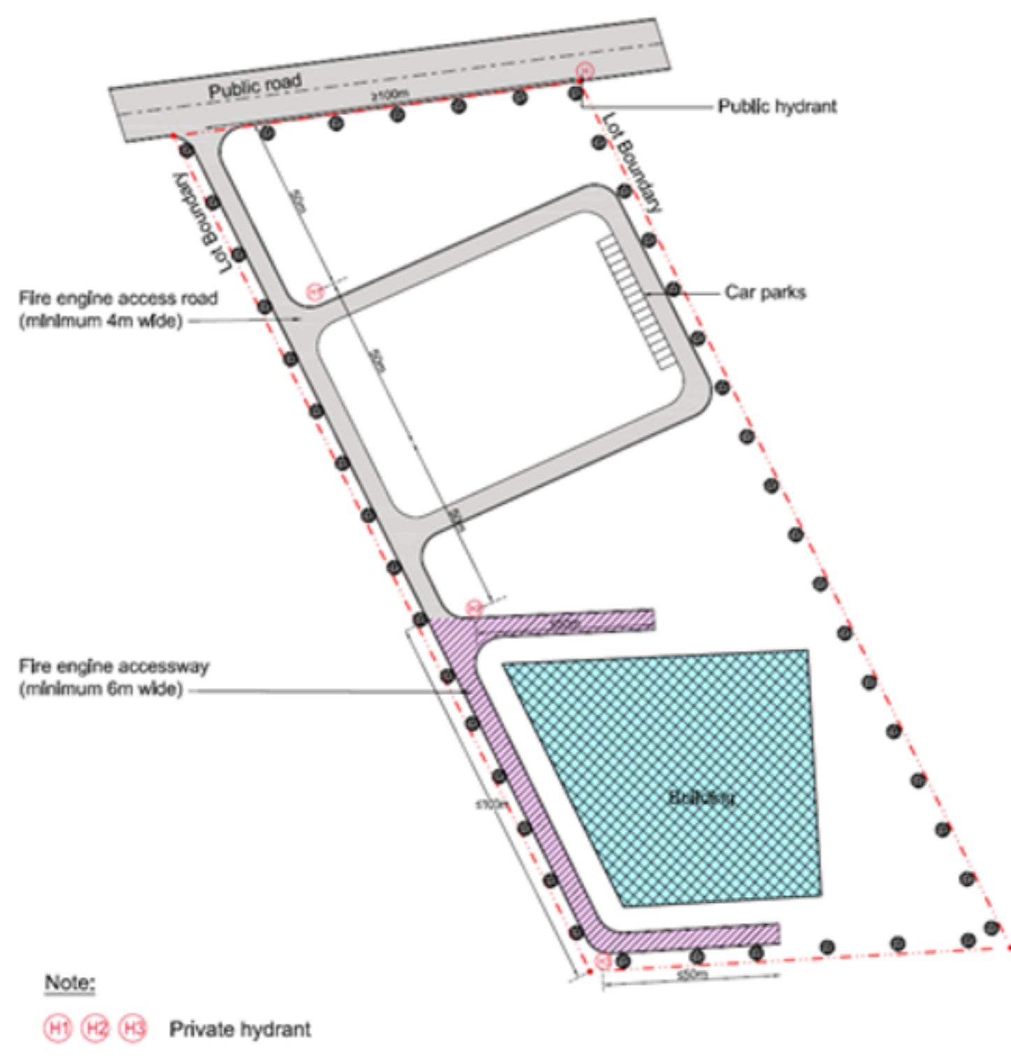
Diagram 4.4.1c.: Siting of Private Fire Hydrant
