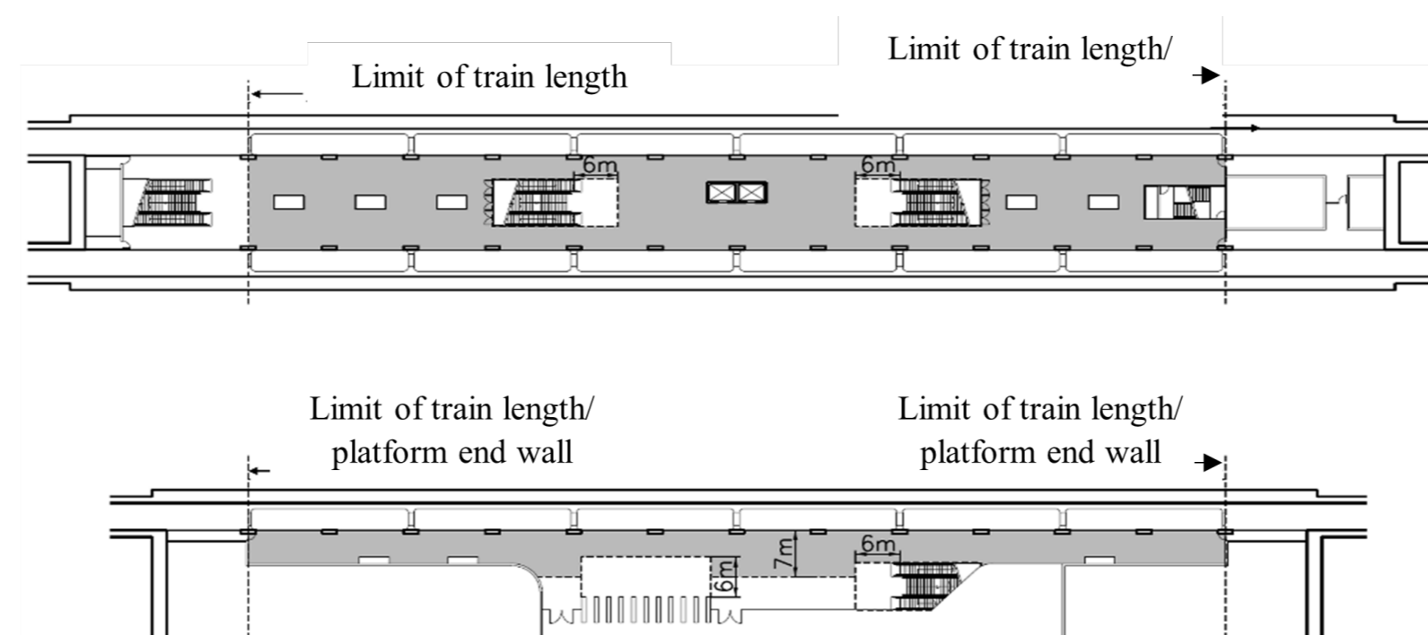
Diagram 1.4.80: Layout of Station Platform
