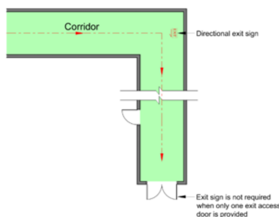
Diagram 8.1.7b.(1): Location of directional signs
