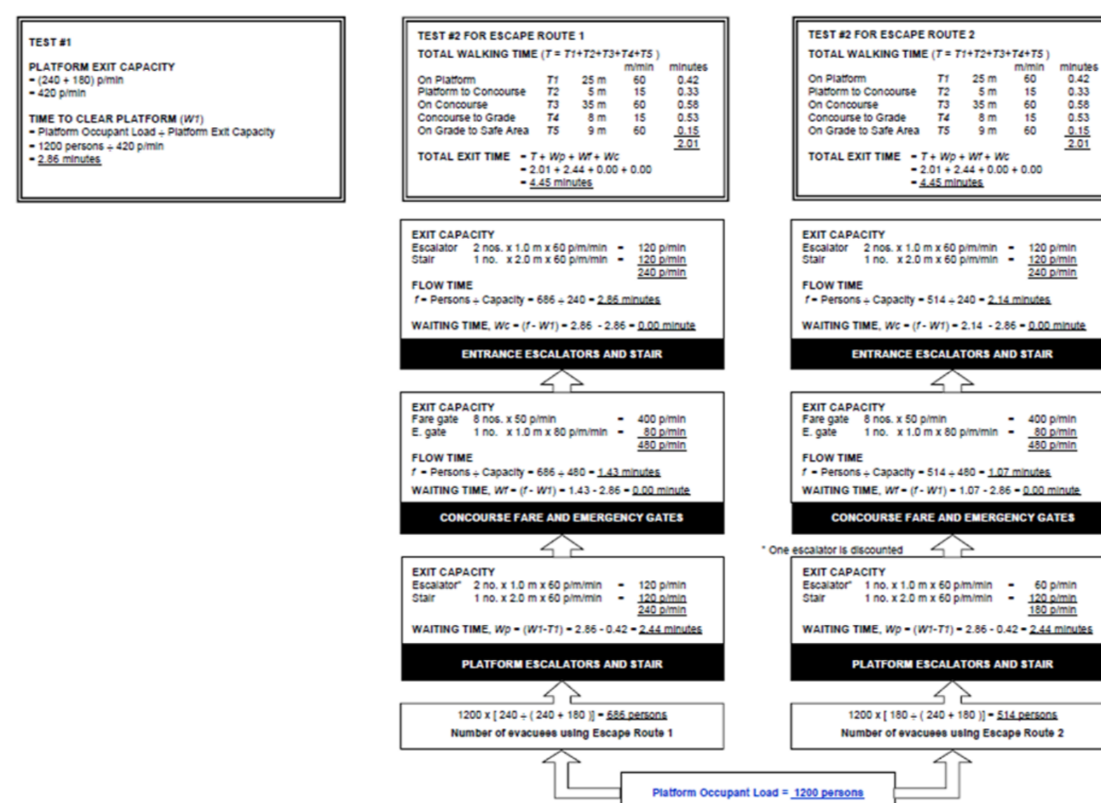
Figure A-2.2: Egress Analysis
