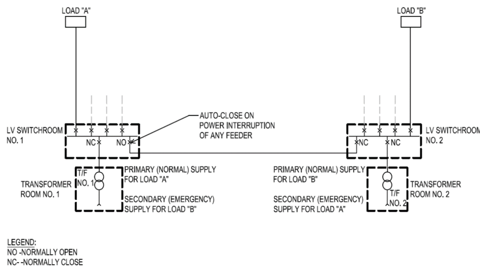
Diagram 5.2.6 – 2: Block diagram of Typical RTS Station Dual Feeder HT Power Supply Scheme
