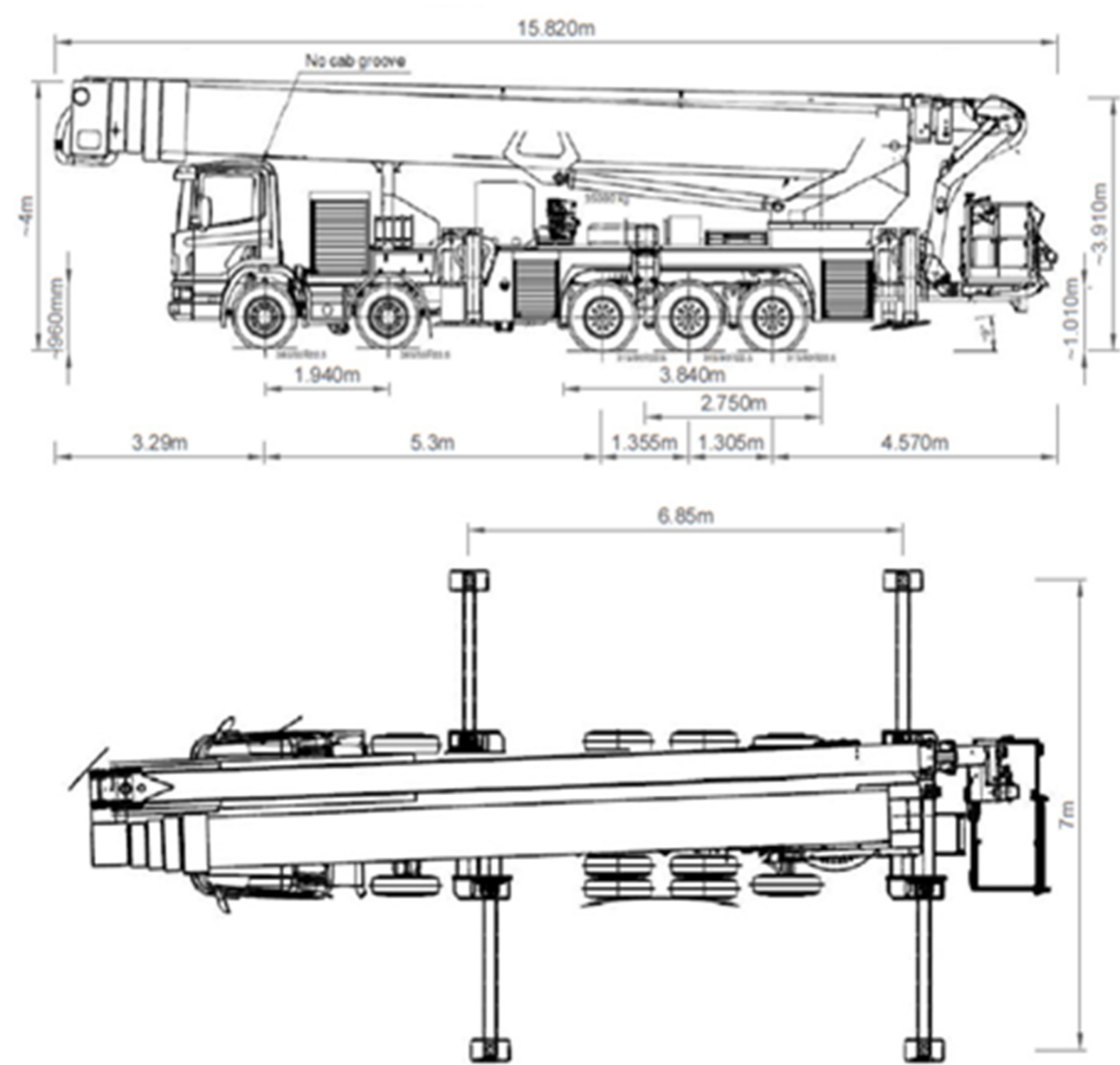
Diagram 4.2.4d.(1) – 3: HL 90 Firefighting Appliances – Wheels & Jacks Layout
