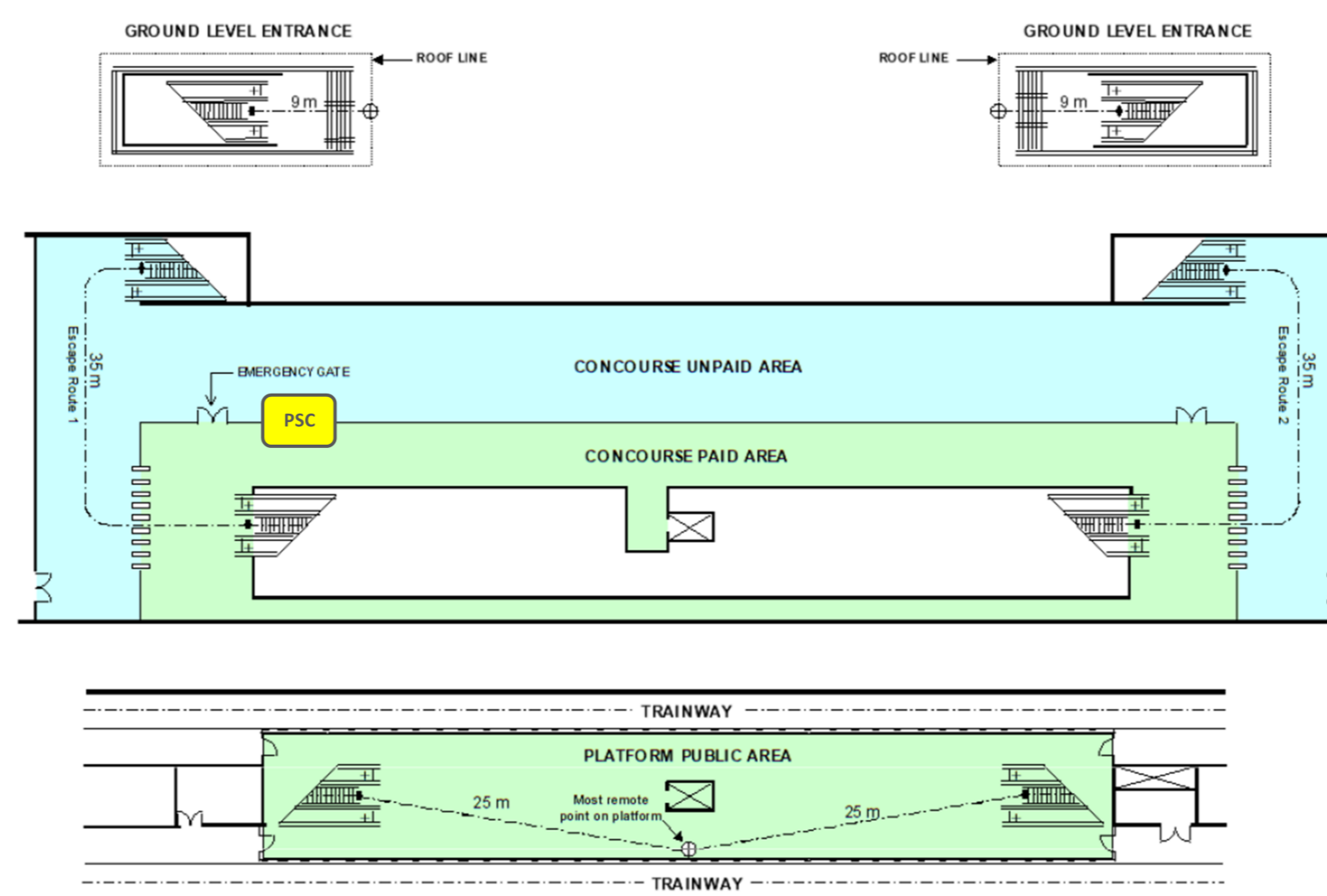
Figure A-2.1: Centre Platform Station
