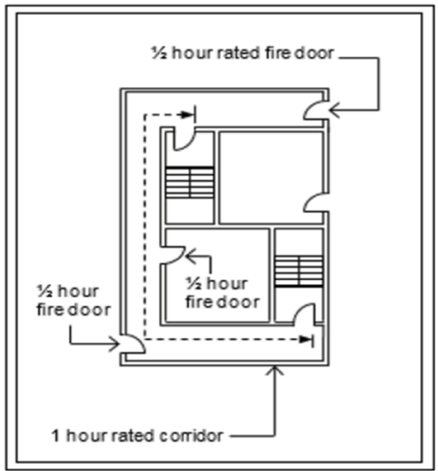
Remoteness of exits is measured along the 1-hr rated corridor with 1/2 hr fire doors
