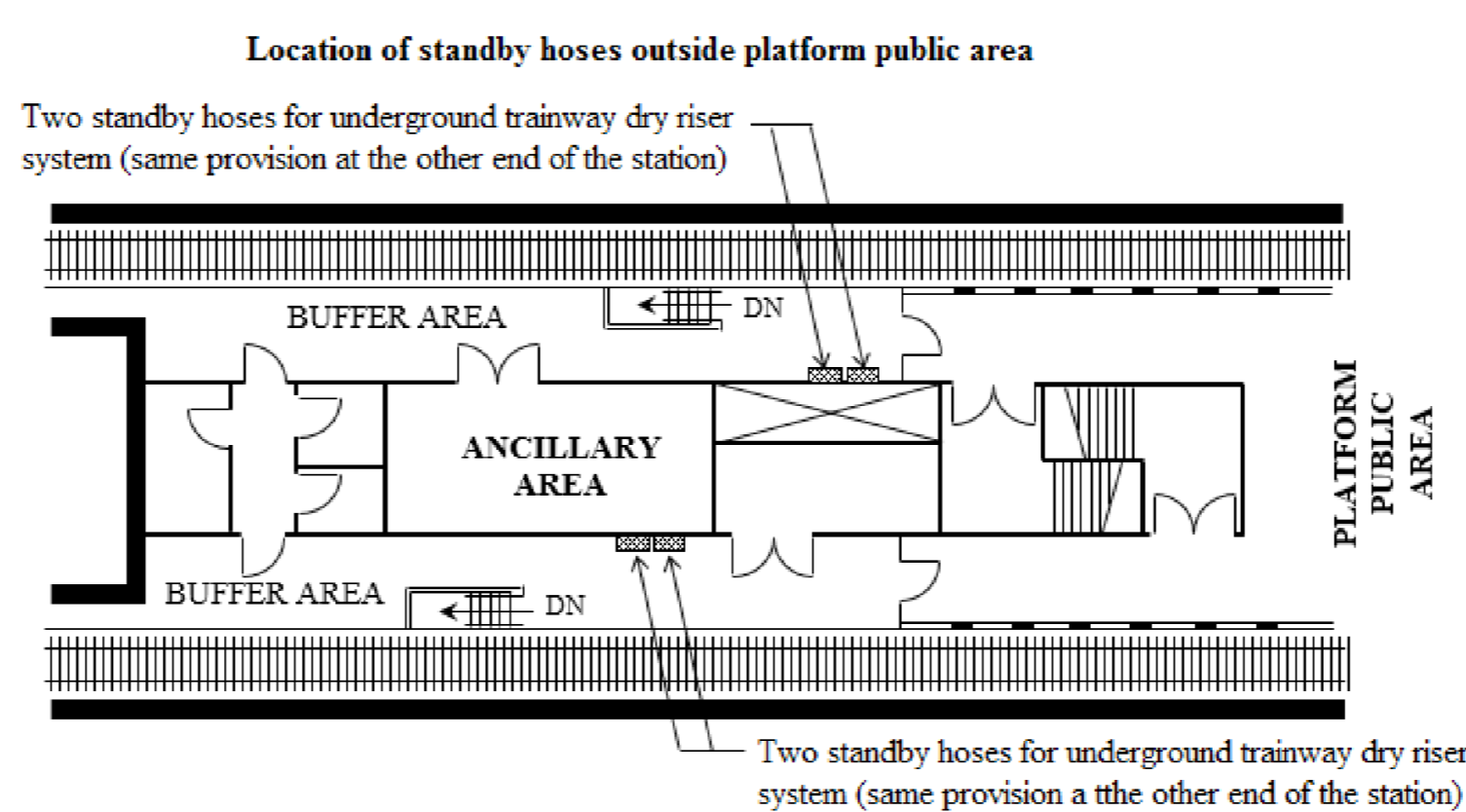
Diagram 9.3.9a(9)(a): Location of Standby Hoses Outside Platform Public Area
