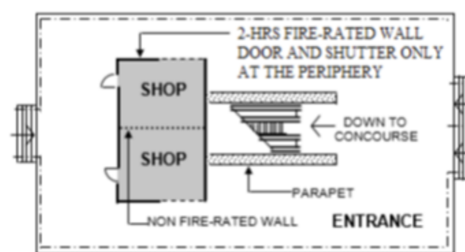
Diagram 3.2.4c.: Compartmentation of Commercial Spaces
