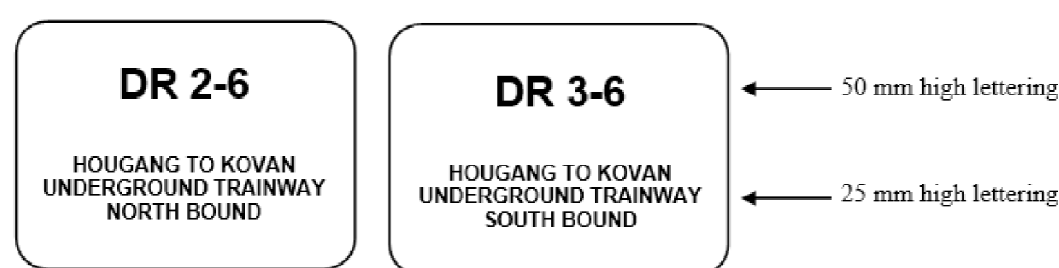
Diagram 9.3.9a(8): Numbering and Labelling of Breaching Inlets for Underground or Enclosed Trainway Dry Rising Mains
