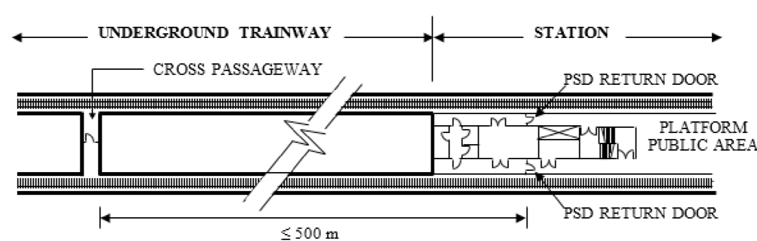
Diagram 9.3.3a: Location of First Cross-passageway in Underground Trainways
