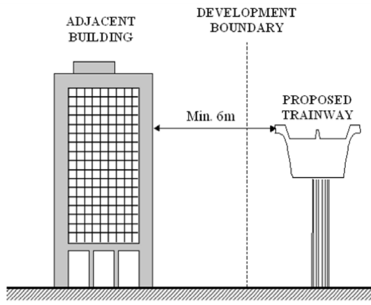
Diagram 9.4.2b: Separation Distance – Proposed Trainway Outside Development Boundary
