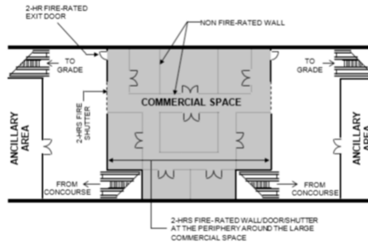
Compartmentation of commercial spaces at the ground level of station entrance
