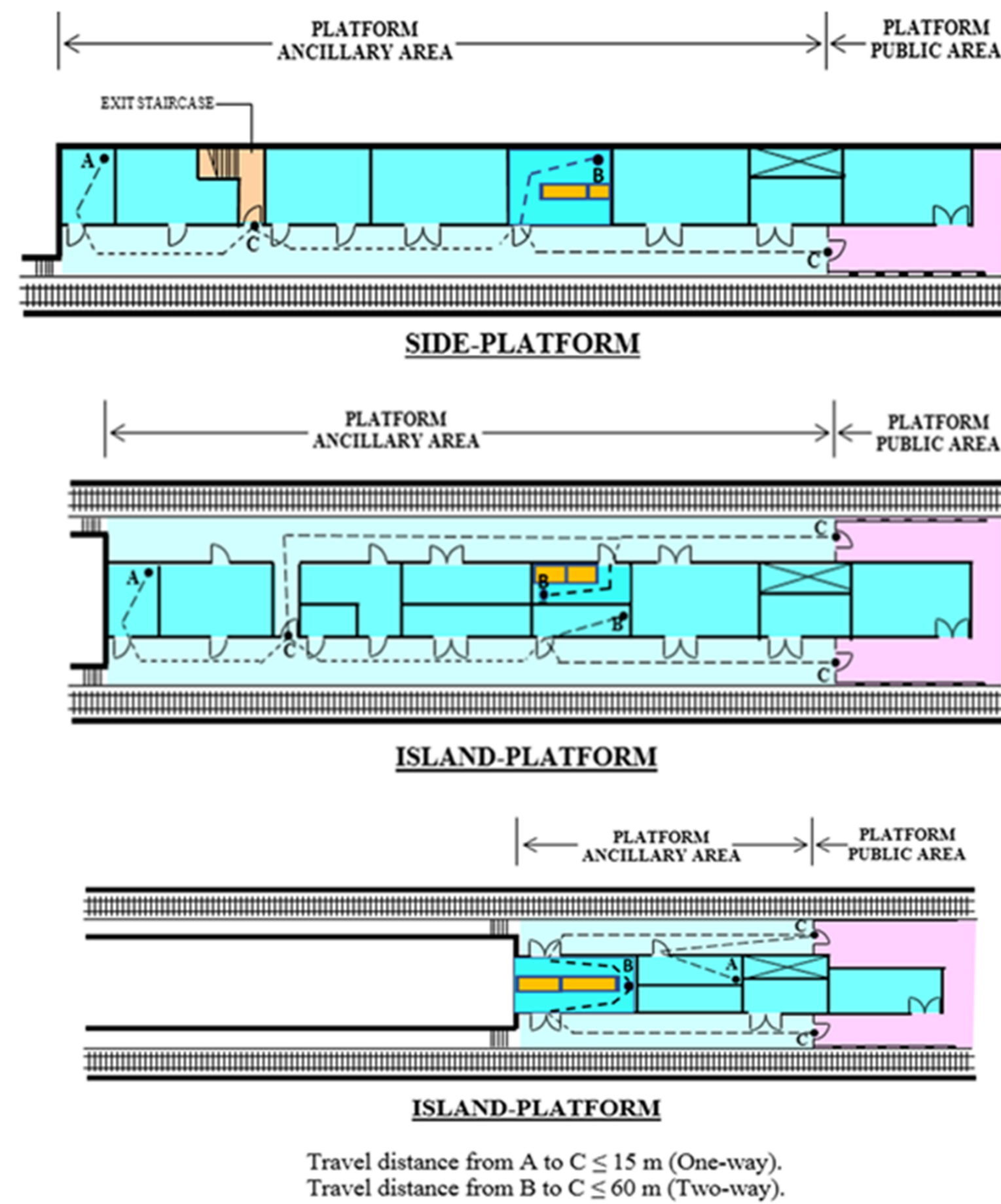
Diagram: 2.2.4d. island Platform
