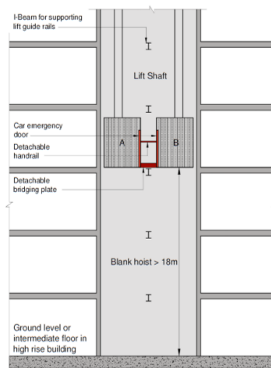
Diagram 6.6.9d(1): Car Emergency Doors for Lift-to-lift Rescue
