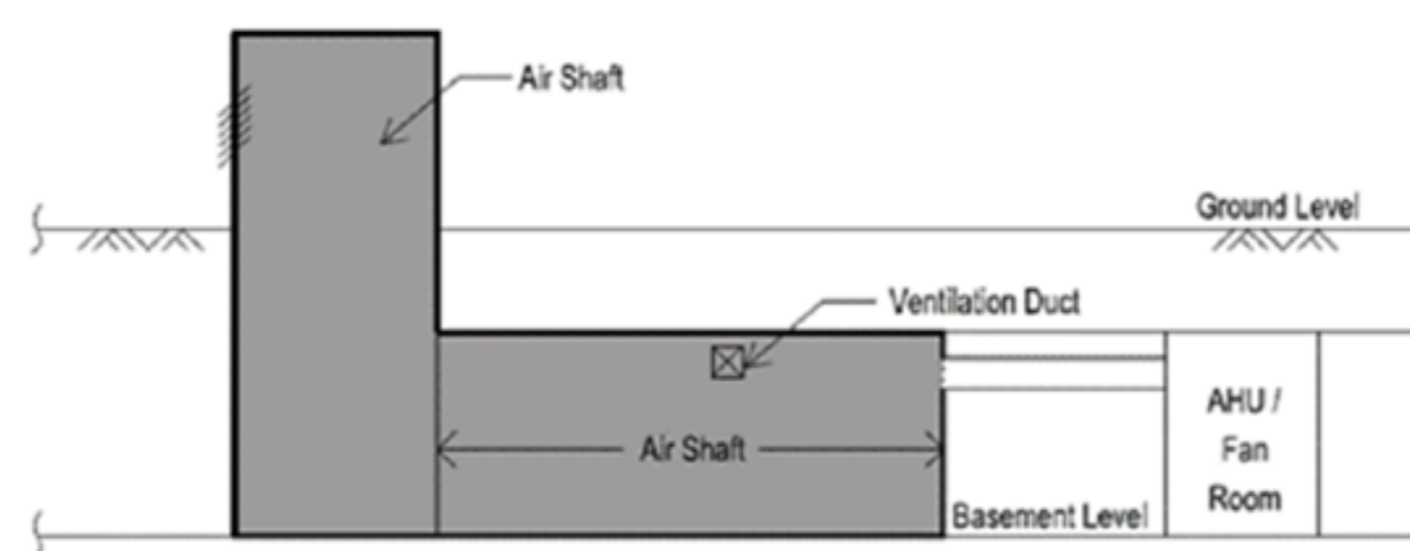
Diagram 7.1.16 - 2: Air Shaft Section A-A
