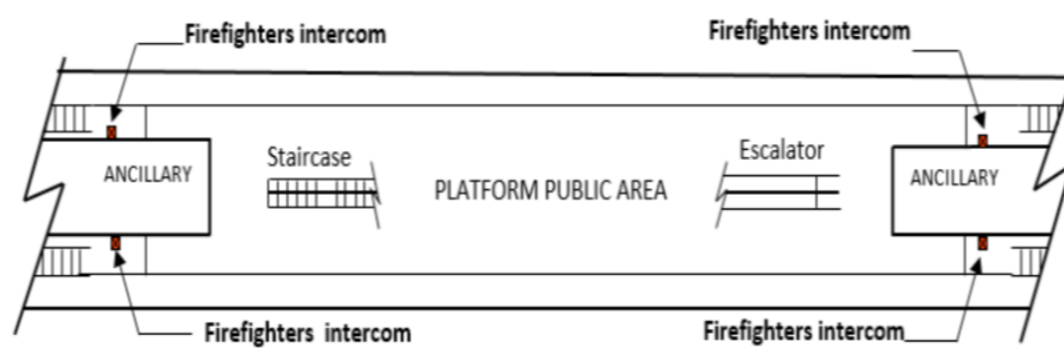
Diagram 8.2.8: Locations of Firefighters' Intercom at Platform Level
