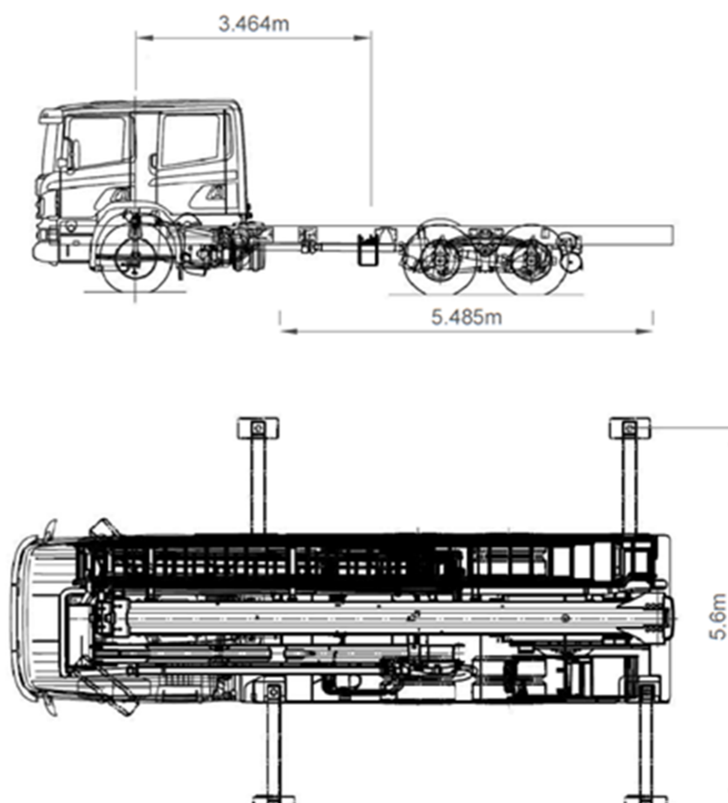
Diagram 4.2.4d.(1) – 1: CPL 34 Firefighting Appliances – Wheels & Jacks Layout
