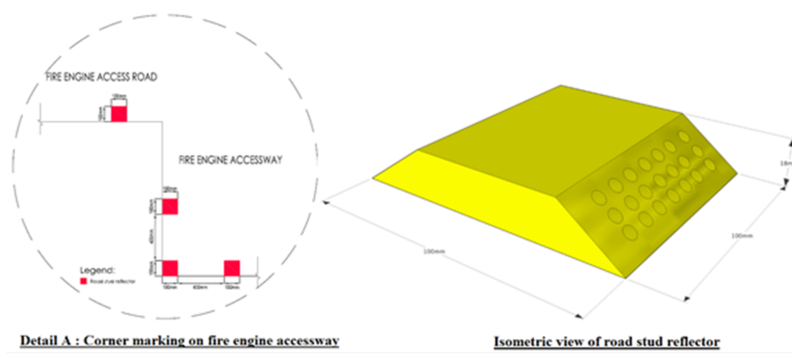
Diagram 4.2.4j(2): Markings for Fire Engine Accessway/ Fire Engine Access Road
