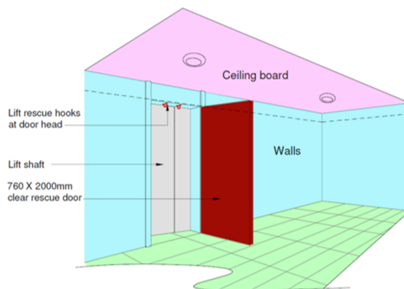
Diagram 6.6.9c(2): Landing Emergency Door
