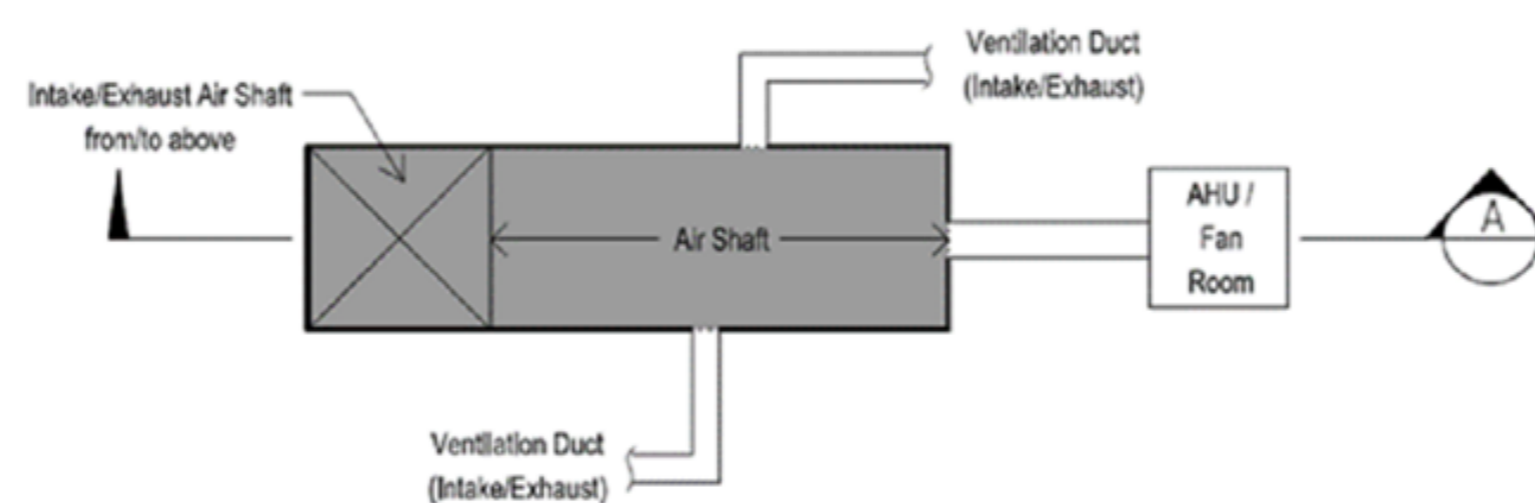
Diagram 7.1.16 - 1: Air Shaft Plan Layout
