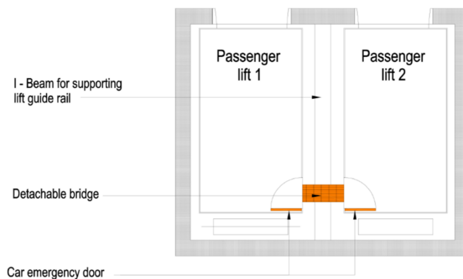
Diagram 6.6.9d(2): Car Emergency Doors – Deployed of Bridging Plate
