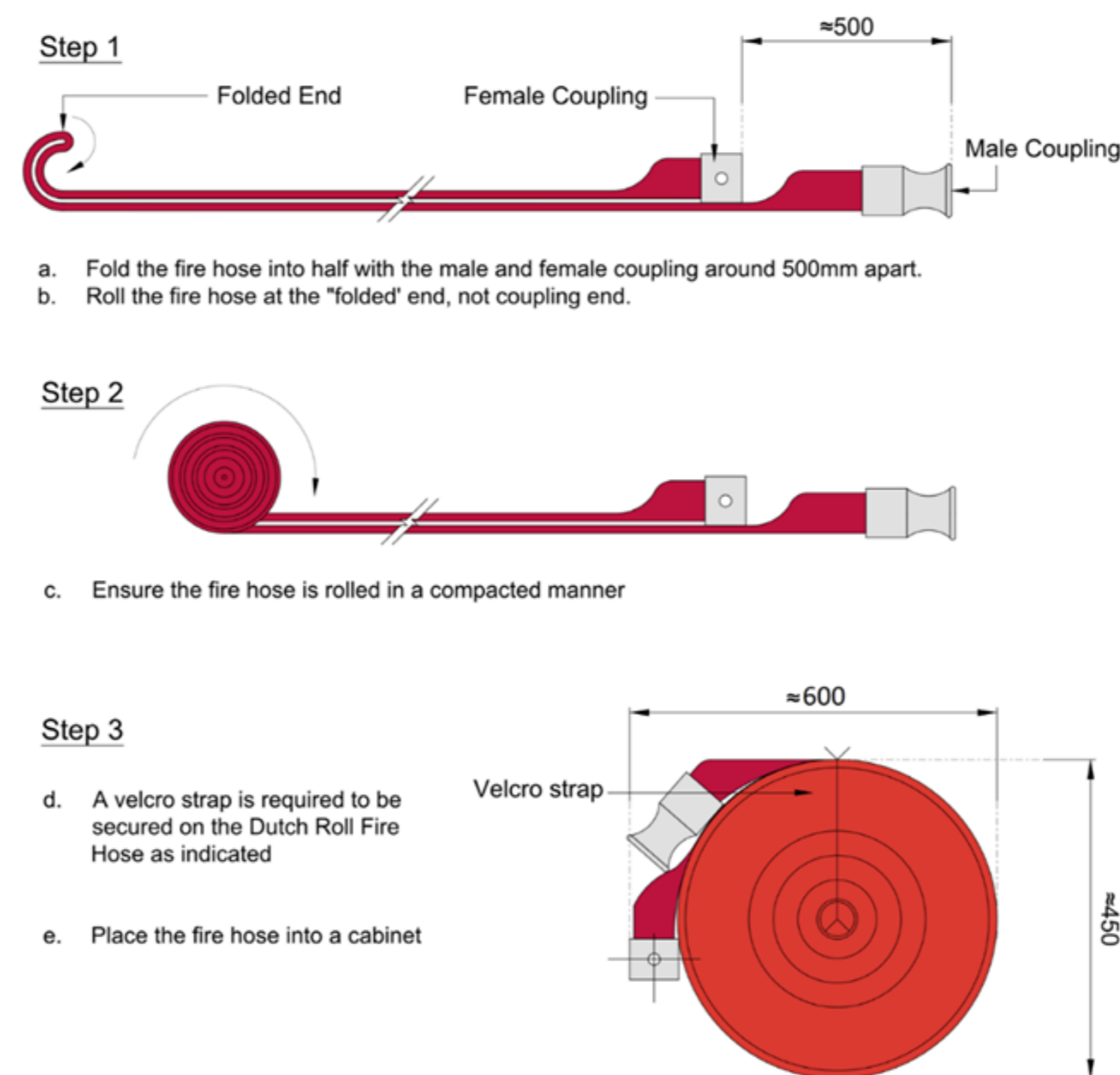
Diagram 6.2.4c.(9): Dutch Roll Folding Method
