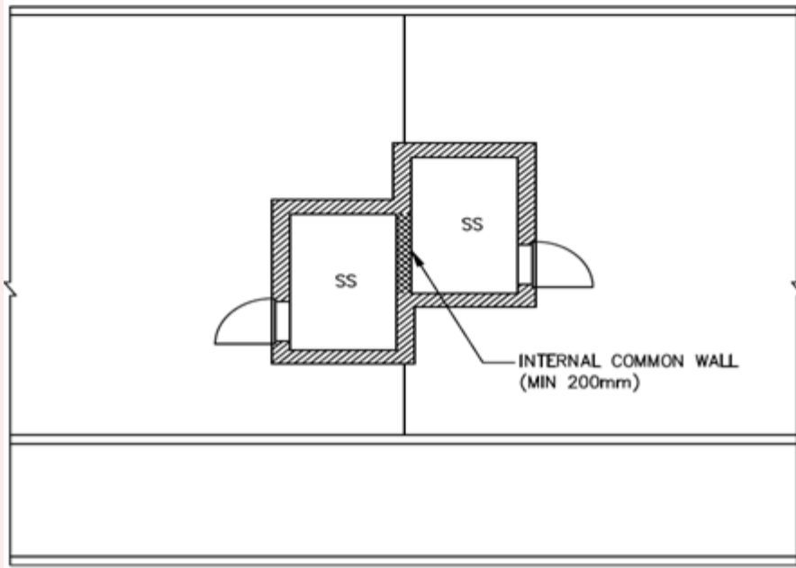
ALTERNATIVE 2
