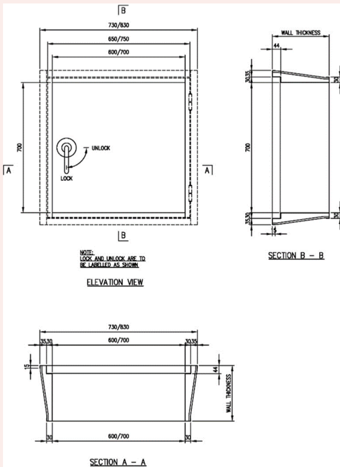
FIGURE 2.12.7(a): MINIMUM DIMENSION OF VERTICAL BLAST HATCH
