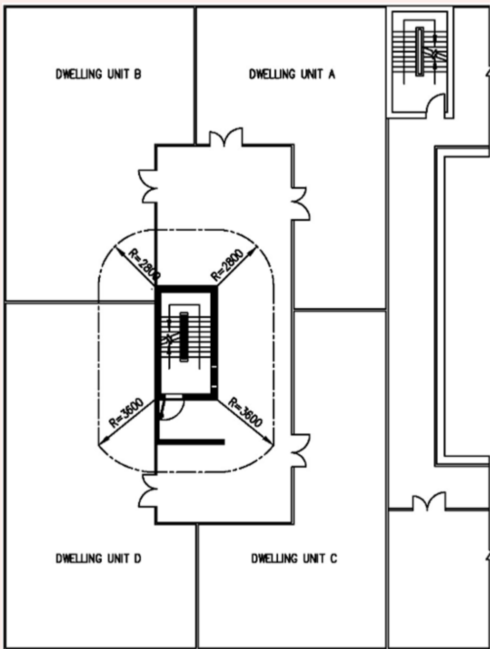
FIGURE 2.4.3(b): REQUIREMENT ON SETBACK DISTANCE OF SS WALLS (WITHOUT DOWN-HANG BEAM) (FOR 3500MM < STOREY HEIGHT | 4000MM)
