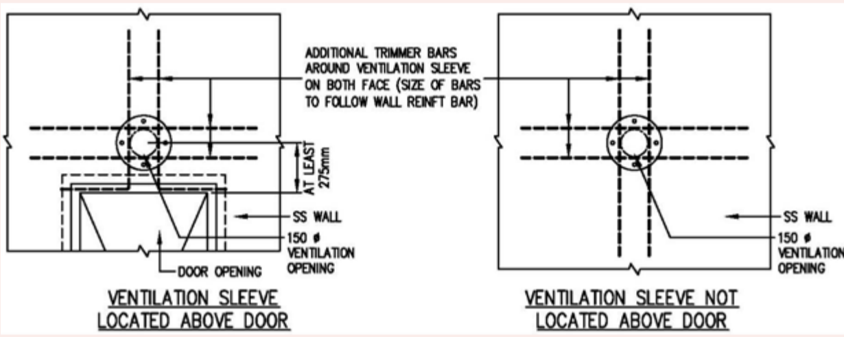
FIGURE 3.5.4(f): TYPICAL DETAILS OF TRIMMER BARS FOR VENTILATION SLEEVE
