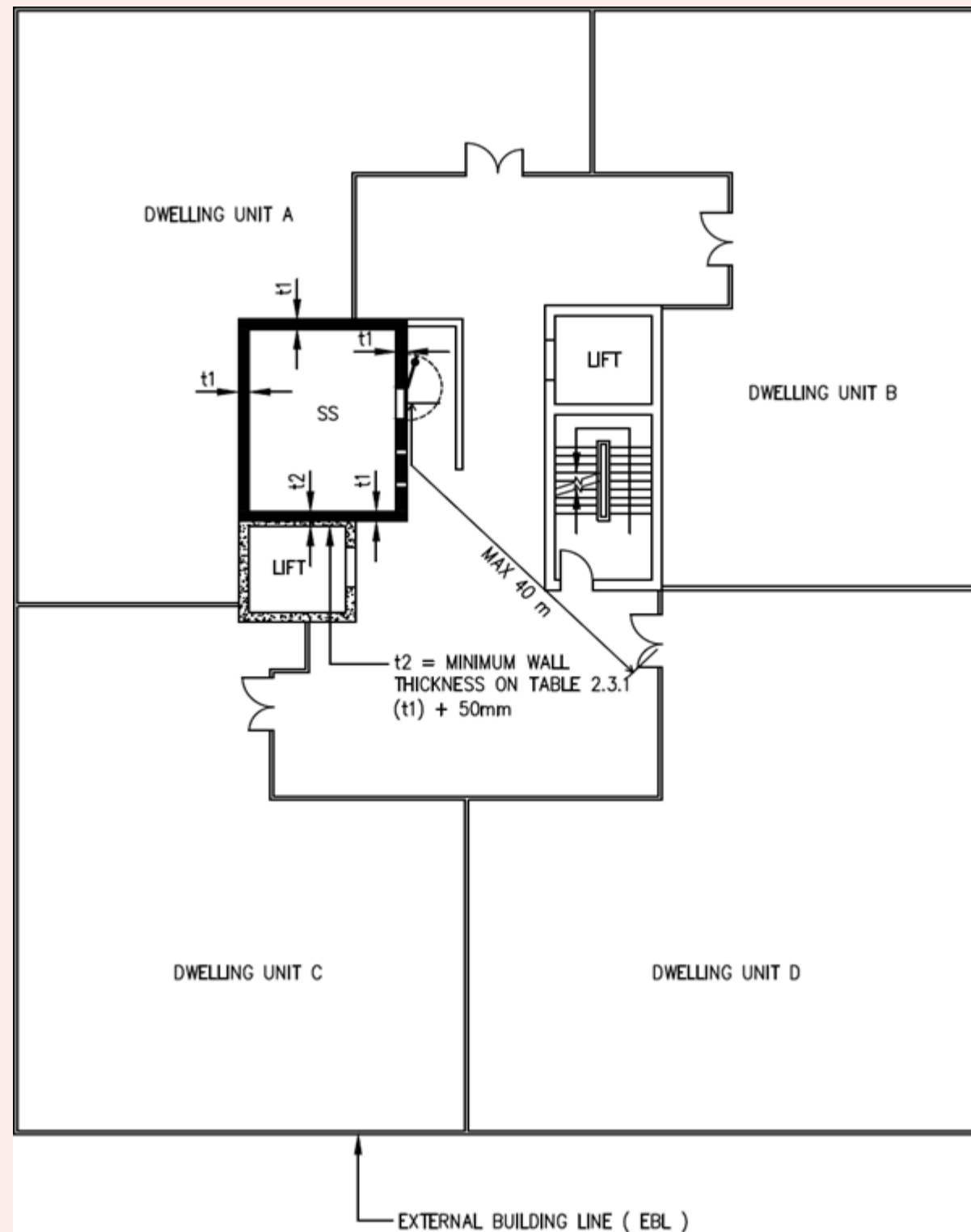
FIGURE 2.4.1: SS LOCATED NEXT TO LIFT SHAFT
