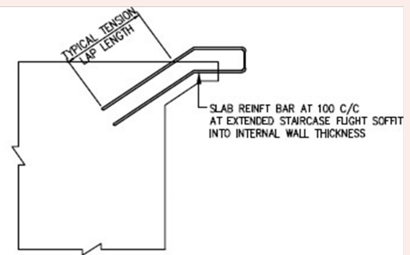
FIGURE 3.5.6.2(b)(v): SECTION K2-K2 (S/C SS COMPONENT 'B') AT INTERNAL WALL LOCATION
