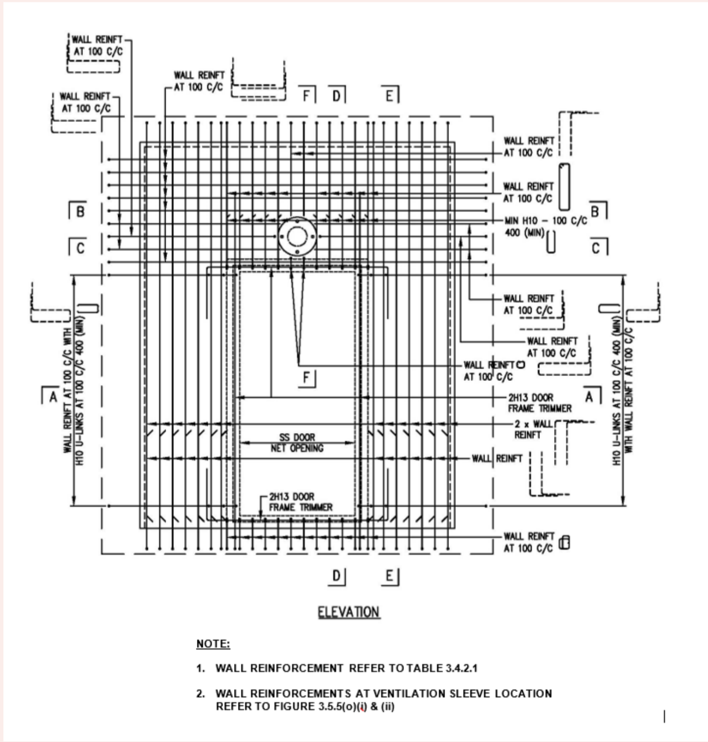
FIGURE 3.5.5(i): DETAILS OF PRECAST SS DOOR FRAME PANEL (TYPE 3)
