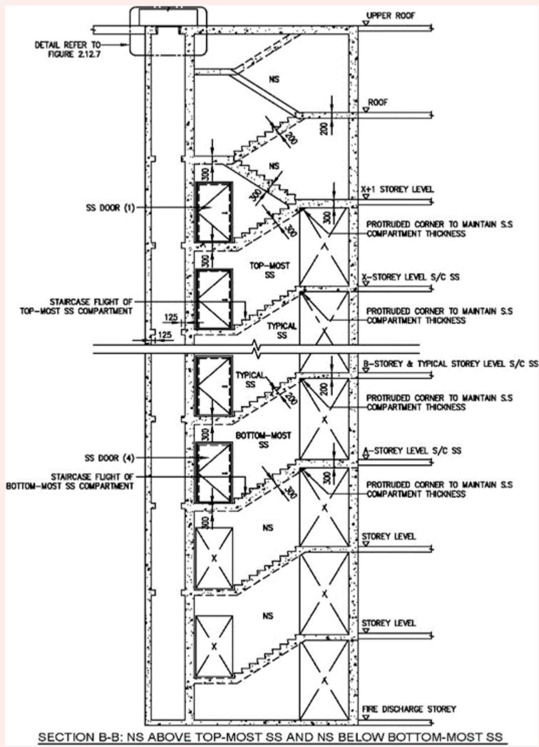
FIGURE 2.12.2(d): SS WITH NS ABOVE TOP-MOST SS COMPARTMENT, INTERMEDIATE SS COMPARTMENT AND SS WITH NS BELOW BOTTOM-MOST SS COMPARTMENT
