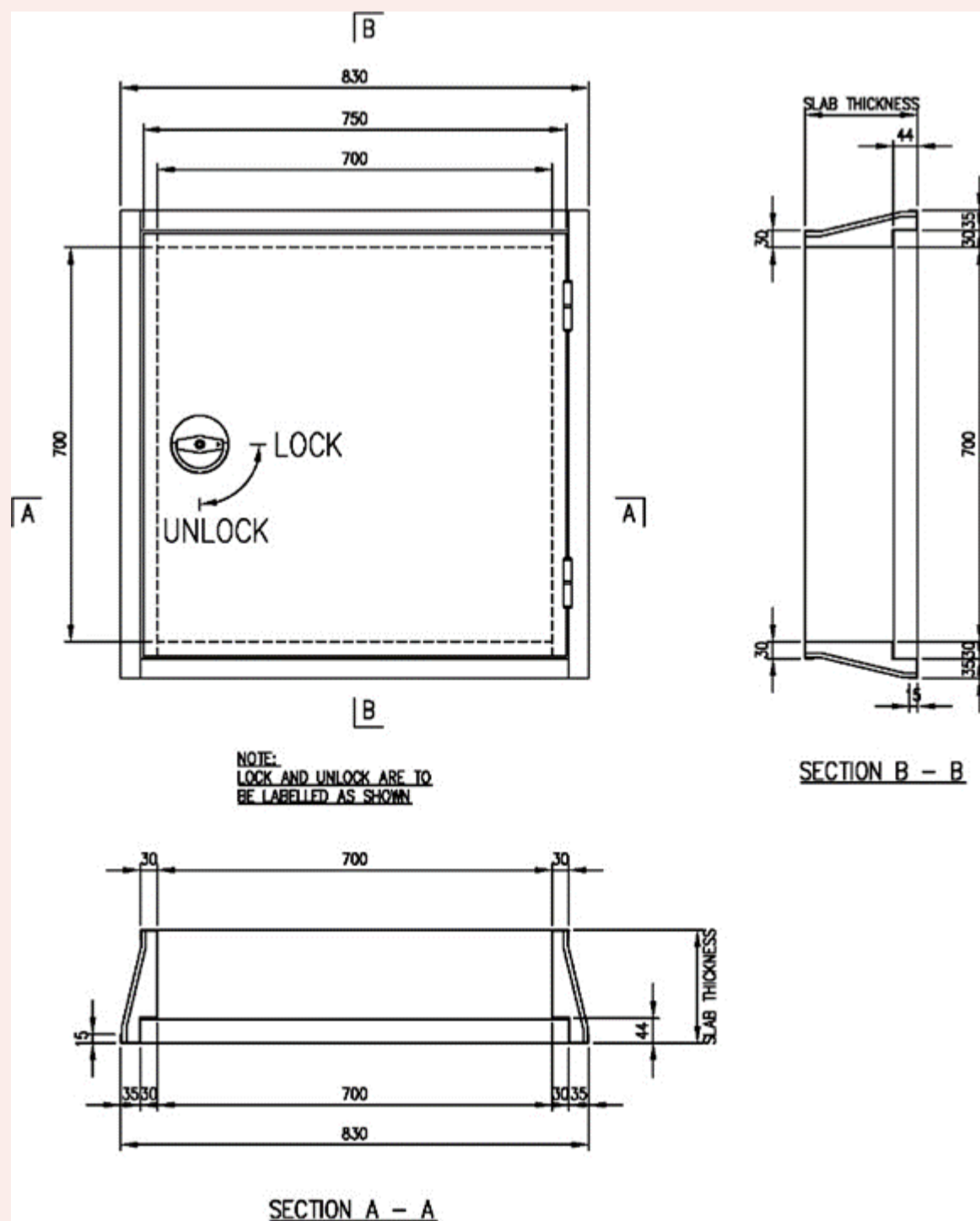
FIGURE 2.11.1(c): MINIMUM DIMENSIONS OF RESCUE HATCH
