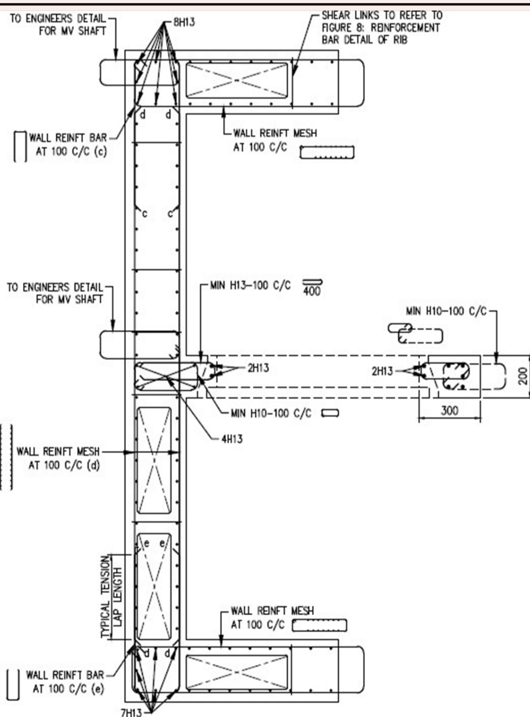
FIGURE 3.5.6.2(a)(iii), FIGURE 3.5.6.2(a)(iv) && FIGURE 3.5.6.2(a)(v)
