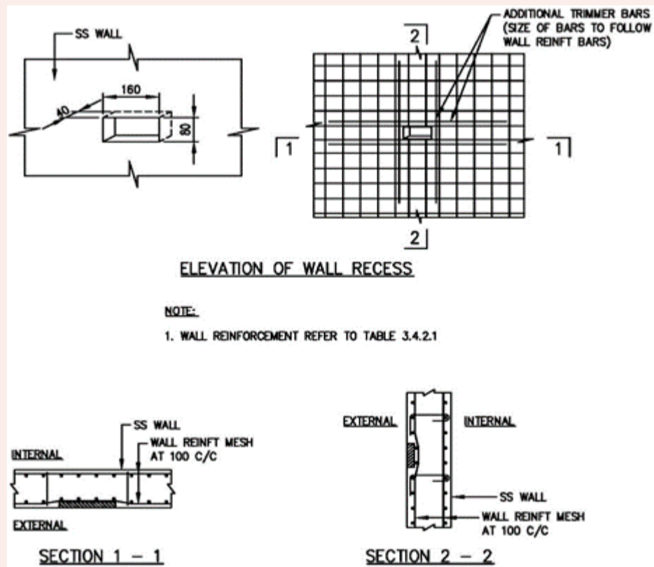
FIGURE 3.5.4(g): TYPICAL DETAILS OF REINFORCEMENT BARS AT WALL RECESS
