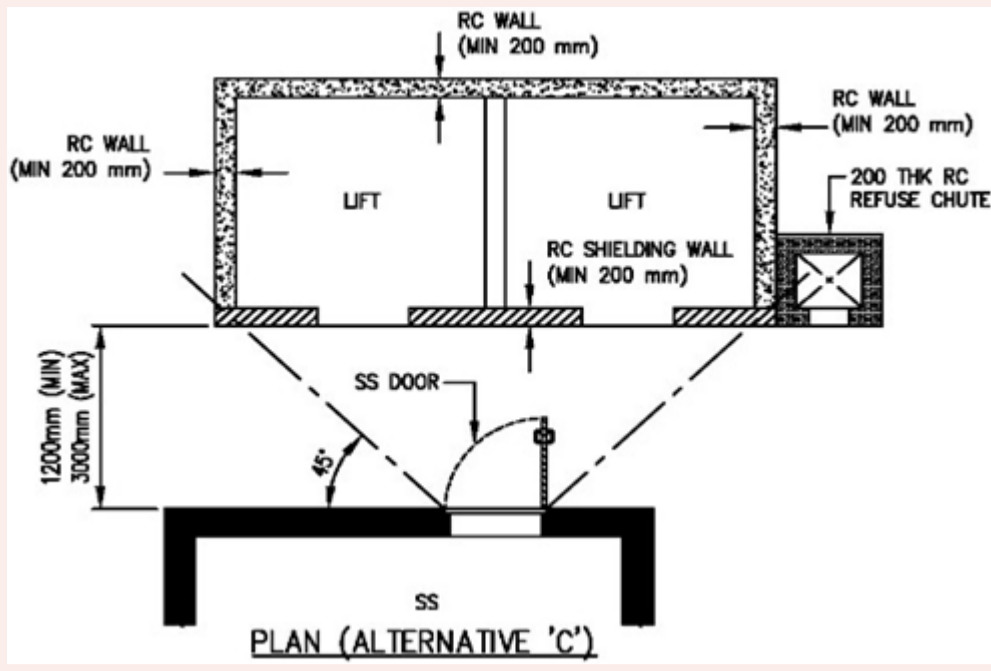
FIGURE 2.5.4(d): SHIELDING FOR SS DOOR
