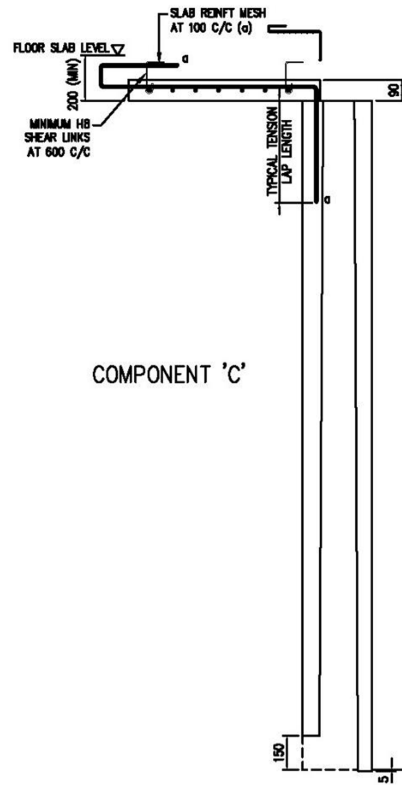
FIGURE 3.5.6.2(c)(iv): SECTION T-T (S/C SS COMPONENT 'C')
