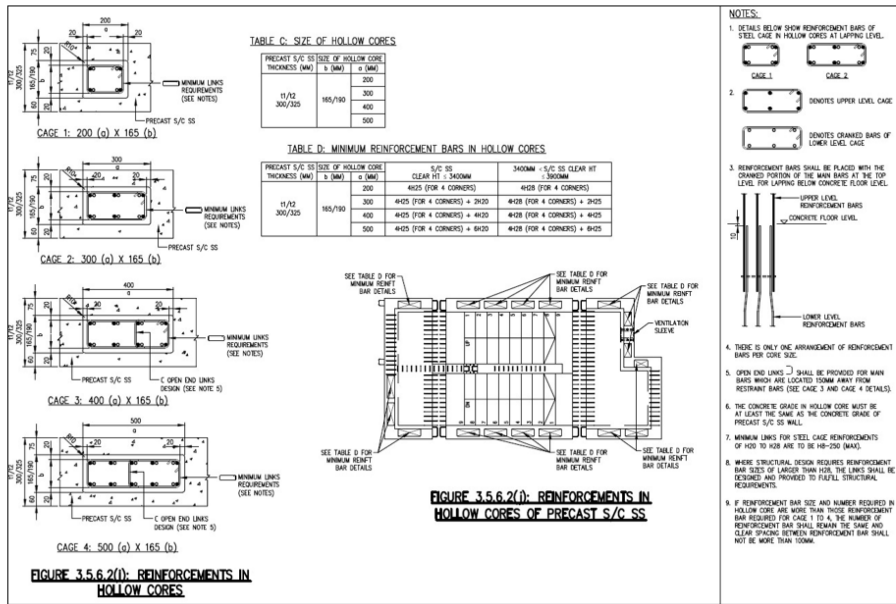
FIGURE 3.5.6.2(i) and 3.5.6.2(j)
