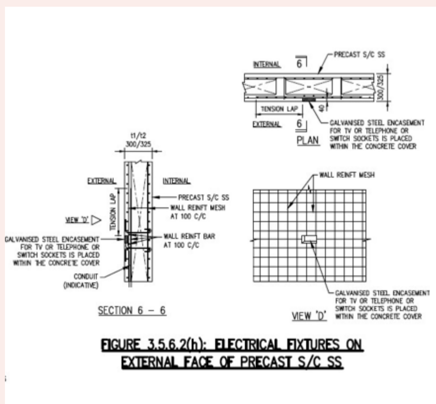
FIGURE 3.5.6.2(h)
