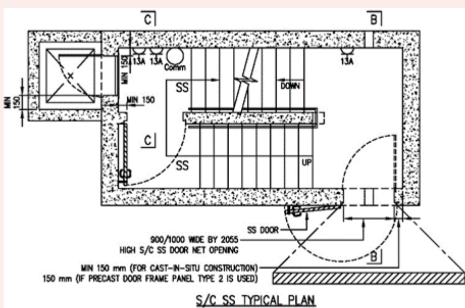
FIGURE 2.5.3(c): CONCRETE WALL SEGMENT AT S/C SS DOORS AND BLAST HATCH
