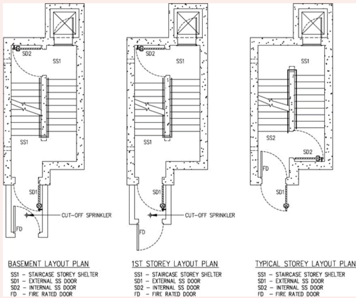
FIGURE 2.12.8: PROVISION OF CUT-OFF SPRINKLER IN S/C SS
