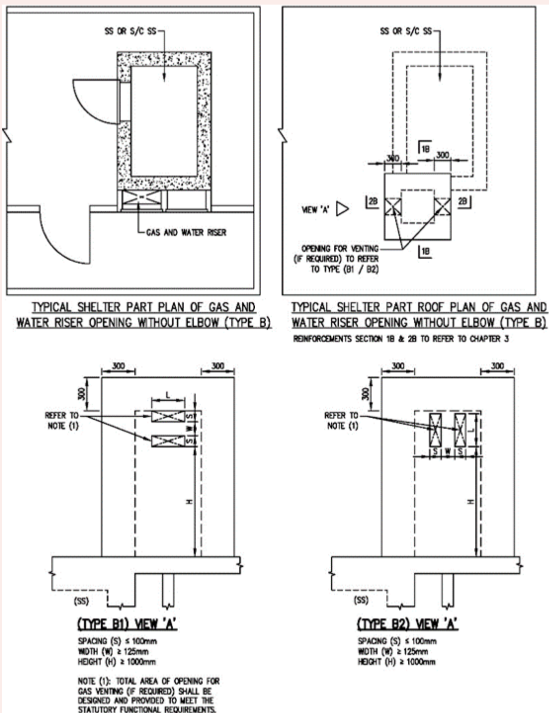
FIGURE 2.4.5(f): PROTECTION REQUIREMENT AT ROOF LEVEL FOR PROVISION OF GAS AND WATER RISER LOCATED WITHIN SETBACK DISTANCE ENVELOP (TYPE B)
