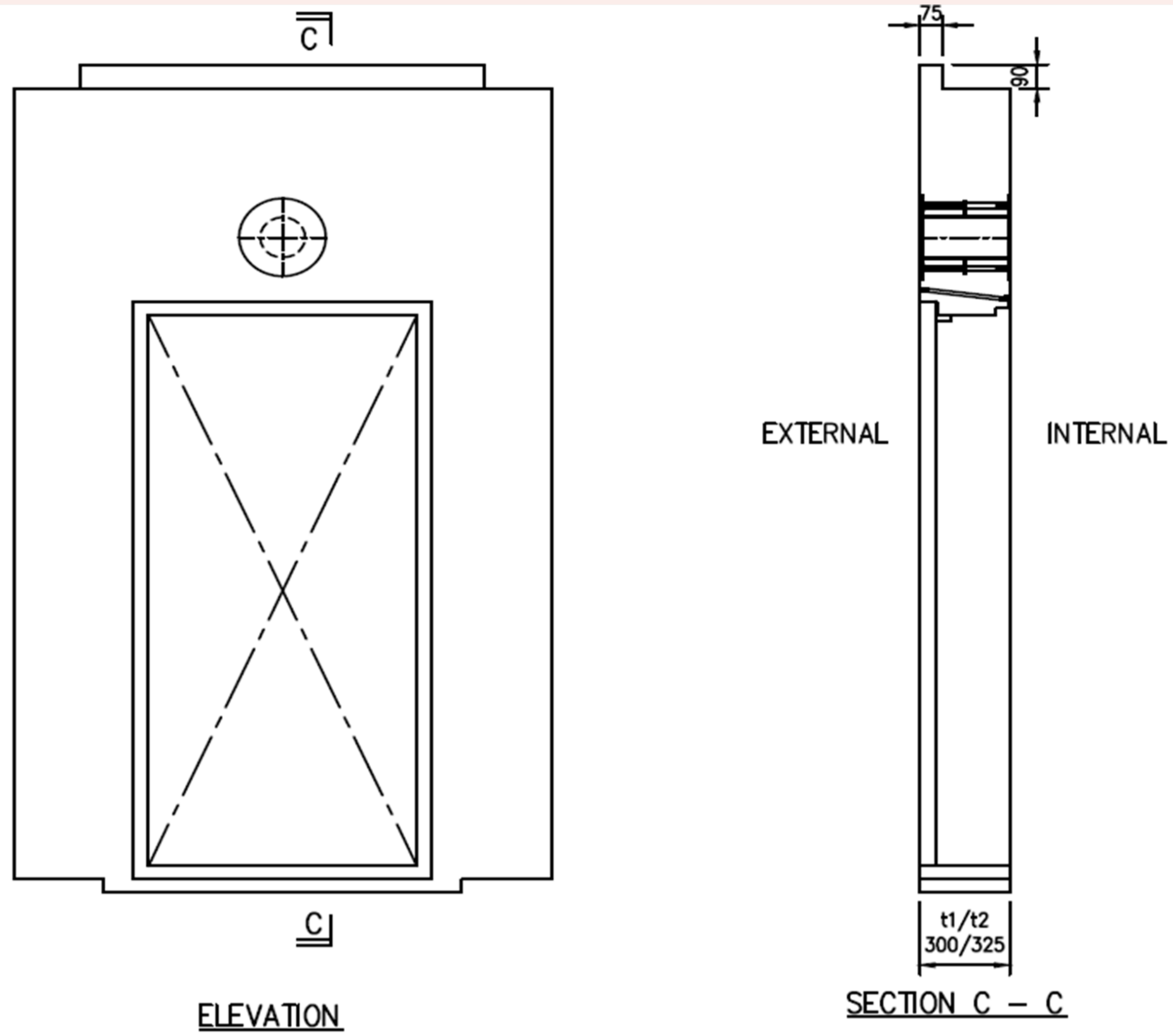
FIGURE 3.5.6.1(c): BLAST DOOR AND VENTILATION SLEEVE
