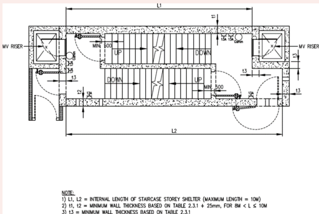
FIGURE 2.2.1(b): TYPICAL LAYOUT OF S/C SS
