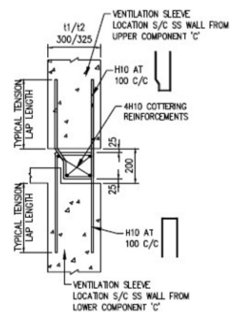
SECTION Y-Y OF DETAIL 'J'
