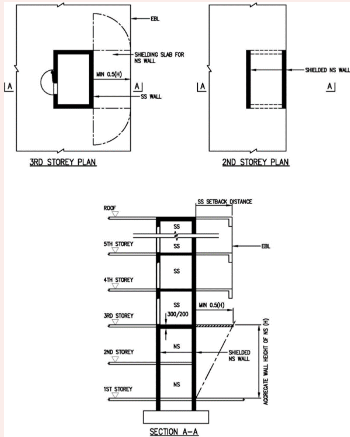
FIGURE 3.3.3: SHIELDED NS WALLS OF SS TOWER (2 OPPOSITE NS WALLS NOT APPLICABLE FOR S/C SS TOWER)
