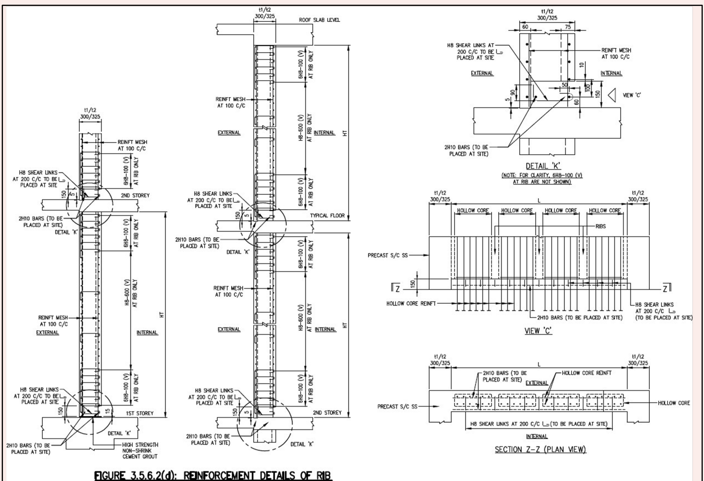
FIGURE 3.5.6.2(d): REINFORCEMENT DETAILS OF RIB
