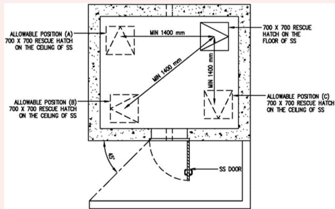
FIGURE 2.11.1(b): MINIMUM DISTANCE BETWEEN CENTRE LINES OF RESCUE HATCH
