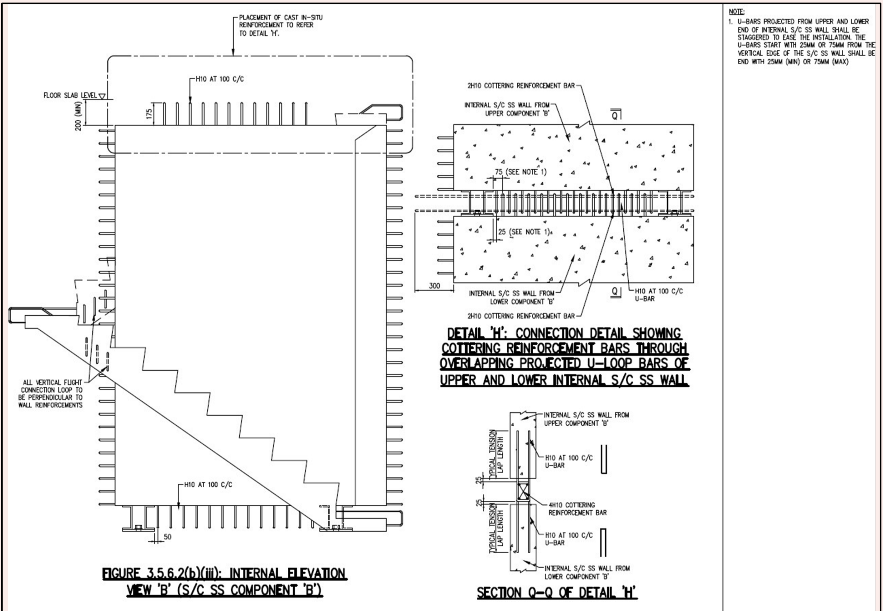
FIGURE 3.5.6.2(b)(iii)
