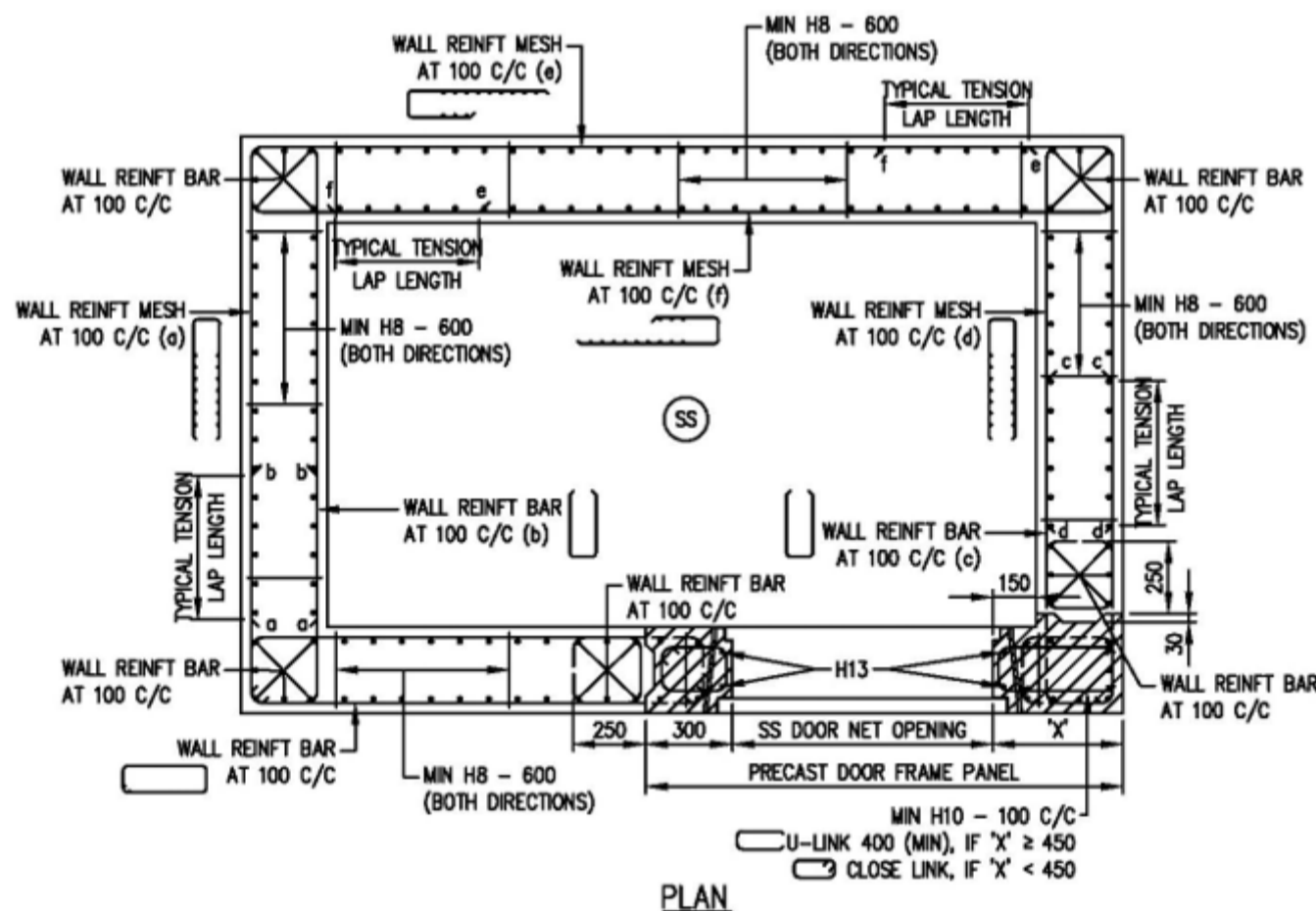
FIGURE 3.5.5(f): PLAN OF SS WALLS WITH PRECAST SS DOOR FRAME PANEL (TYPE 2)
