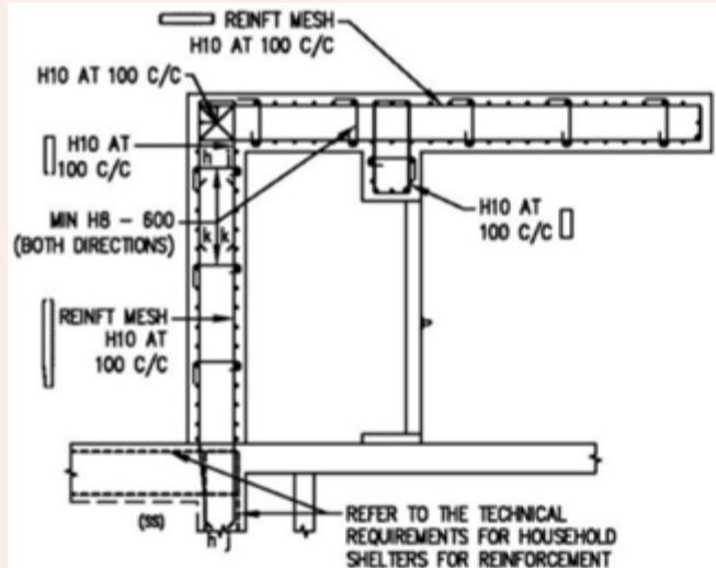
REINFORCEMENT DETAIL OF SECTION 1C-1C OF RC PROTECTION REQUIREMENT AT ROOF LEVEL FOR PROVISION OF ANY OTHER SERVICE RISER LOCATED WITHIN SETBACK DISTANCE ENVELOP
