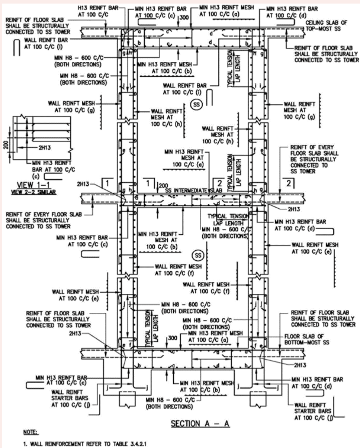
FIGURE 3.5.4(c): SECTIONAL DETAILS OF SS SLABS/WALLS
