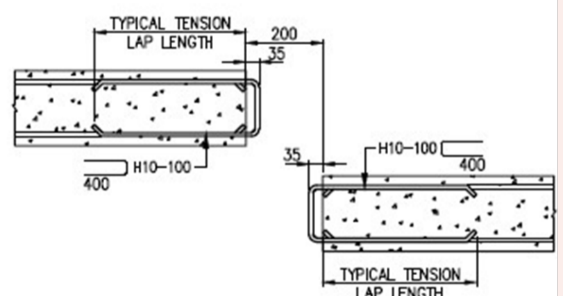
SECTION R-R: SECTION OF STAIRCASE FLIGHT CAST IN-SITU JOINT LOCATION
