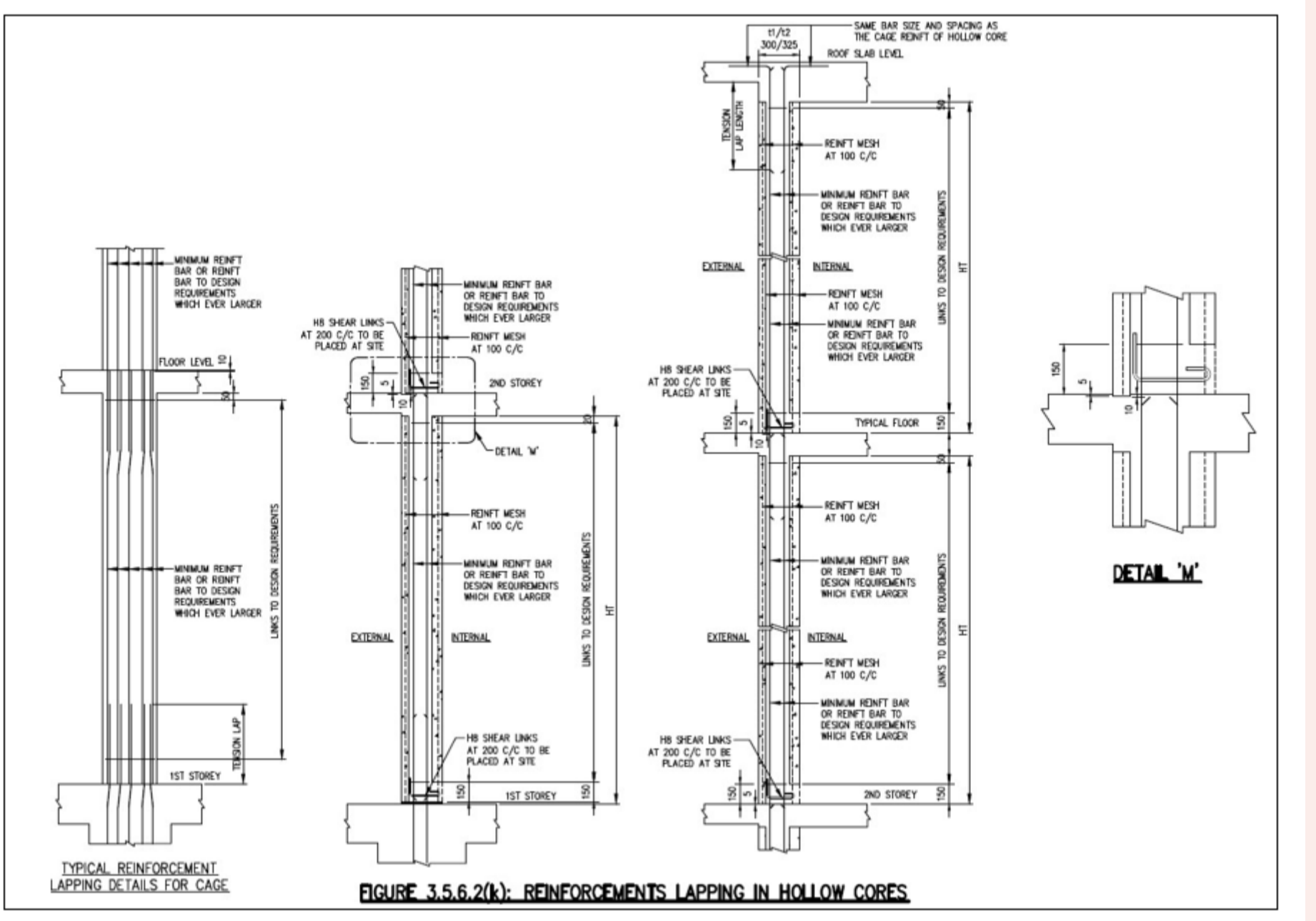
FIGURE 3.5.6.2(k)
