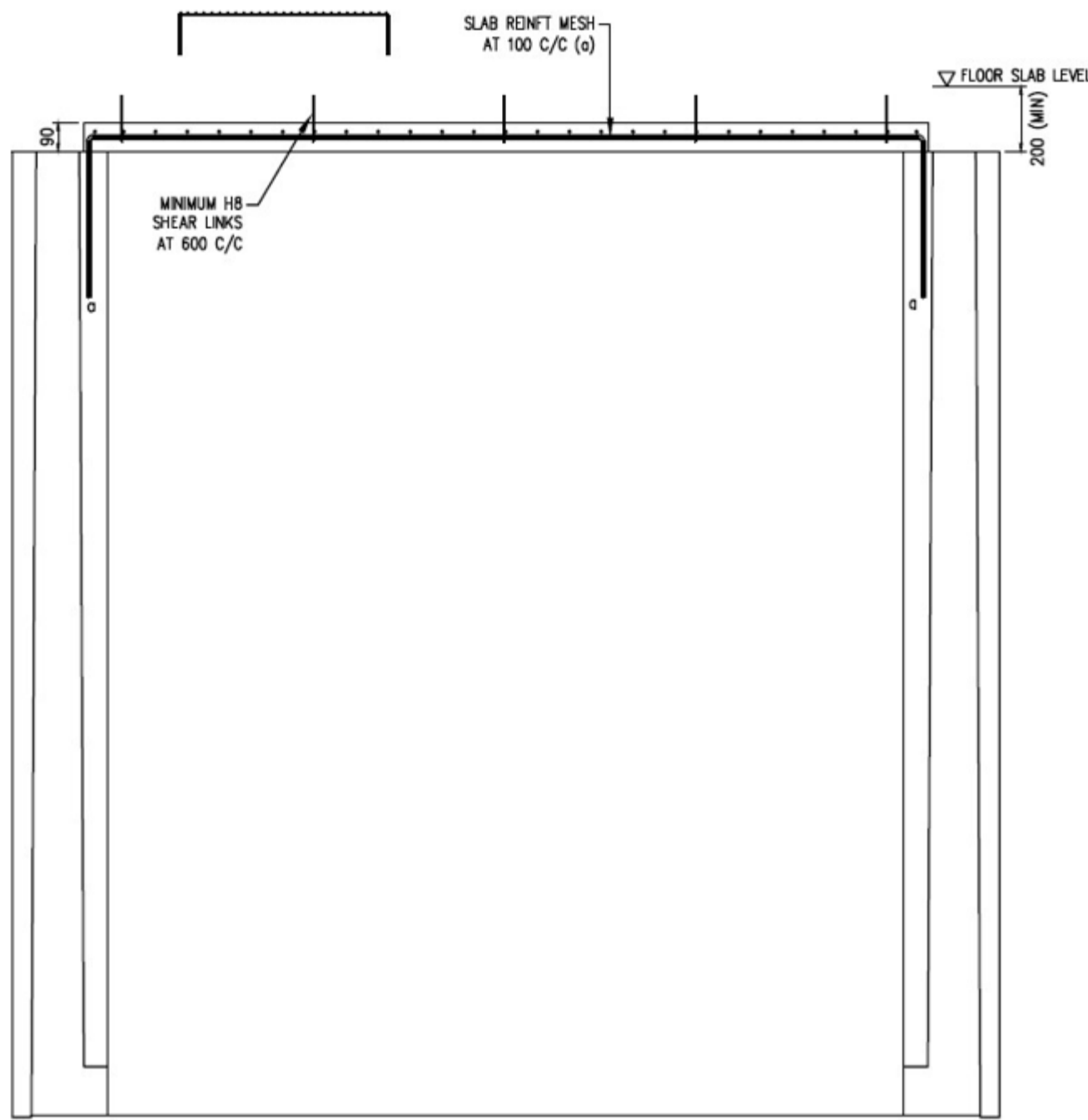
FIGURE 3.5.6.2(c)(vii): SECTION Y-V (S/C SS COMPONENT 'C')
