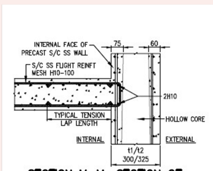
SECTION M-M: SECTION OF STAIRCASE FLIGHT AT HOLLOW CORE
