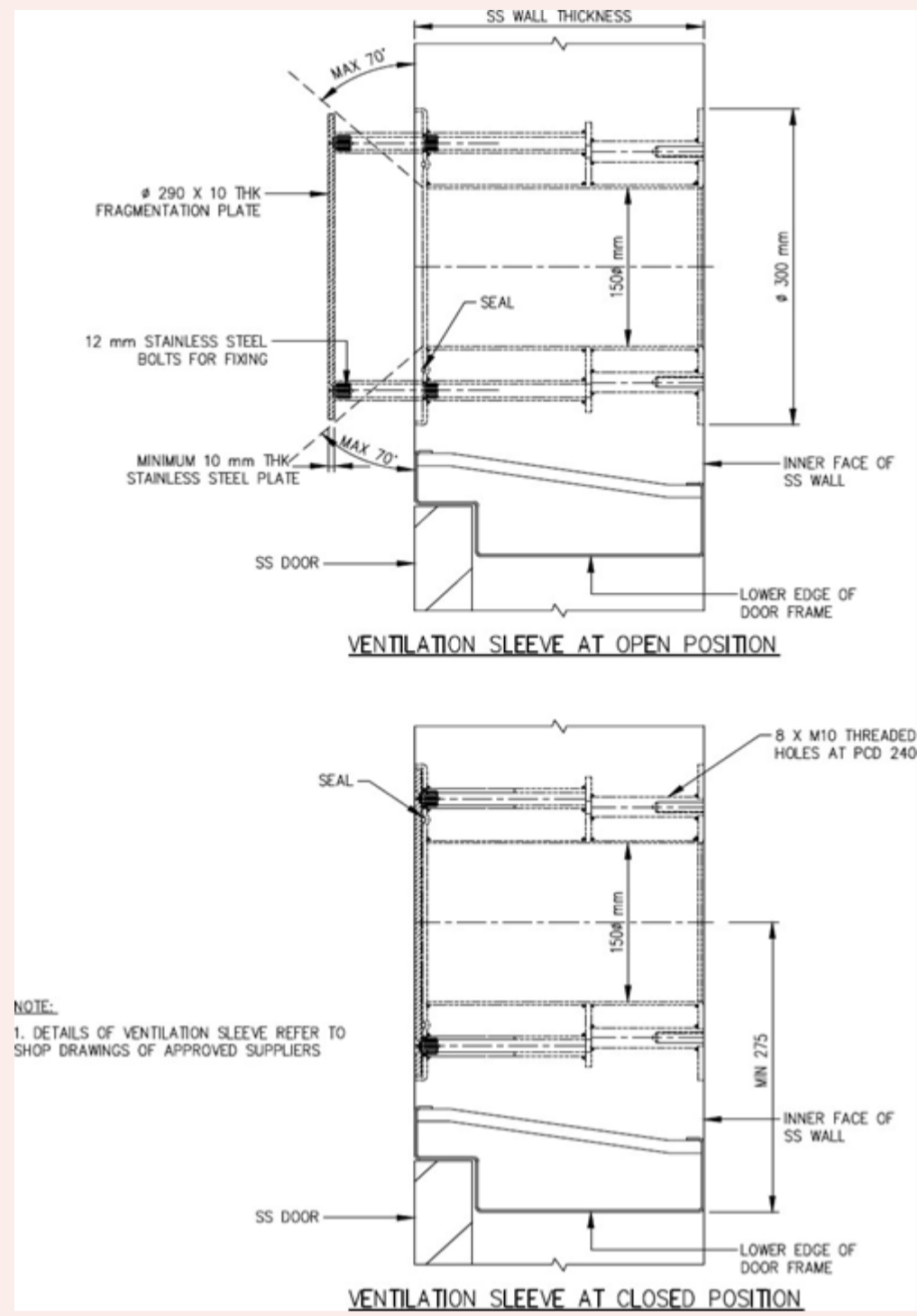
FIGURE 4.4: DETAILS OF VENTILATION SLEEVE AND FRAGMENTATION PLATE
