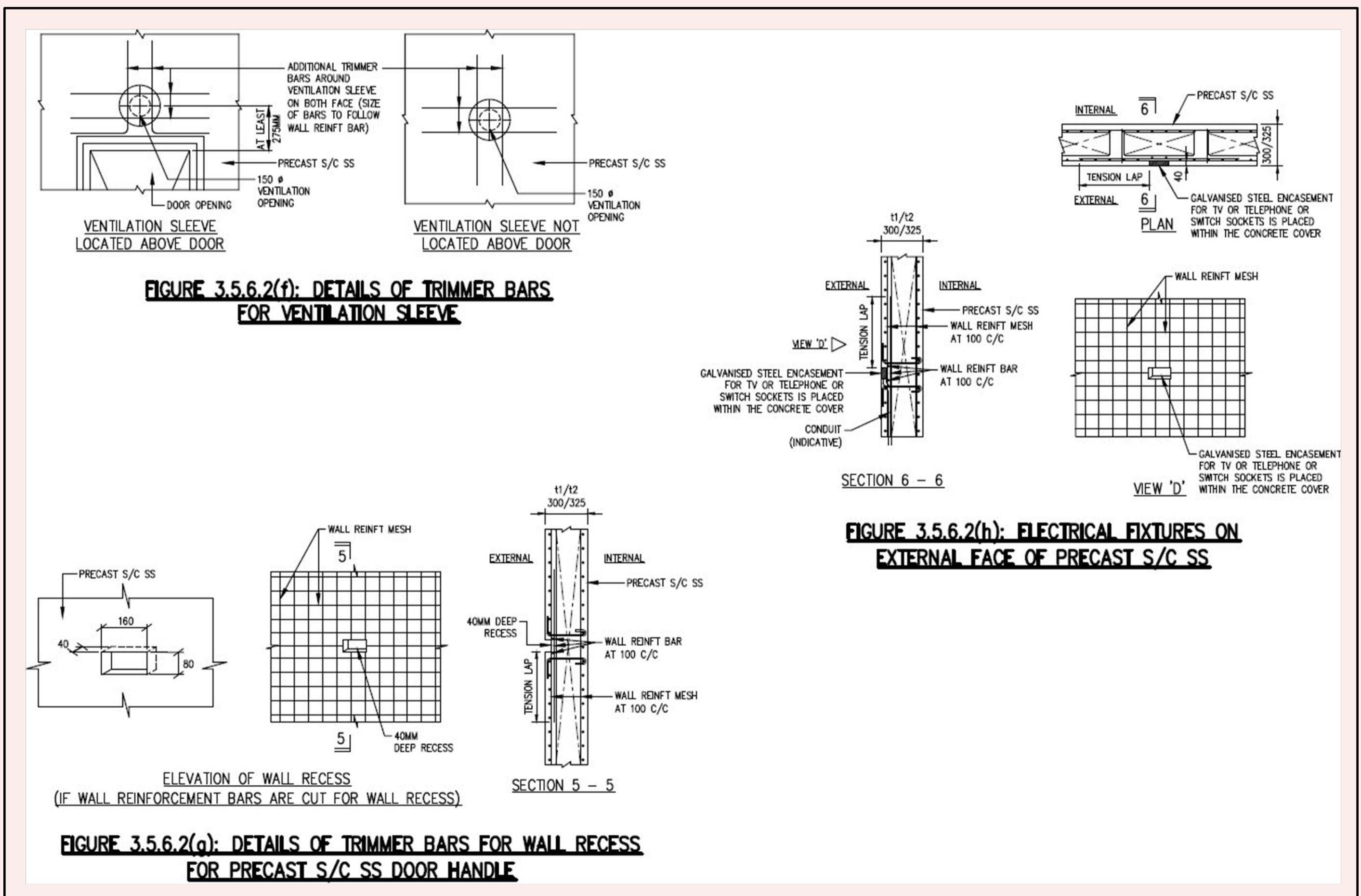
FIGURE 3.5.6.2(f), FIGURE 3.5.6.2(g) & FIGURE 3.5.6.2(h)
