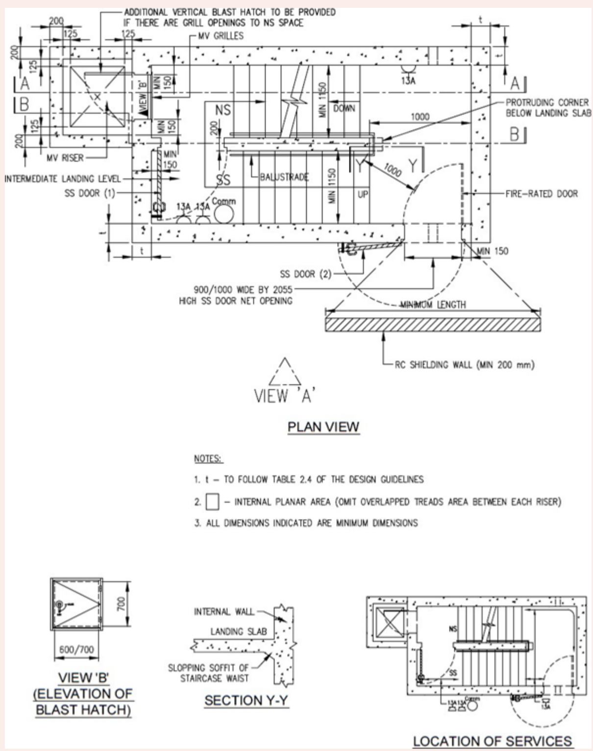
FIGURE 2.12.1(f): TYPICAL PLAN OF S/C SS COMPARTMENT
