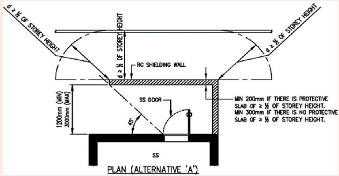
FIGURE 2.5.4(a): SHIELDING FOR SS DOOR
