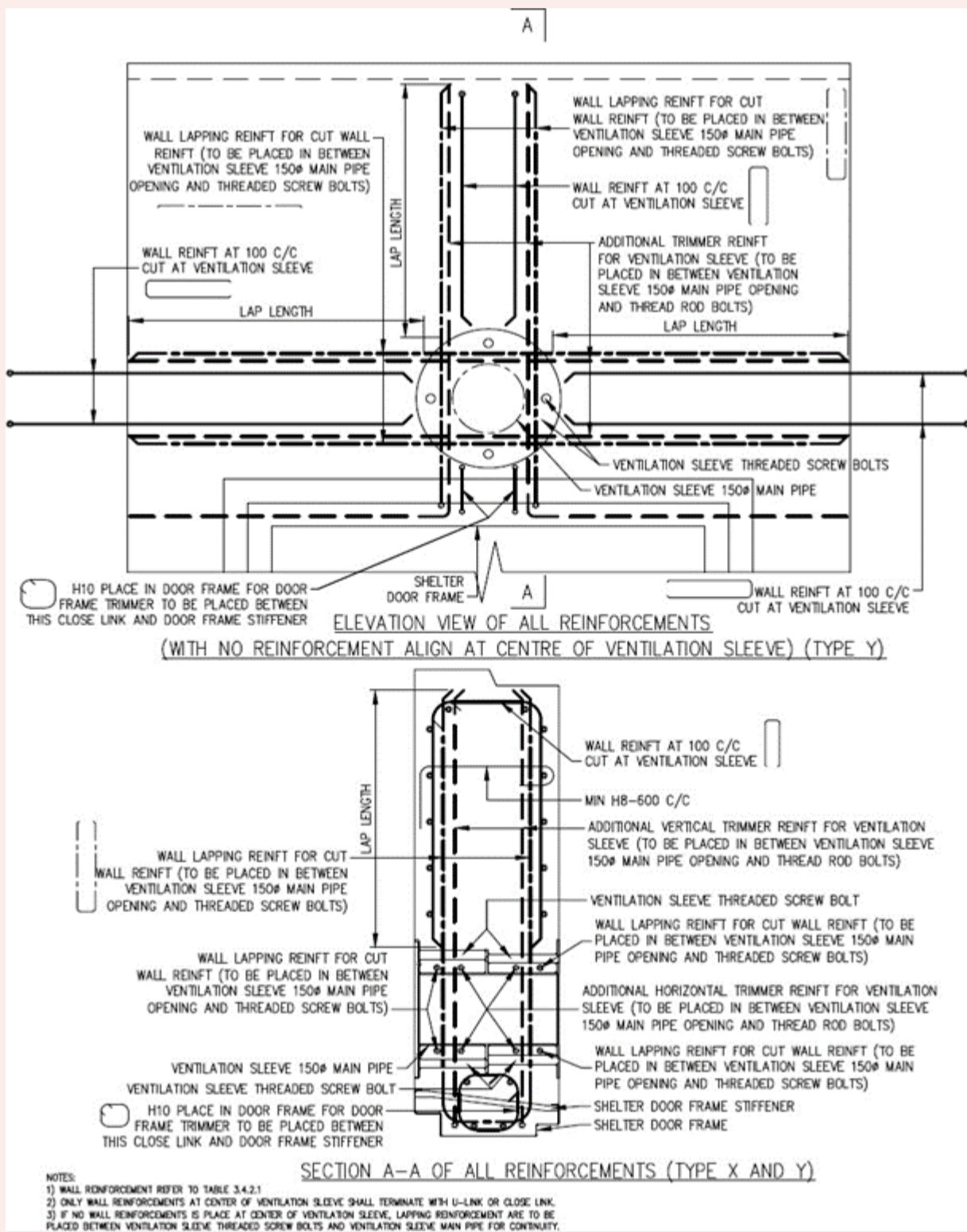
FIGURE 3.5.5(o)(ii): TYPICAL DETAILS AND SECTIONS OF REINFORCEMENTS AT VENTILATION SLEEVE LOCATION
