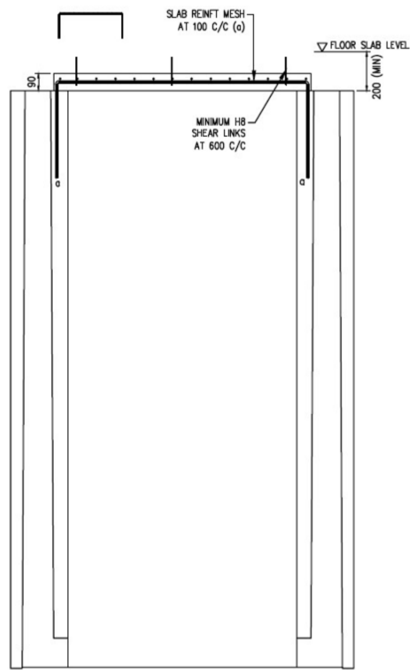
FIGURE 3.5.6.2(c)(viii): SECTION W-W (S/C SS COMPONENT 'C')
