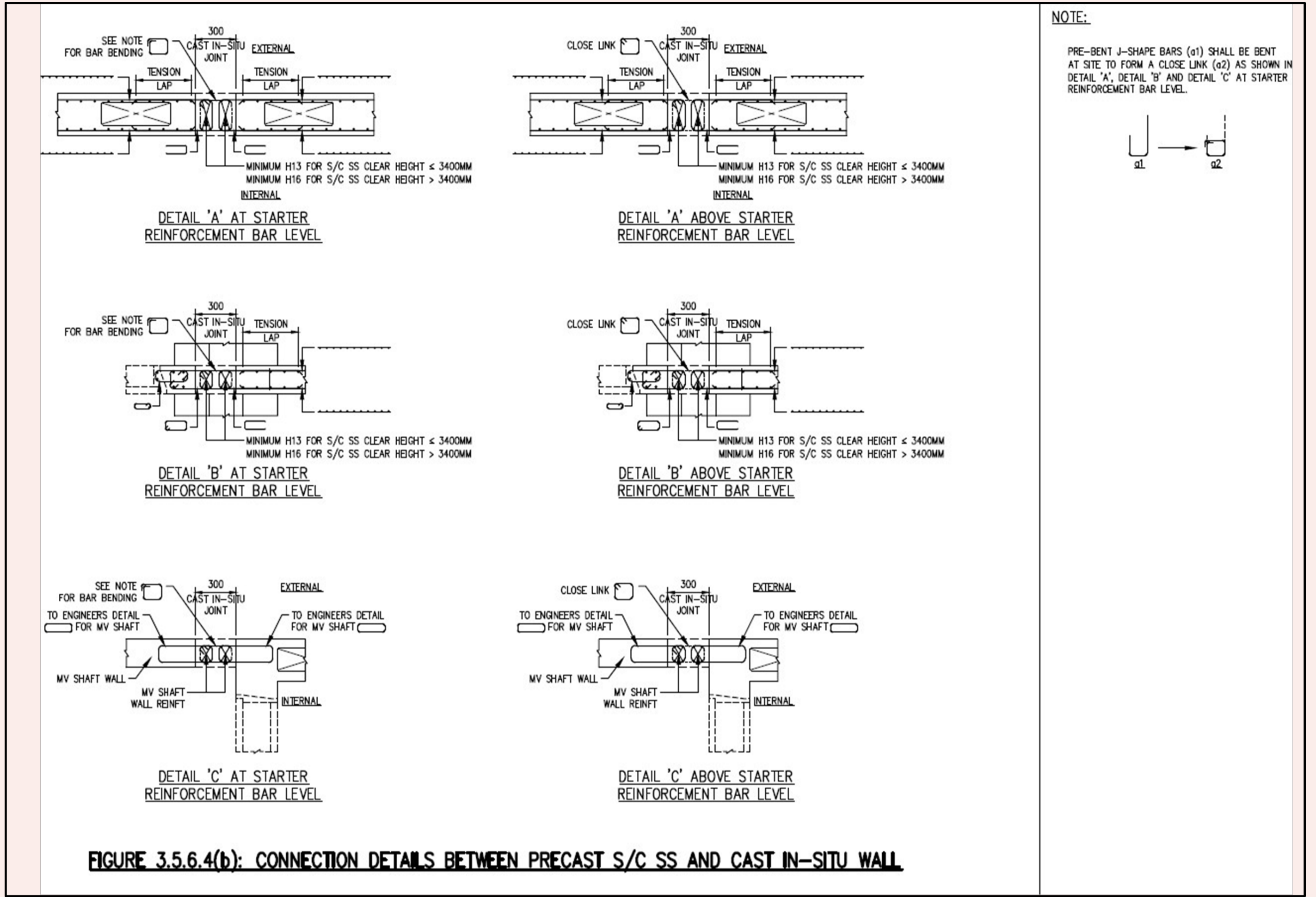
FIGURE 3.5.6.4(b)
