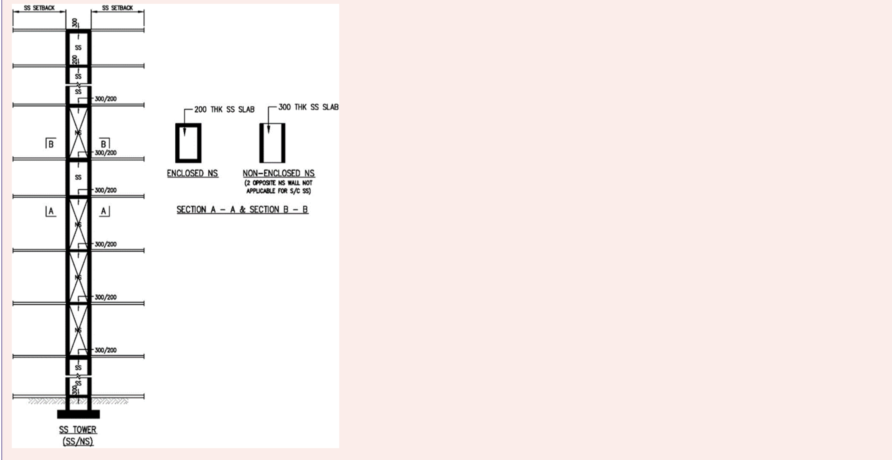
FIGURE 2.3.2: SS TOWER SHOWING SS AND NS (WITH ENCLOSED AND NON-ENCLOSED NS WALL) SLAB THICKNESS
