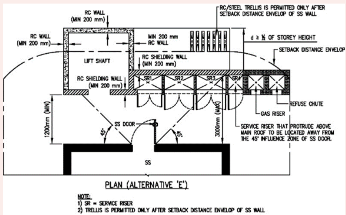
FIGURE 2.5.4(f): SHIELDING FOR SS DOOR
