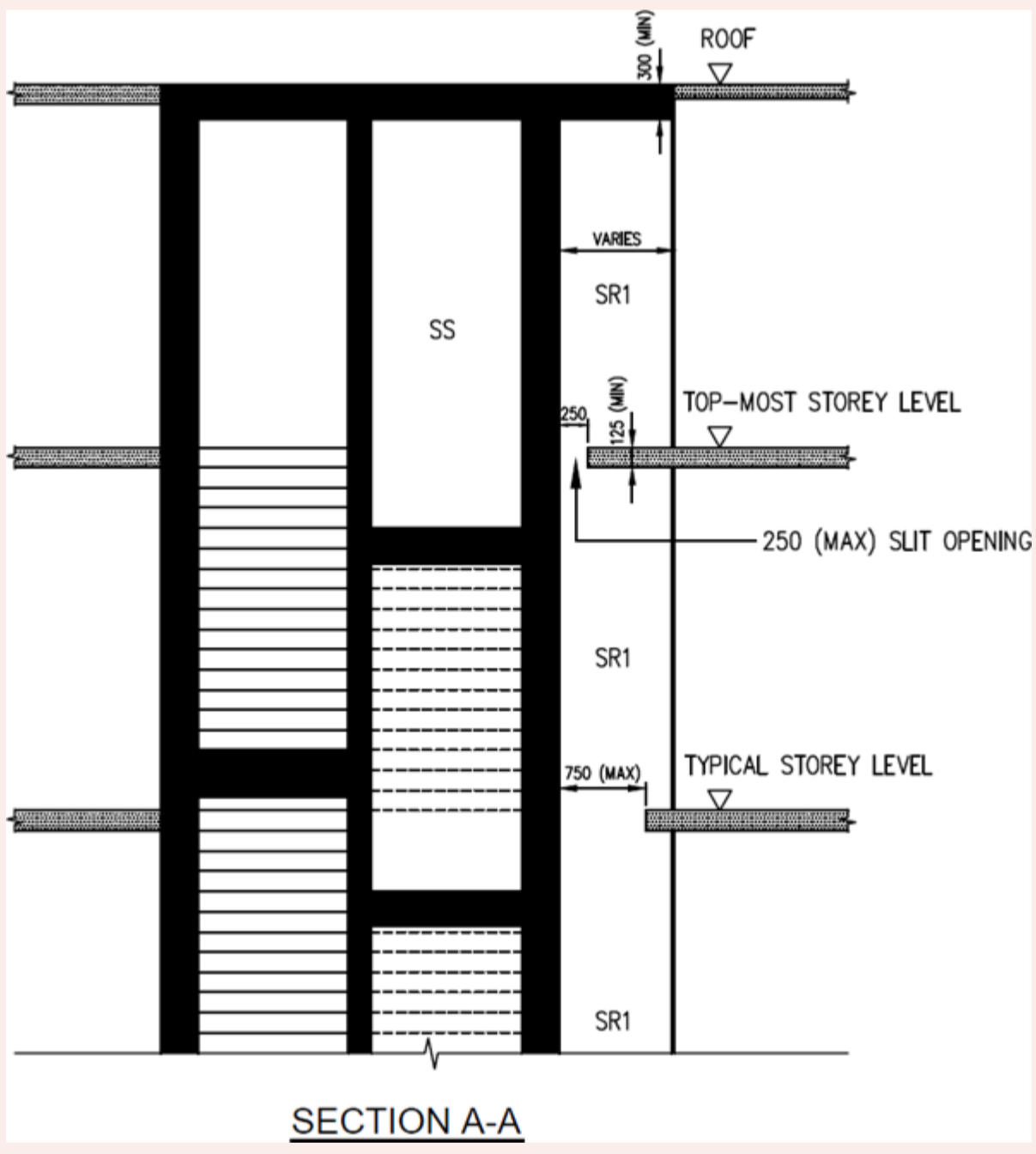
FIGURE 2.4.5(d): SERVICE RISERS ABUTTING S/C SS WALLS
