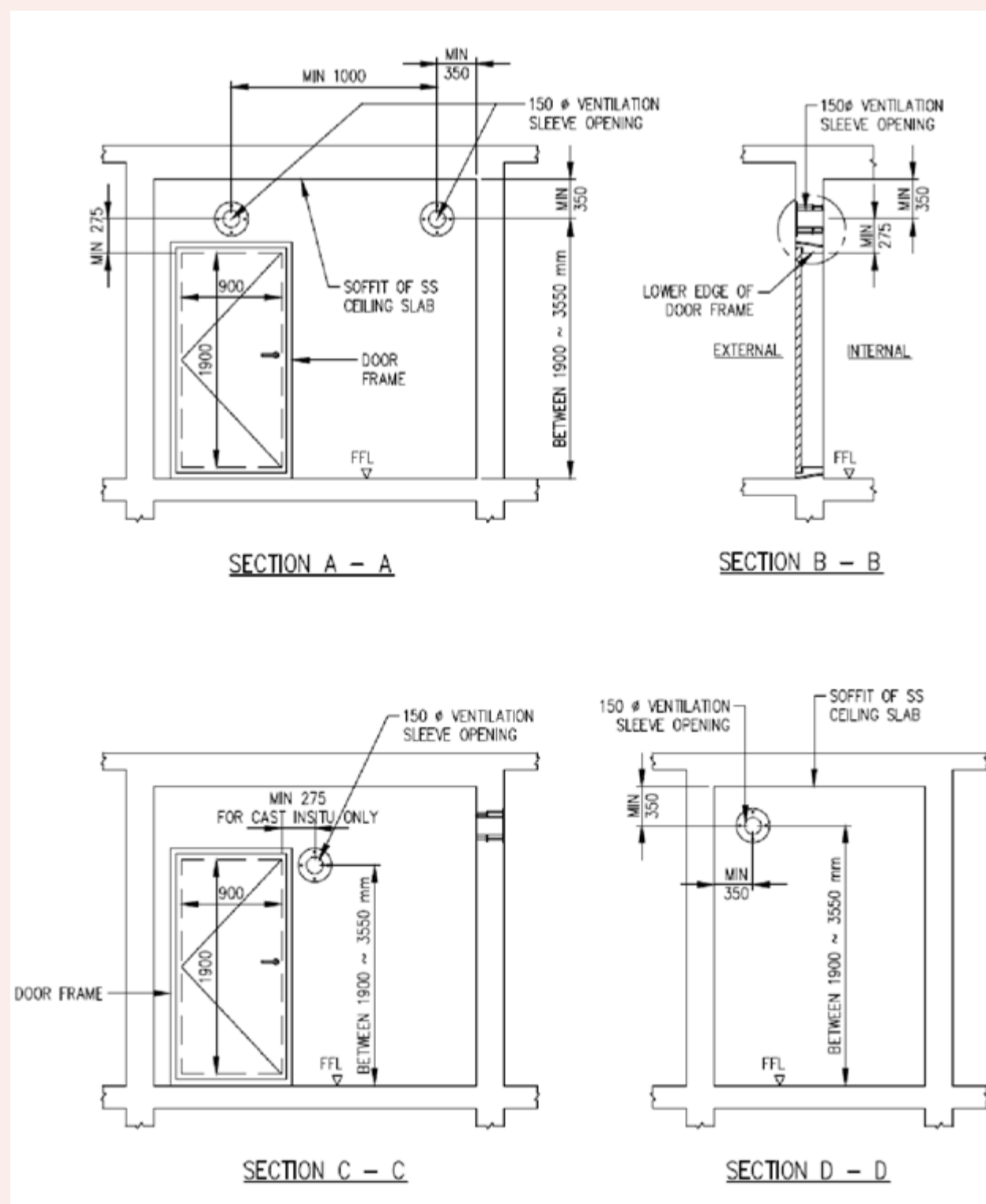
FIGURE 4.2(b): SECTIONAL VIEWS OF VENTILATION SLEEVES
