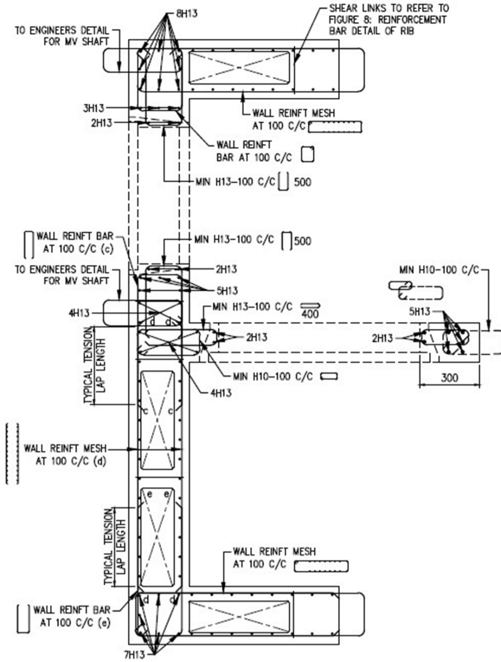
FIGURE 3.5.6.2(a)(ii): PLAN OF PRECAST S/C SS WALL WITH REINFORCEMENT DETAILS AT BLAST HATCH OPENING (S/C SS COMPONENT 'A')
