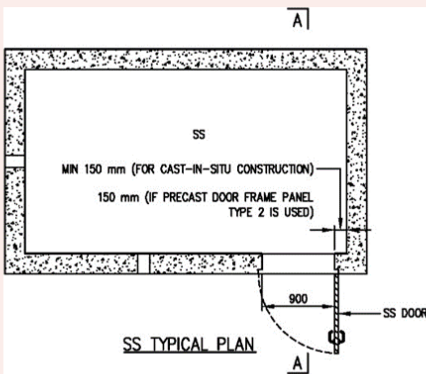
FIGURE 2.5.3(a): CONCRETE WALL SEGMENT AT SS DOOR
