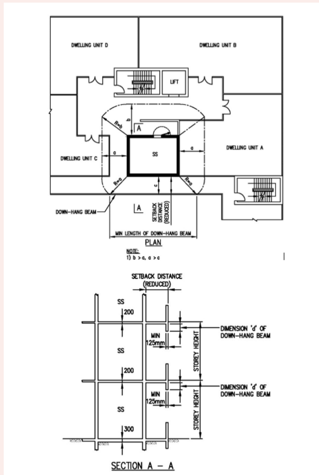
FIGURE 2.4.4(a): REQUIREMENT ON SETBACK DISTANCE OF SS WALLS (WITH DOWN-HANG BEAM) (EFFECTIVE STOREY HEIGHT = STOREY HEIGHT - DIMENSION 'd' OF DOWN-HANG BEAM)
