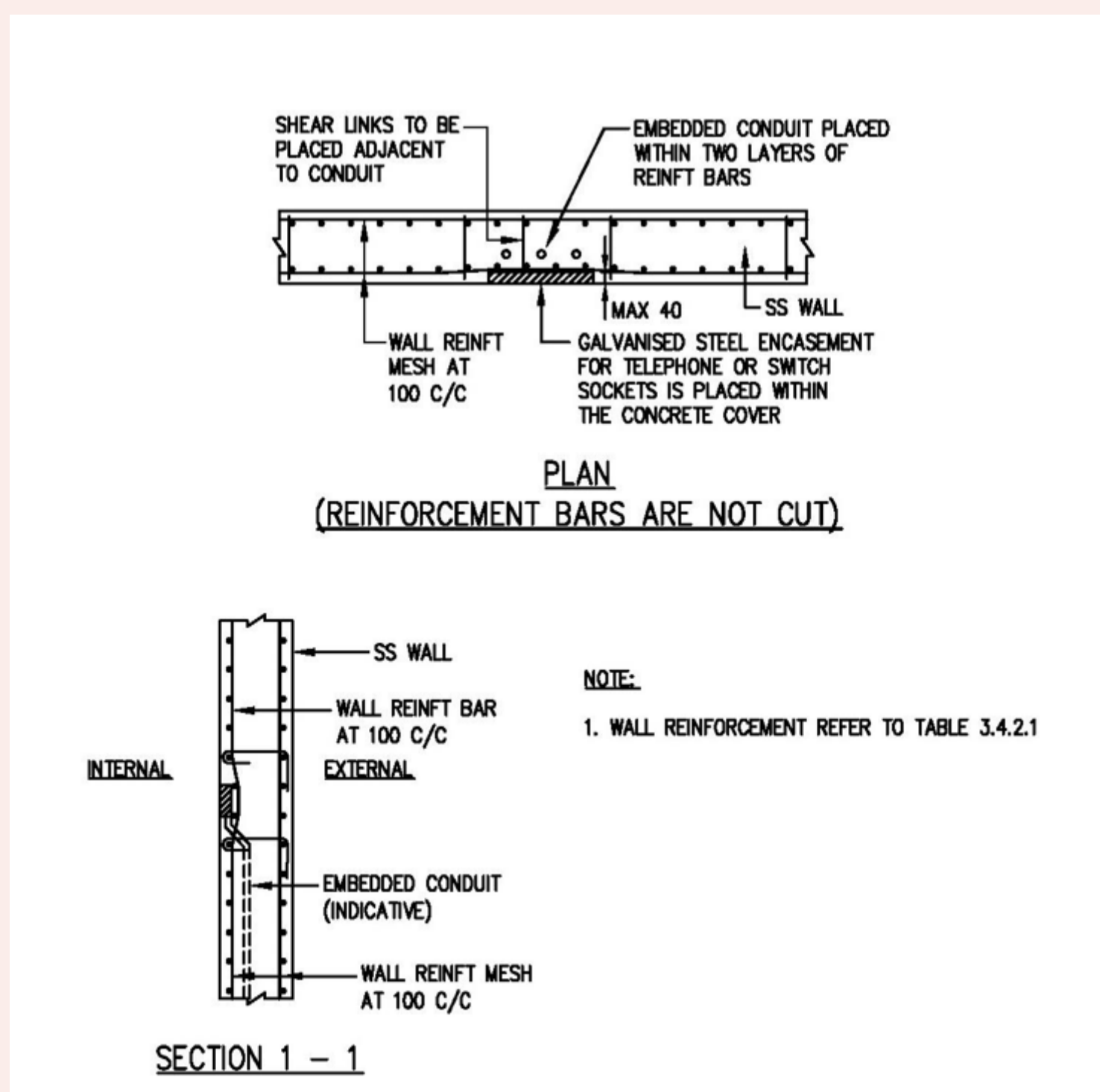
FIGURE 3.5.4(e): TYPICAL DETAILS OF EMBEDDED CONDUIT IN SS WALL
