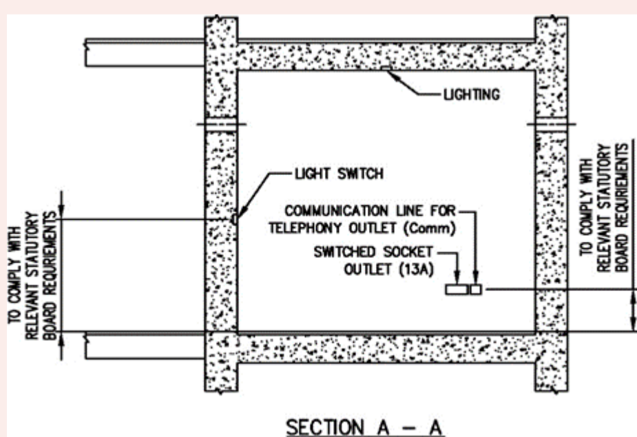
FIGURE 2.6.1(b): FIXTURE IN SS
