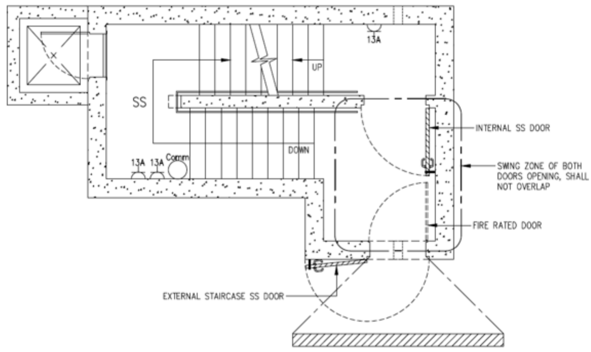
PLAN OF STAIRCASE SS COMPARTMENT AT TYPICAL FLOOR
