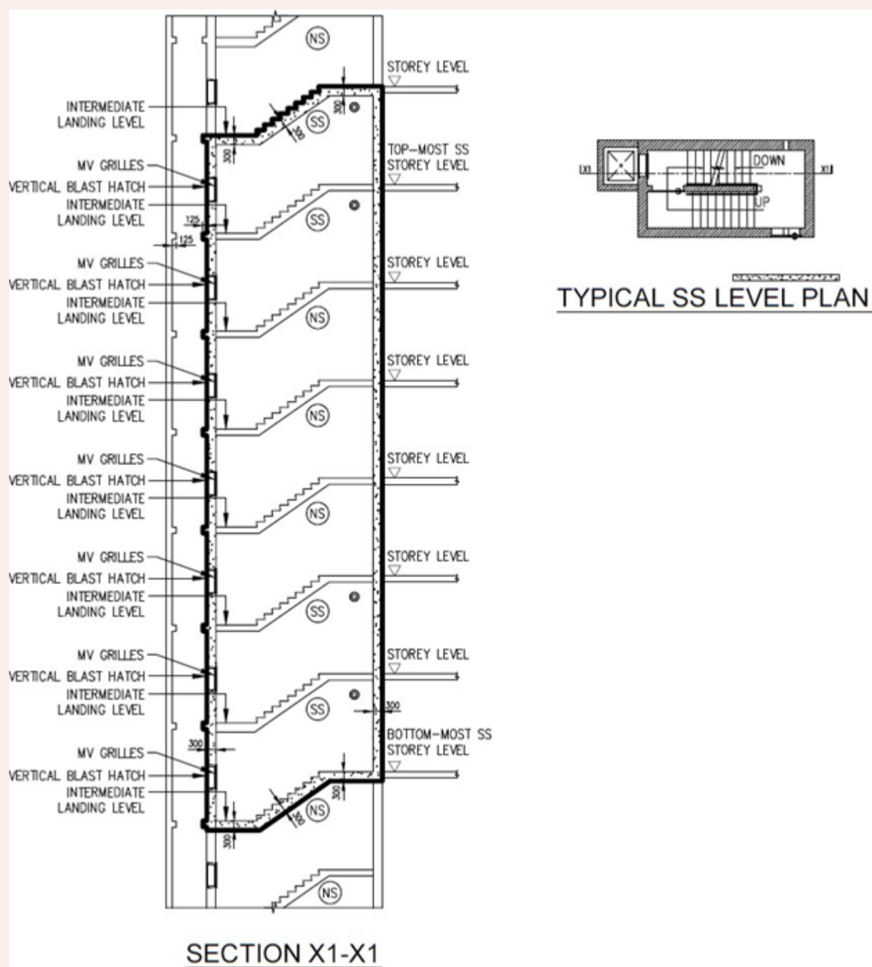
FIGURE 2.12.1(b): PROTECTION CARCASS OF S/C SS TOWER
