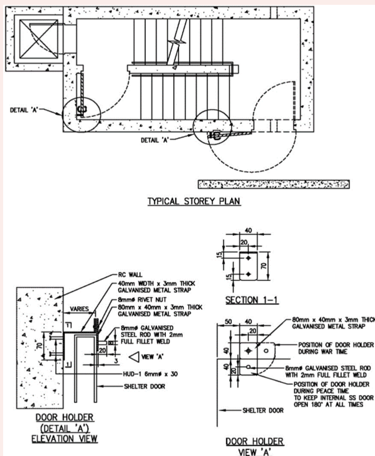
FIGURE 2.12.2(i): DETAIL OF SS DOOR HOLDER
