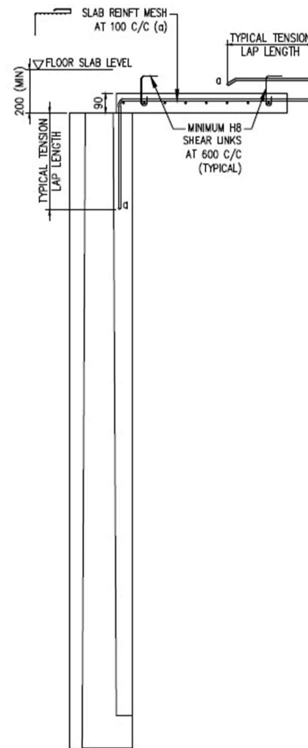
FIGURE 3.5.6.2(a)(iv): SECTION D-D (S/C SS COMPONENT 'A')
