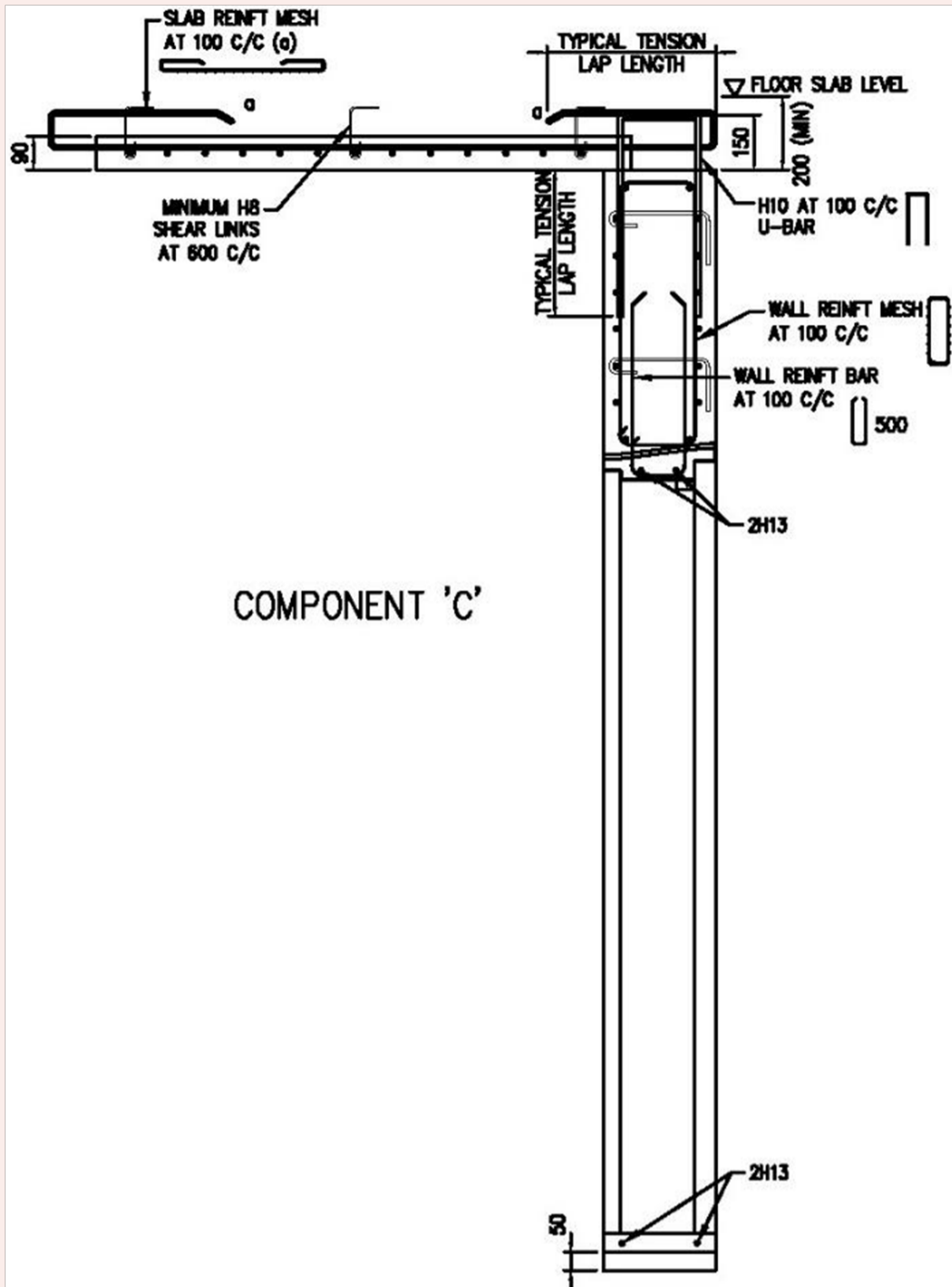
FIGURE 3.5.6.2(c)(iii): SECTION S-S (S/C SS COMPONENT 'C')
