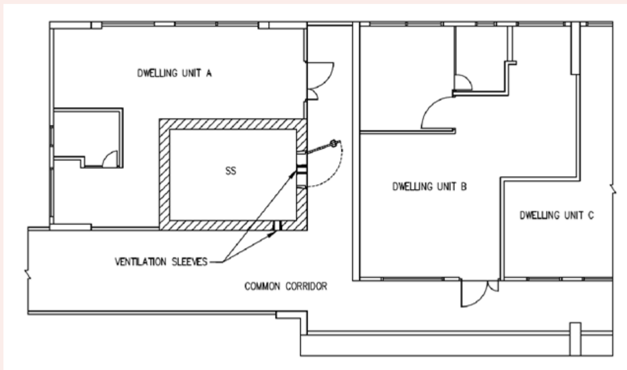
FIGURE 4.2(c): LOCATION OF VENTILATION SLEEVES
