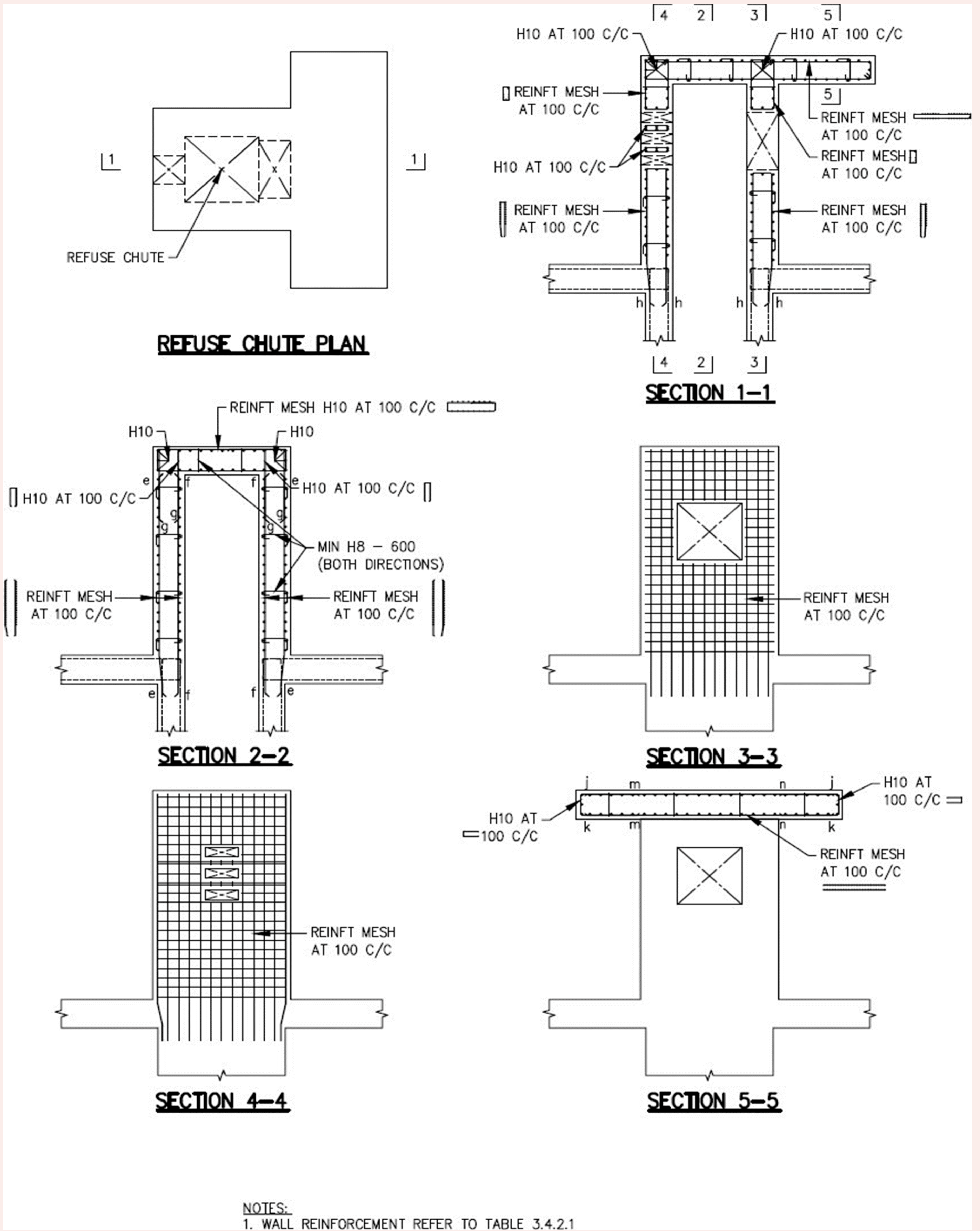
FIGURE 3.6.3(a): REINFORCEMENT DETAILS OF REFUSE CHUTE ABOVE ROOF LEVEL WITHIN SS SETBACK DISTANCE
