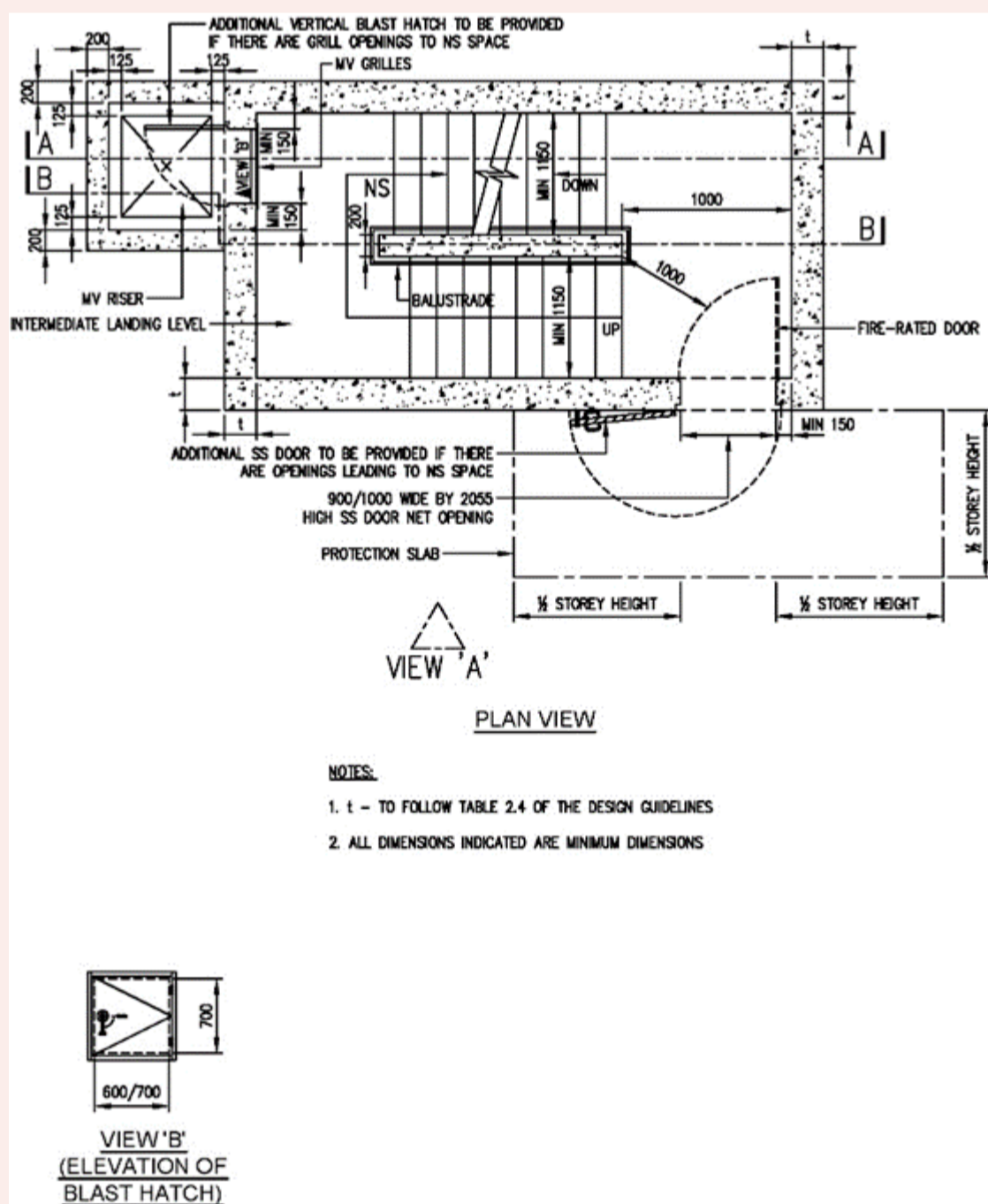
FIGURE 2.12.1(d): PLAN OF NON-SHELTER (NS) ABOVE TOP-MOST S/C SS COMPARTMENT
