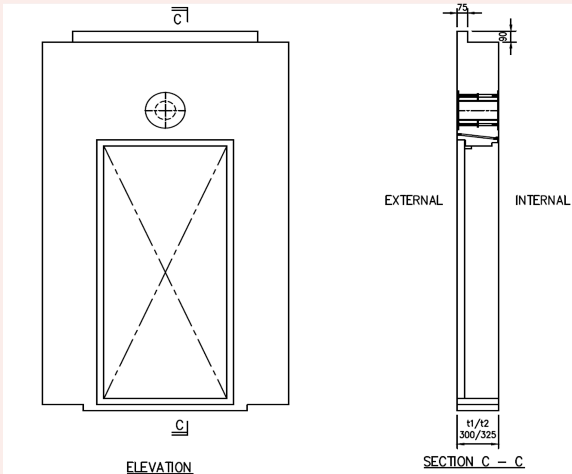
FIGURE 3.5.6.1(c): BLAST DOOR AND VENTILATION SLEEVE
