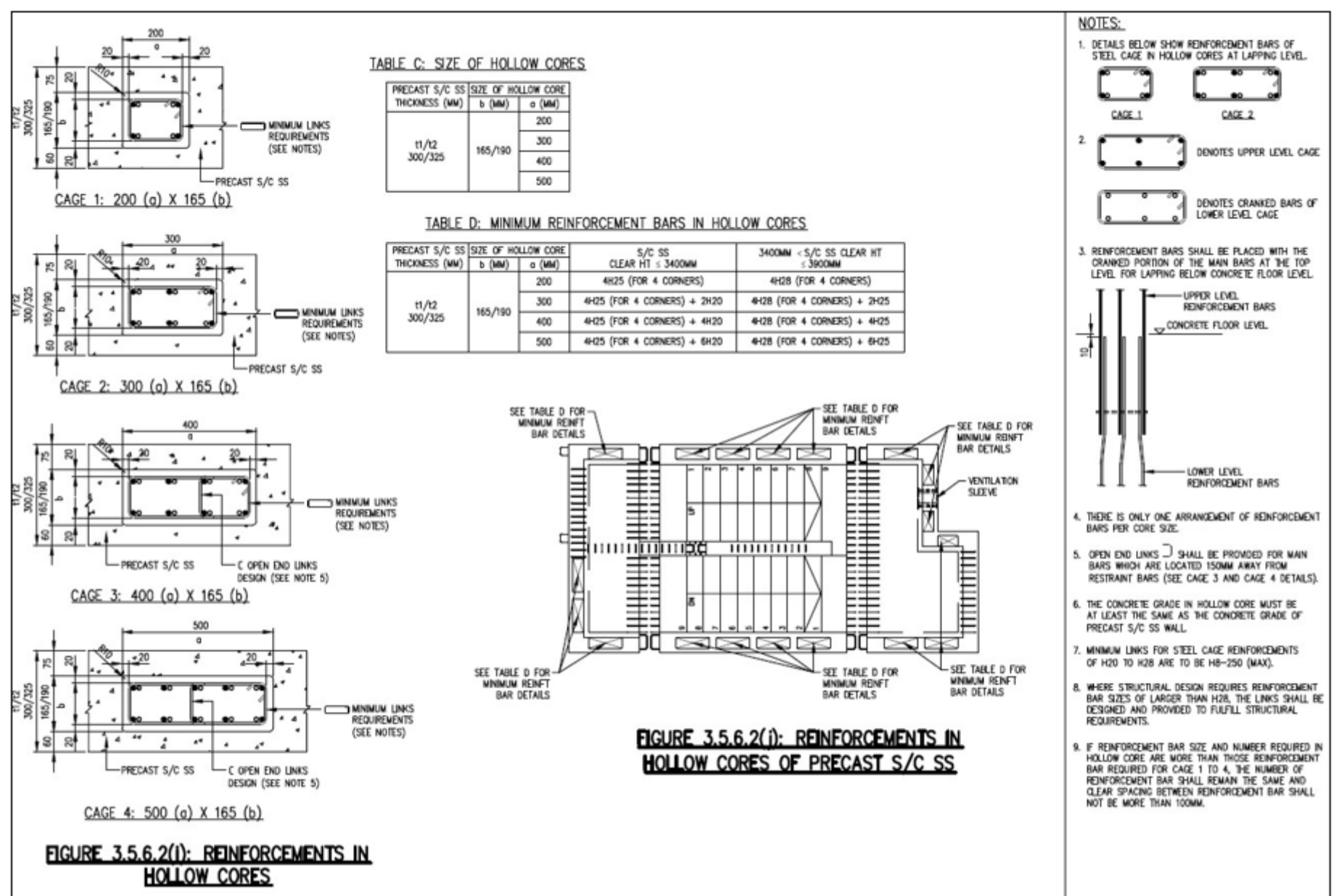
FIGURE 3.5.6.2(i) & FIGURE 3.5.6.2 (j)
