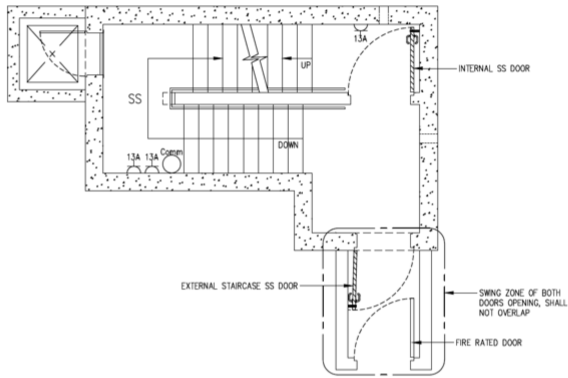
PLAN OF STAIRCASE SS COMPARTMENT AT TYPICAL FLOOR
