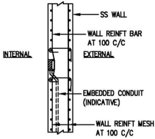
SECTION 1 - 1
