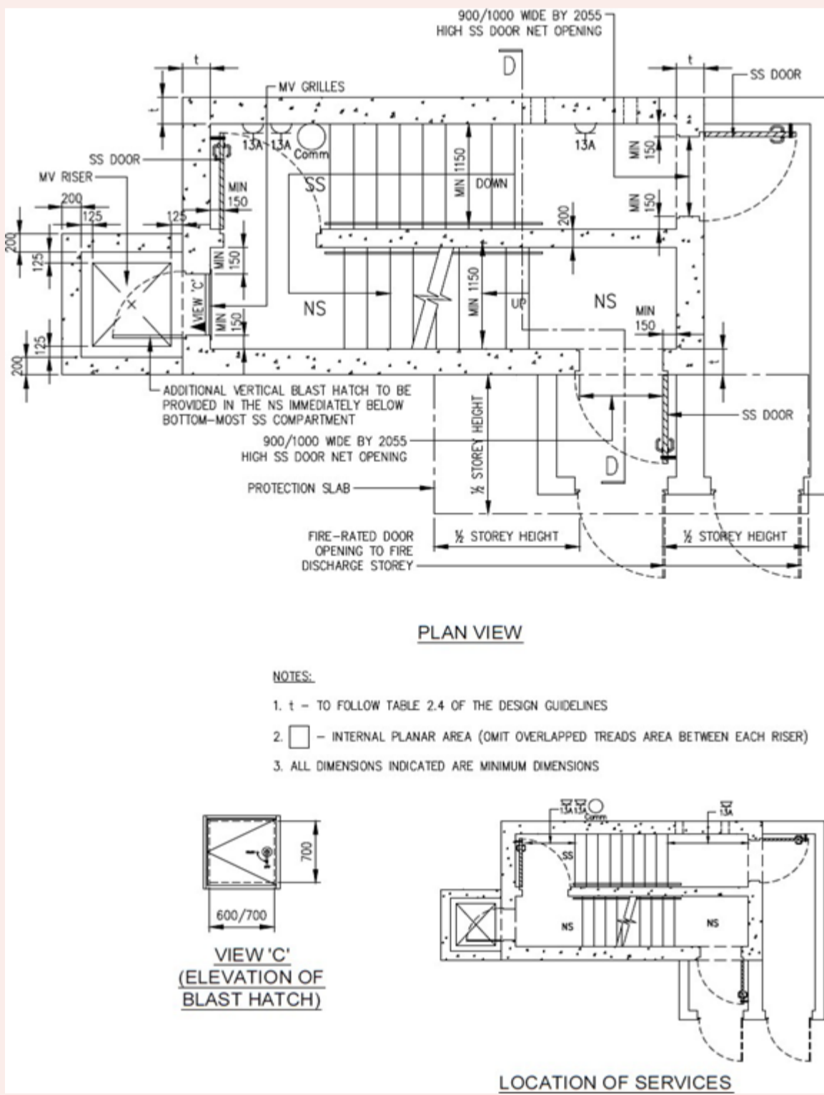
FIGURE 2.12.2(f): DETAIL PLAN OF S/C SS AND NS AT FIRE DISCHARGE STOREY
