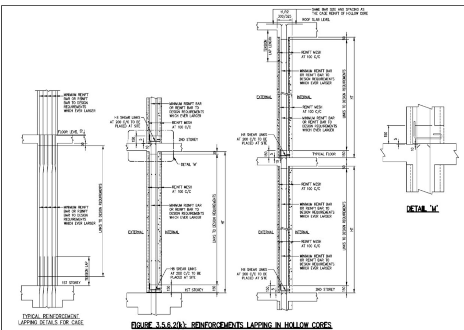
FIGURE 3.5.6.2(k)
