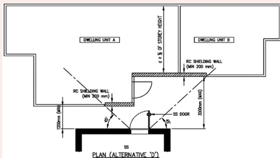
FIGURE 2.5.4(d): SHIELDING FOR SS DOOR
