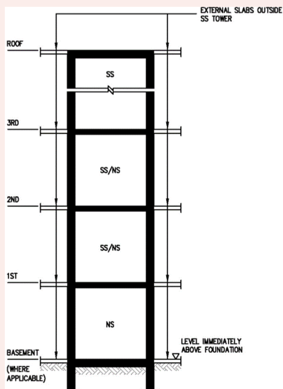
FIGURE 2.4.2: SCHEMATIC SECTION OF SS TOWER
