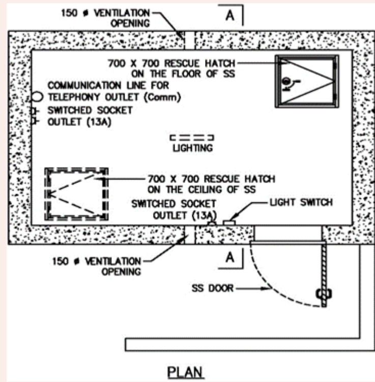
FIGURE 2.6.1(a): SPECIFIC SS FIXTURE AND OPENINGS
