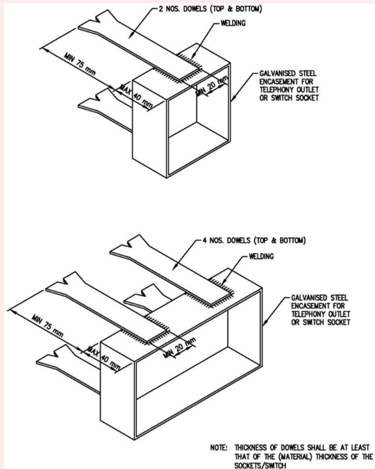
FIGURE 3.6.1(b): TYPICAL DETAILS OF EMBEDDED SOCKET/SWITCH
