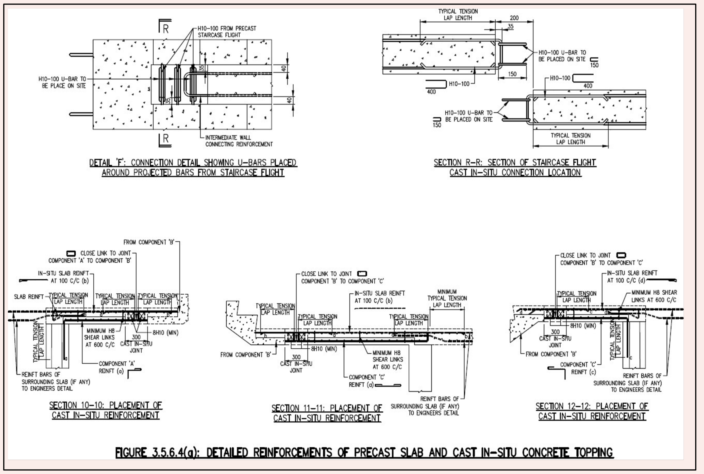
FIGURE 3.5.6.4(a)
