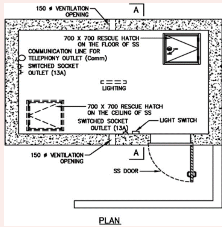
FIGURE 2.6.1(a): SPECIFIC SS FIXTURE AND OPENINGS
