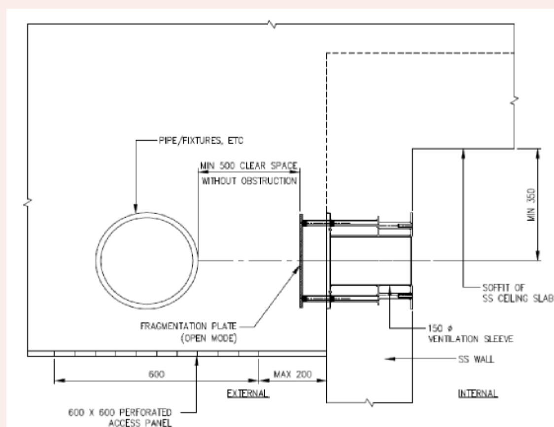
FIGURE 4.3.2: PERFORATED ACCESS PANEL BELOW VENTILATION SLEEVE
