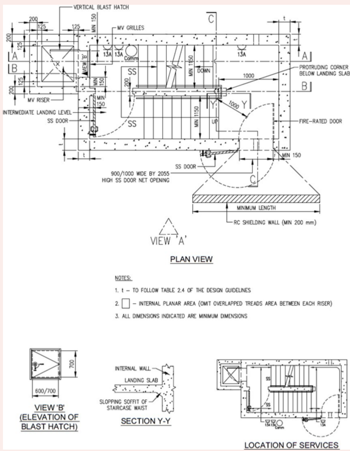
FIGURE 2.12.2(d): SS WITH NS ABOVE TOP-MOST SS COMPARTMENT, INTERMEDIATE SS COMPARTMENT AND SS WITH NS BELOW BOTTOM-MOST SS COMPARTMENT
