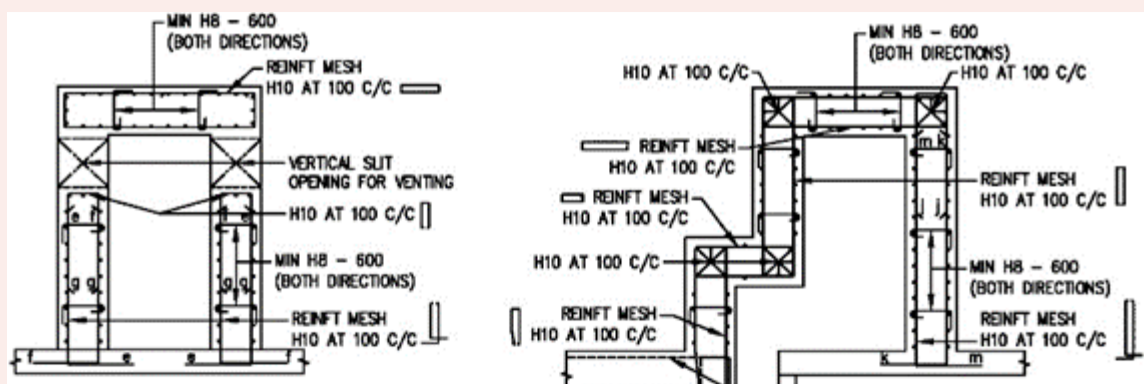
REINFORCEMENT DETAIL OF SECTION 2A-2A OF RC PROTECTION REQUIREMENT AT ROOF LEVEL FOR PROVISION OF GAS AND WATER RISER LOCATED WITHIN SETBACK DISTANCE ENVELOP (TYPE A)
