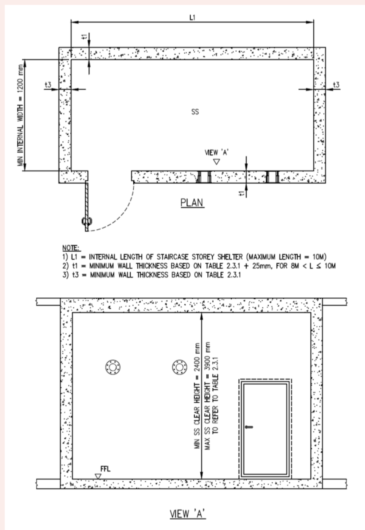
FIGURE 2.2.1(a): TYPICAL LAYOUT OF SS
