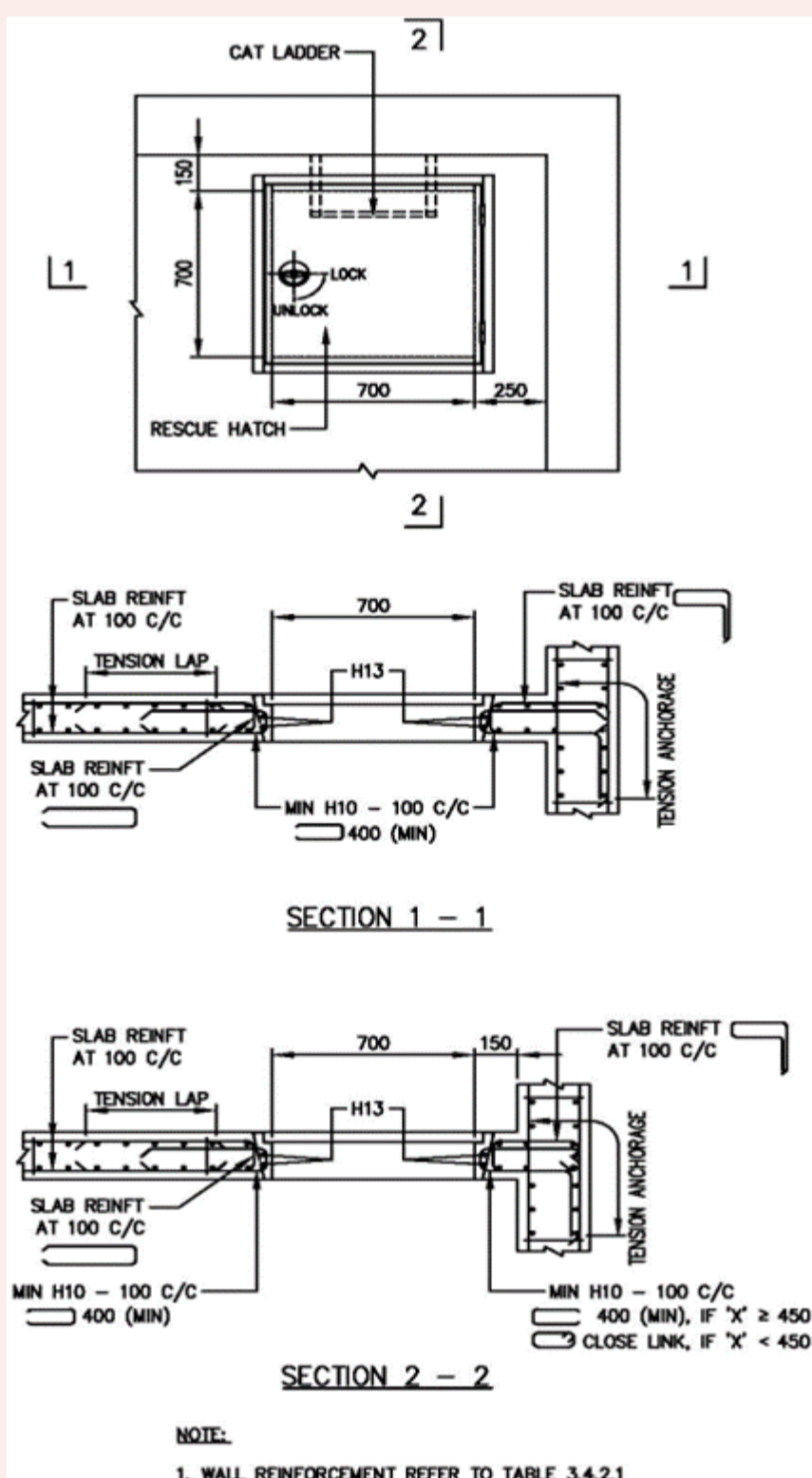
FIGURE 3.5.4(i): DETAILS OF SS SLAB REINFORCEMENT NEAR RESCUE HATCH
