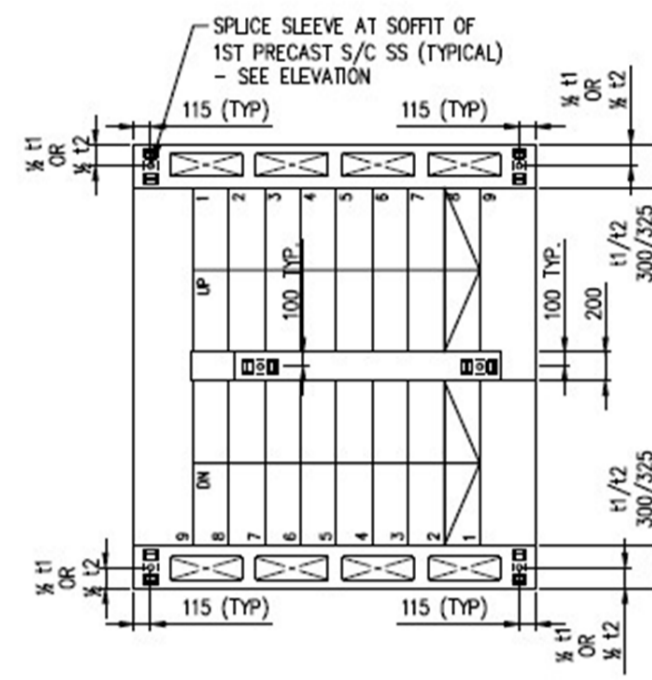
REFERENCE PLAN FOR 1ST STOREY COMPONENT 'B' PRECAST S/C SS (SIZE AND ARRANGEMENT OF CORES SHOWN IS INDICATIVE ONLY)
