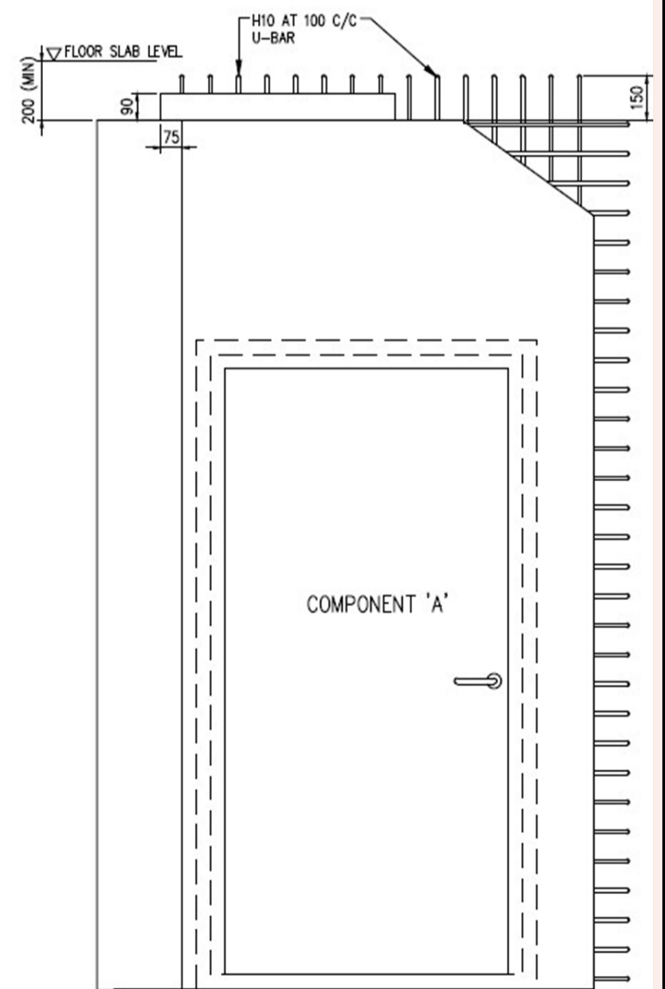
FIGURE 3.5.6.2(a)(v): SECTION E-E (S/C SS COMPONENT 'A')
