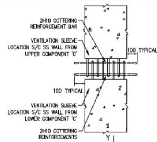
DETAIL 'J': CONNECTION DETAIL SHOWING COTTERING REINFORCEMENT BARS THROUGH OVERLAPPING PROJECTED U-LOOP BARS OF UPPER AND LOWER S/C SS WALL WITH VENTILATION SLEEVE
