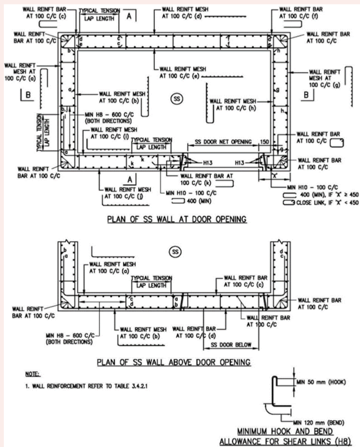
FIGURE 3.5.4(a): PLAN OF SS WALL
