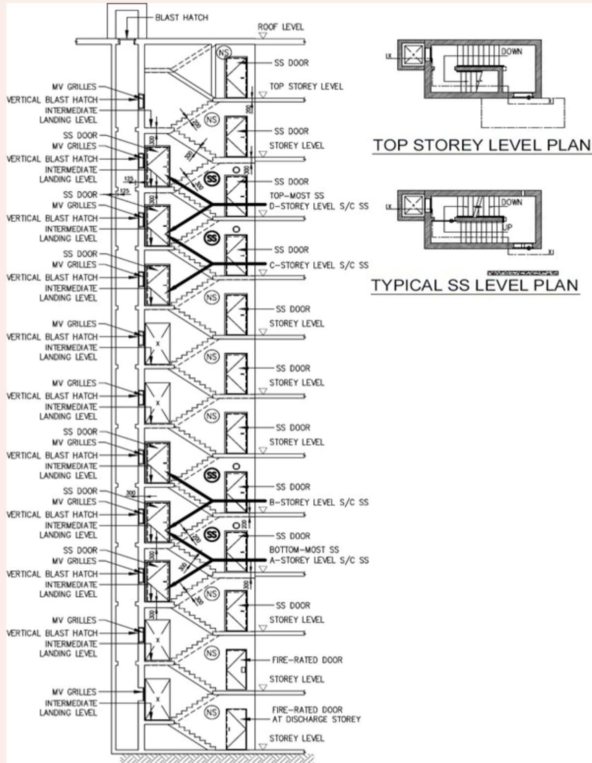
FIGURE 2.12.1(a): SECTION X-X OF S/C SS WITH SS/NS
