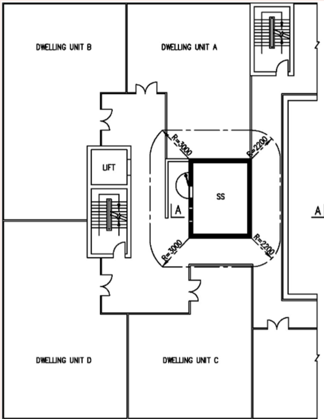
FIGURE 2.4.3(a): REQUIREMENT ON SETBACK DISTANCE OF SS WALLS (WITHOUT DOWN-HANG BEAM) (FOR 2500MM < STOREY HEIGHT | 2800MM)
