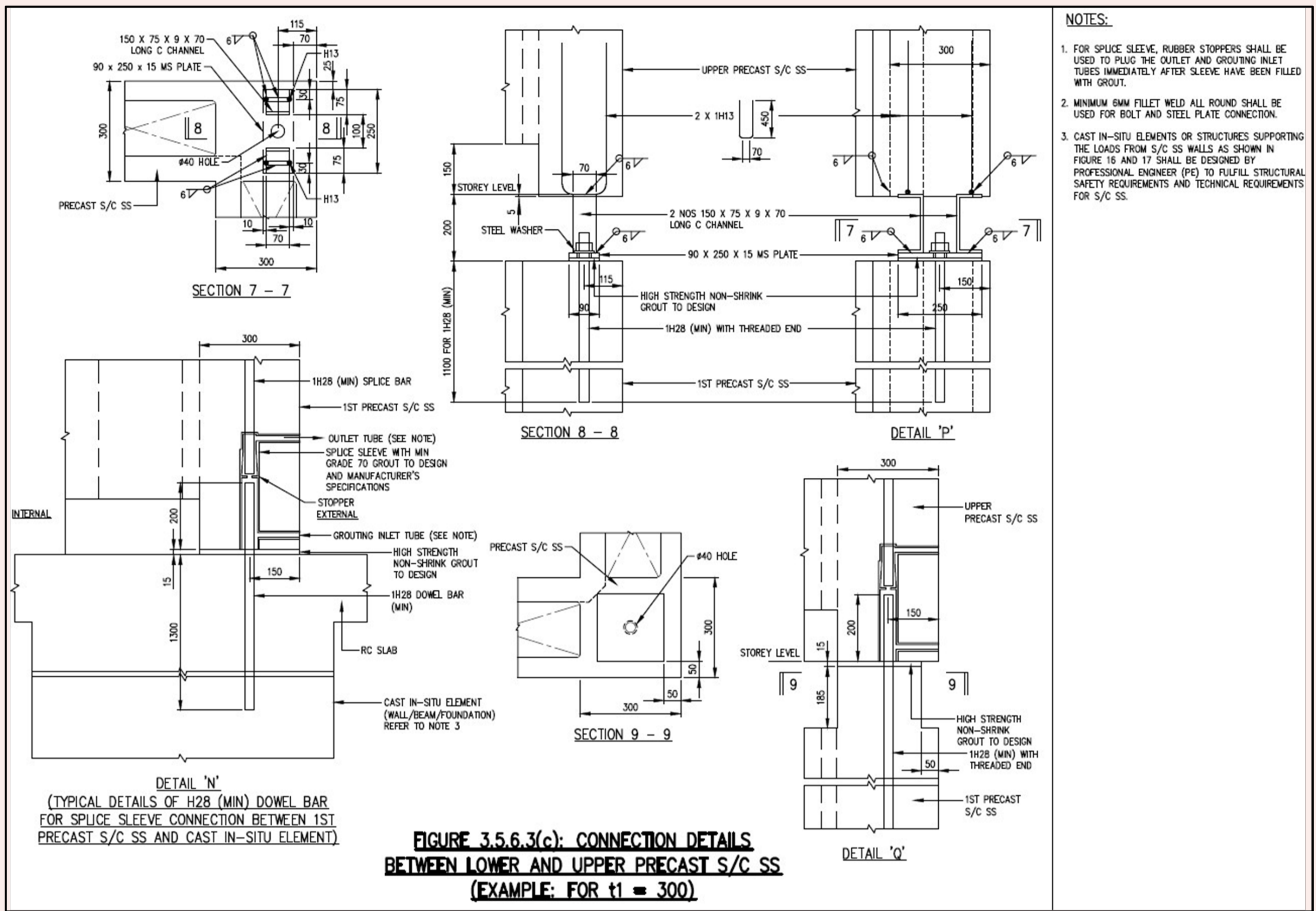
FIGURE 3.5.6.3(a) to 3.5.6.3(c)
