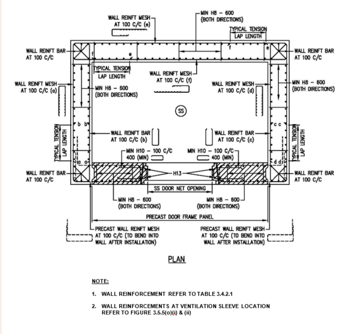
FIGURE 3.5.5(i): DETAILS OF PRECAST SS DOOR FRAME PANEL (TYPE 3)
