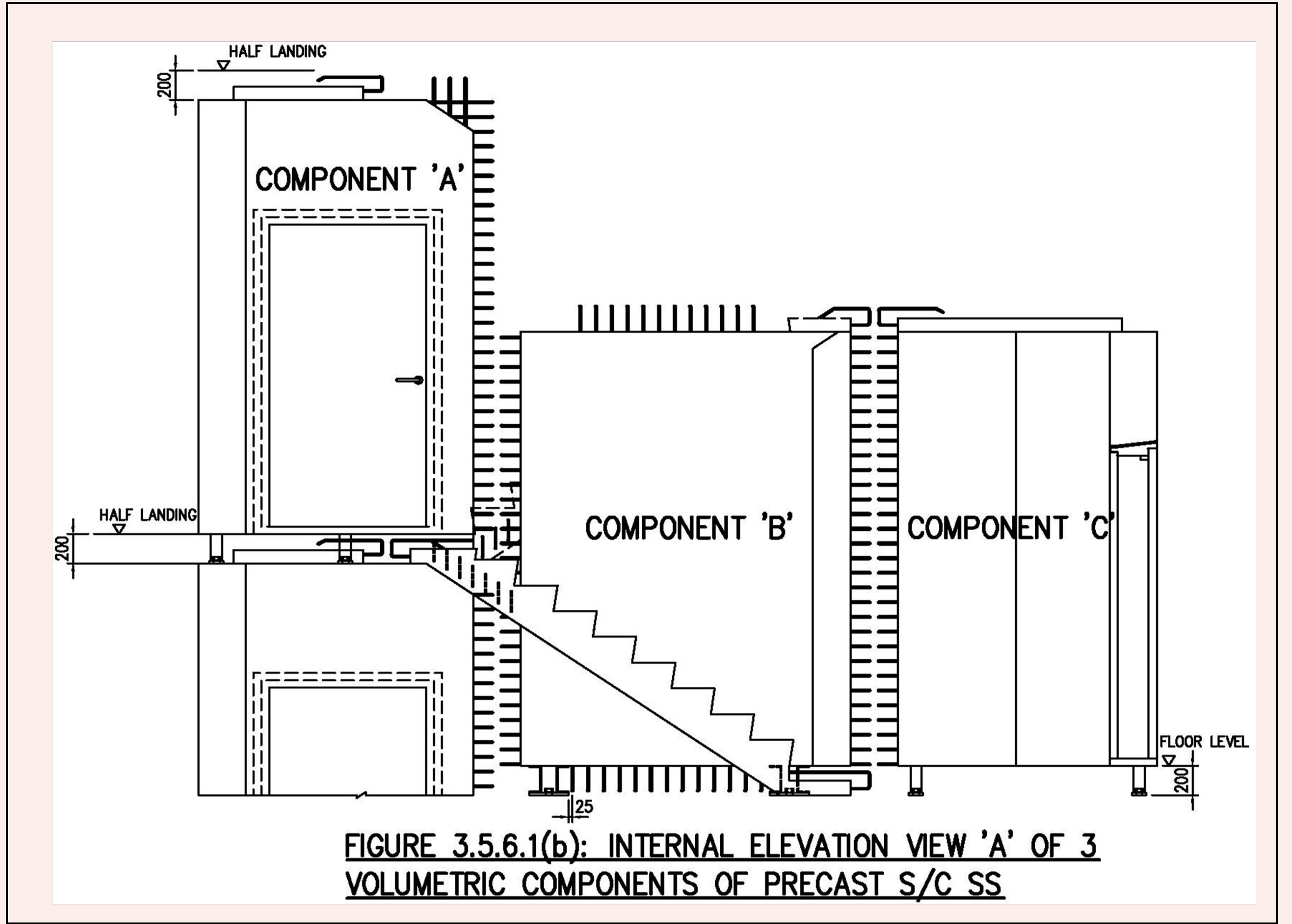
FIGURE 3.5.6.1(b)
