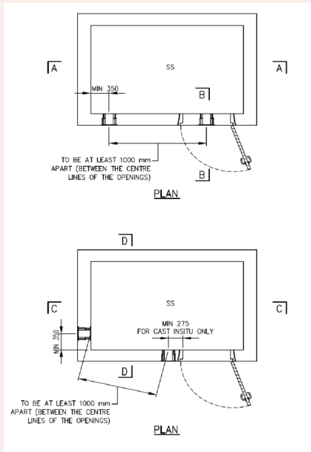
FIGURE 4.2(a): POSITION OF VENTILATION SLEEVES
