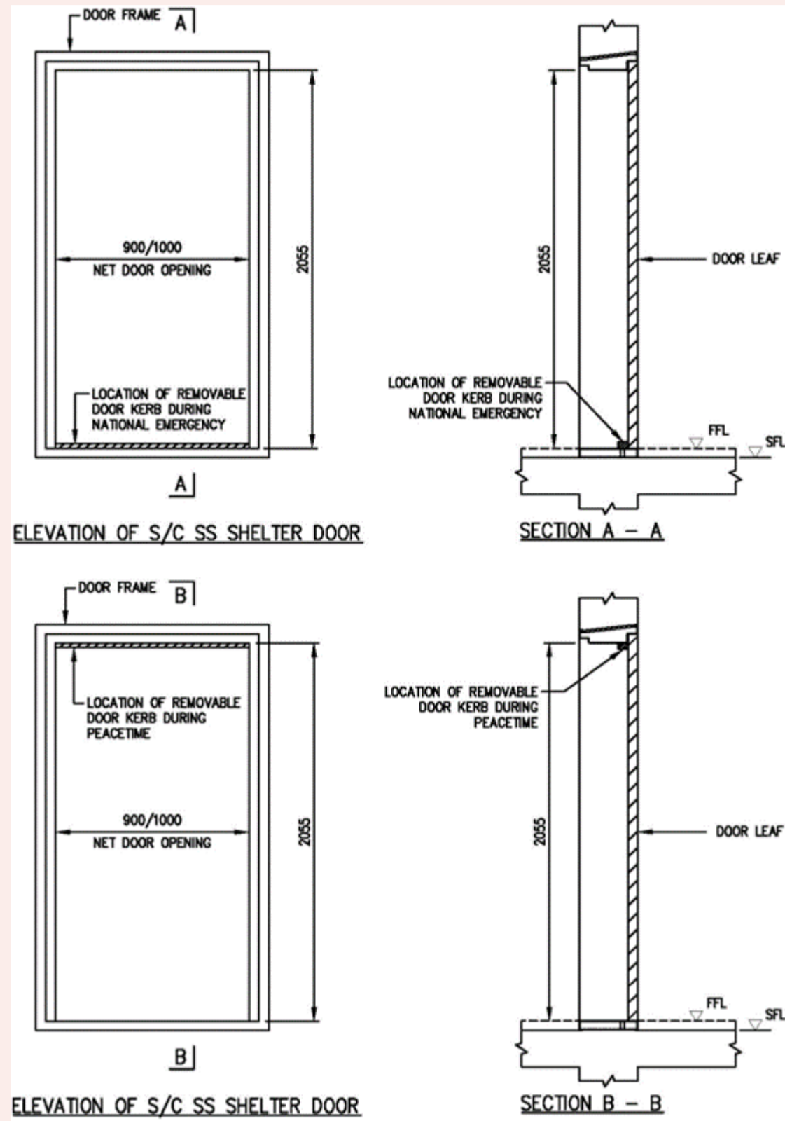
FIGURE 5.3: MOUNTING OF REMOVABLE KERB
