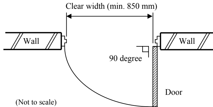
Diagram 2.2.5.13(c) - Measurement of door width
