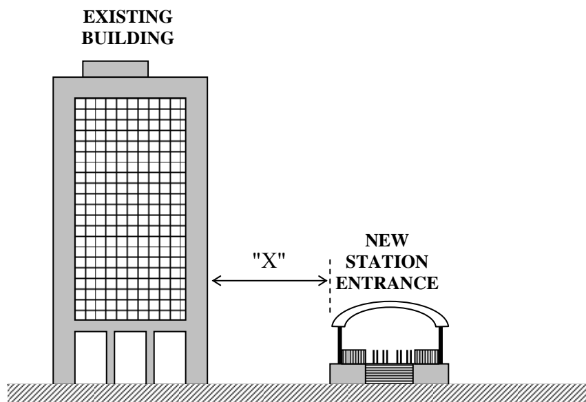
Diagram 2.3.5.2(d) - Separation distance 'X' between the external wall of a ground level entrance (with no habitable room) and the external wall of an adjacent building
